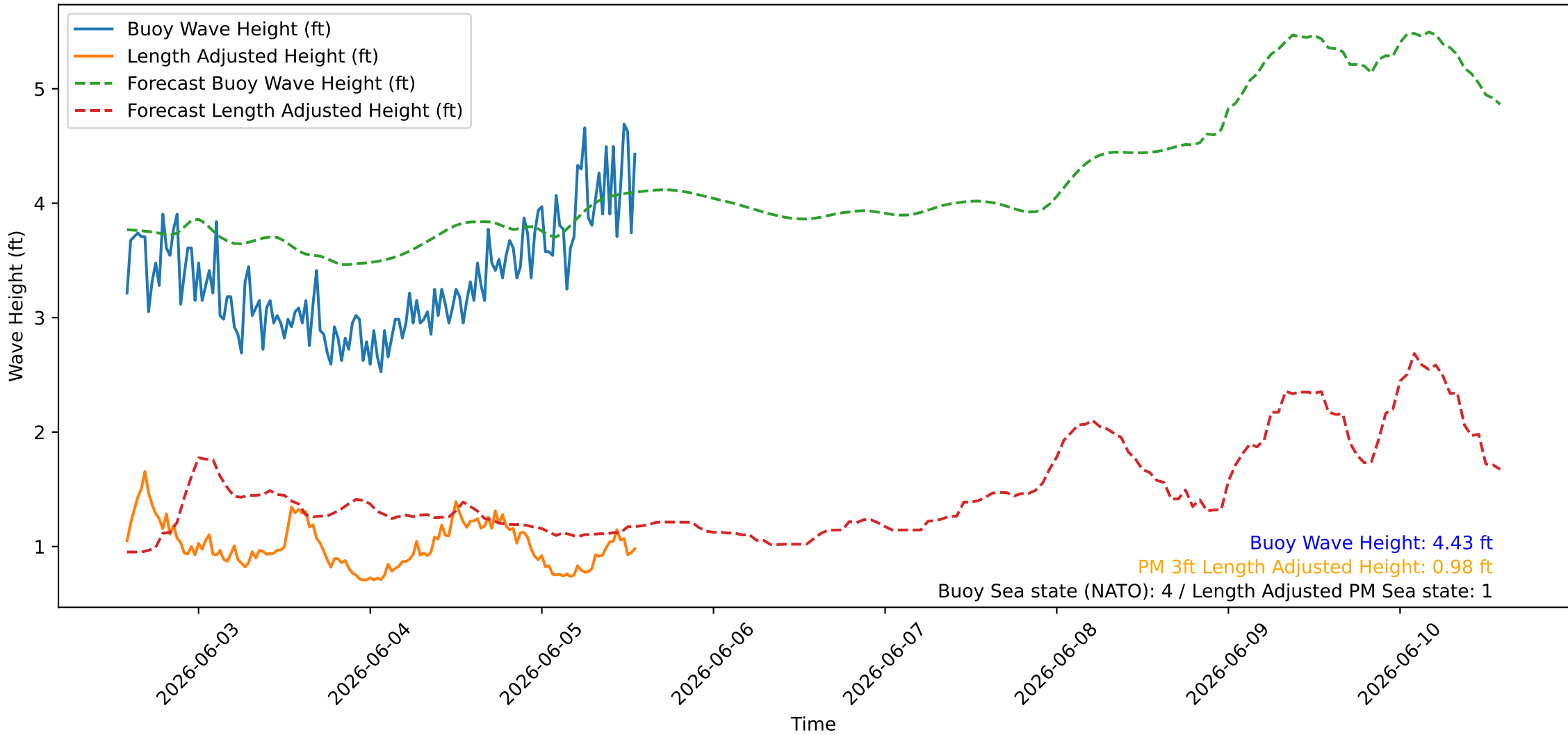
Wave Heights over Time for Red Beach at 2026-06-05 13:50:46
