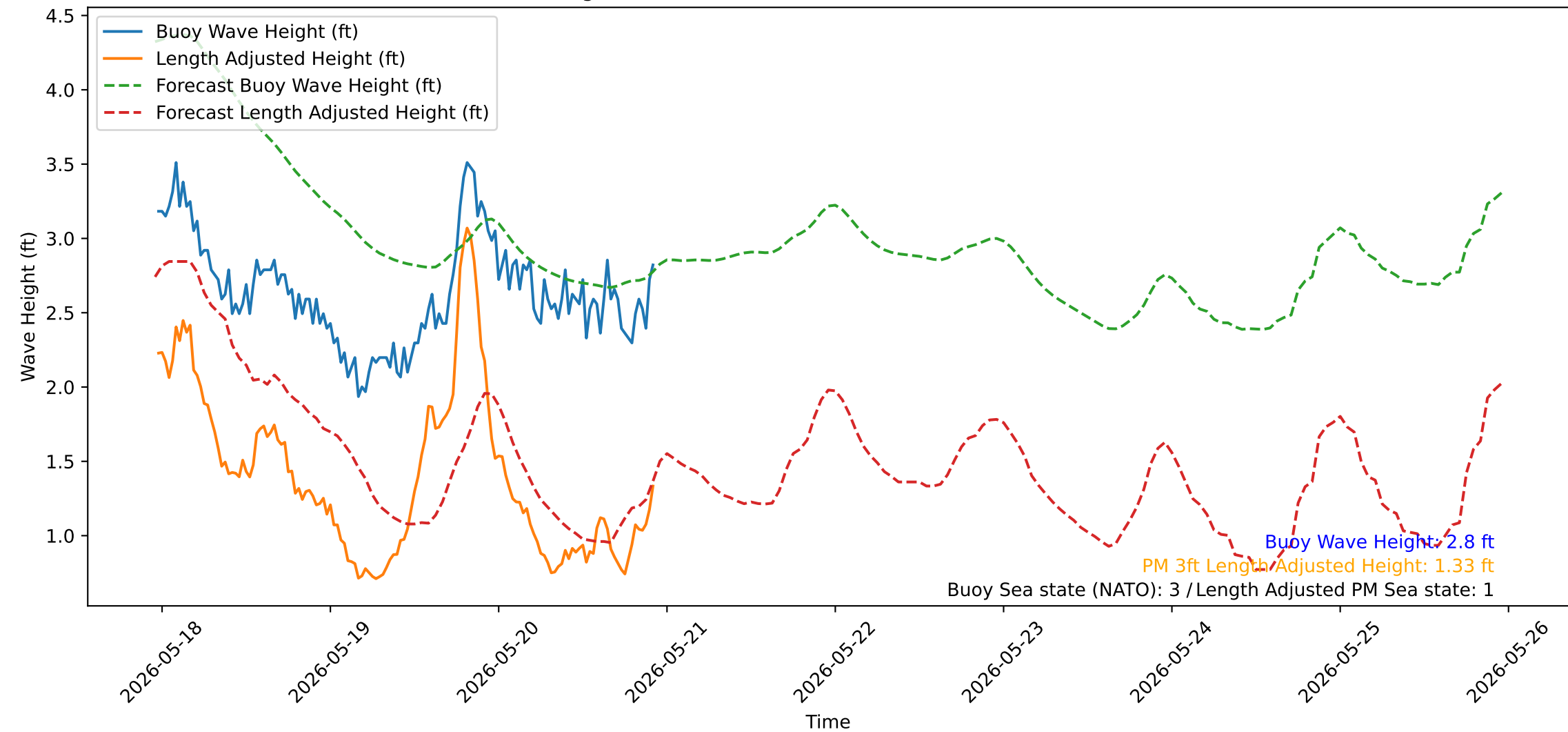
Wave Heights over Time for Red Beach at 2026-05-20 23:00:51
