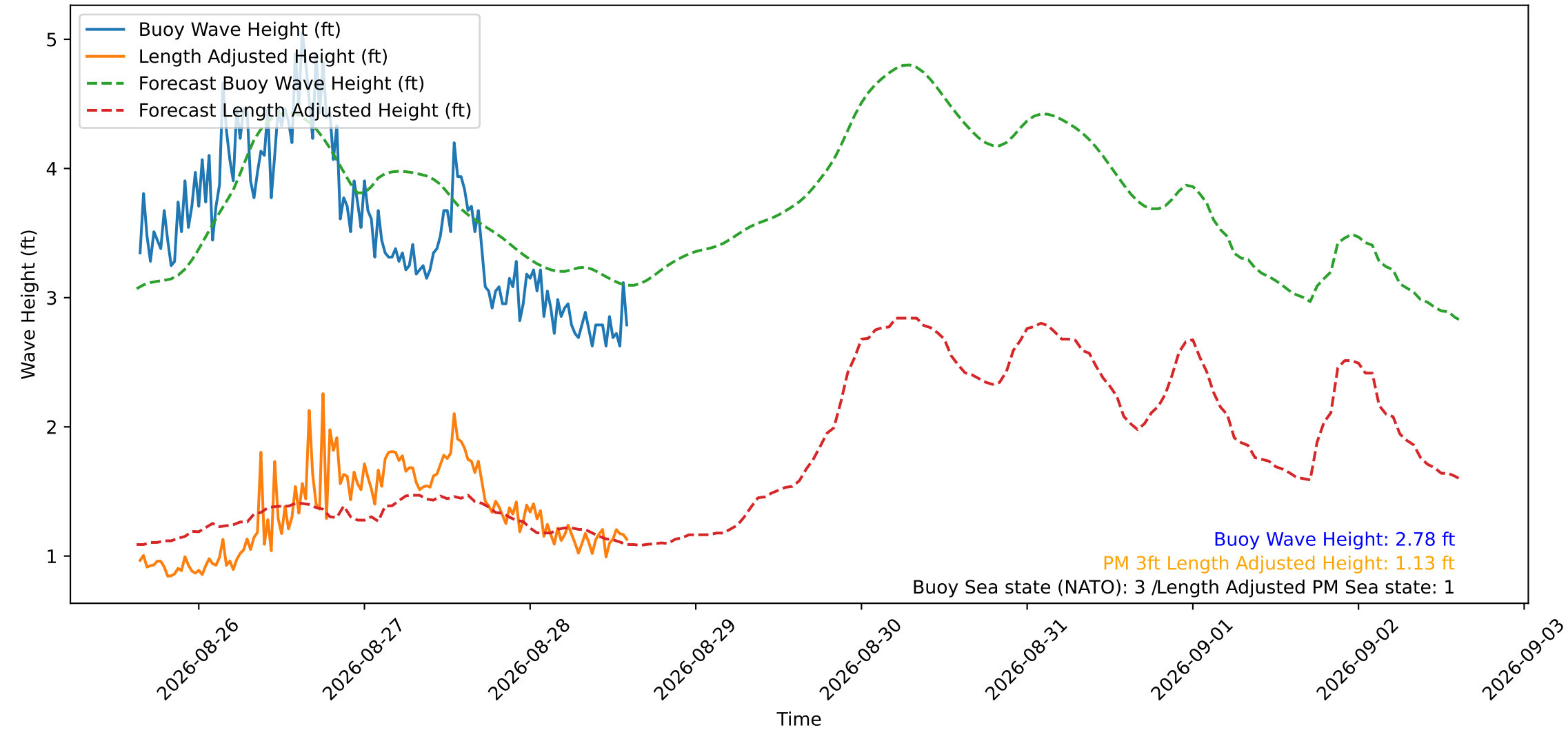
Wave Heights over Time for Red Beach at 2026-08-28 15:00:50
