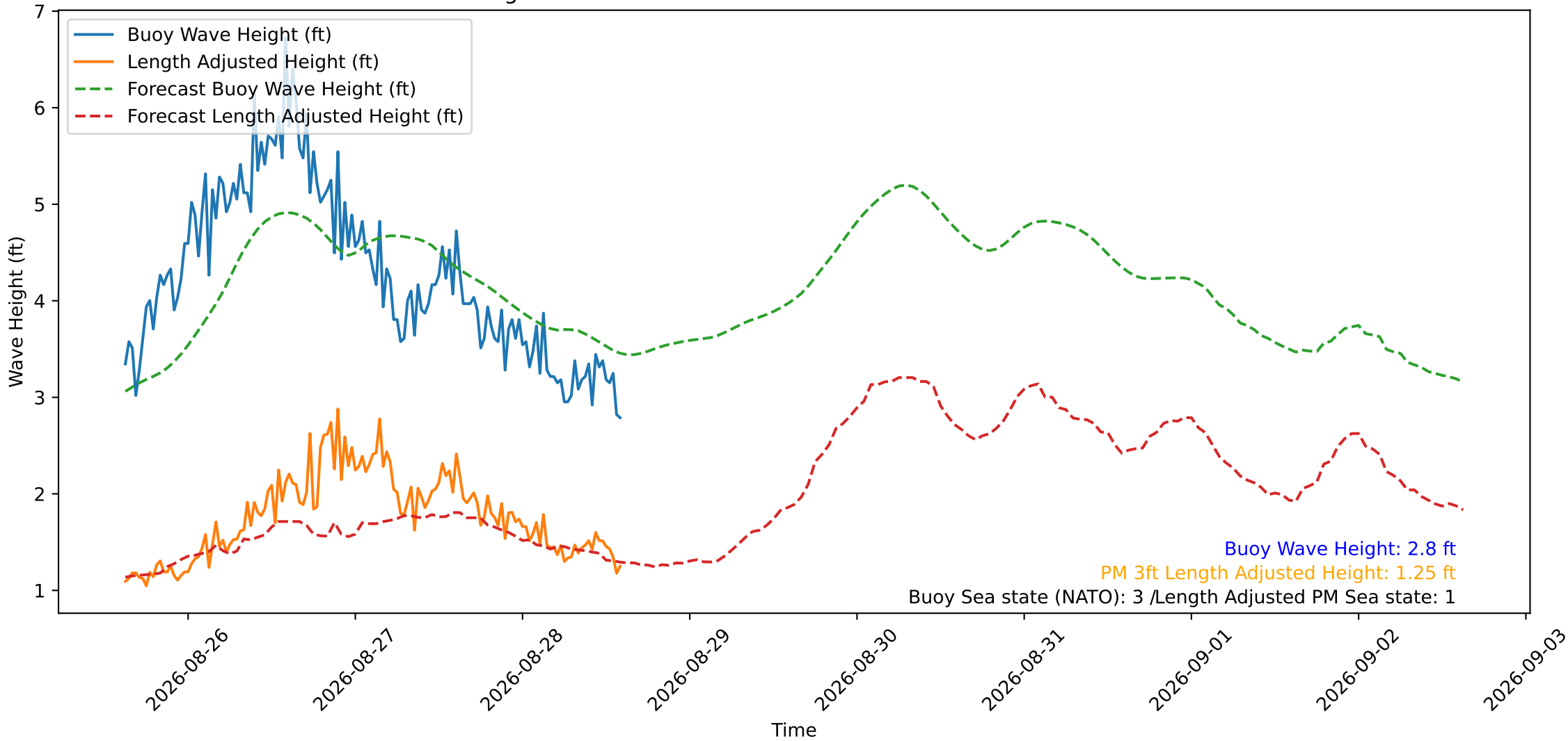
Wave Heights over Time for Oceanside Harbor at 2026-08-28 15:00:30
