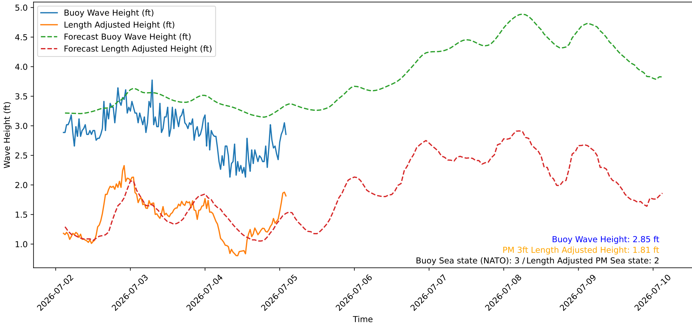
Wave Heights over Time for Oceanside Harbor at 2026-07-05 02:40:26
