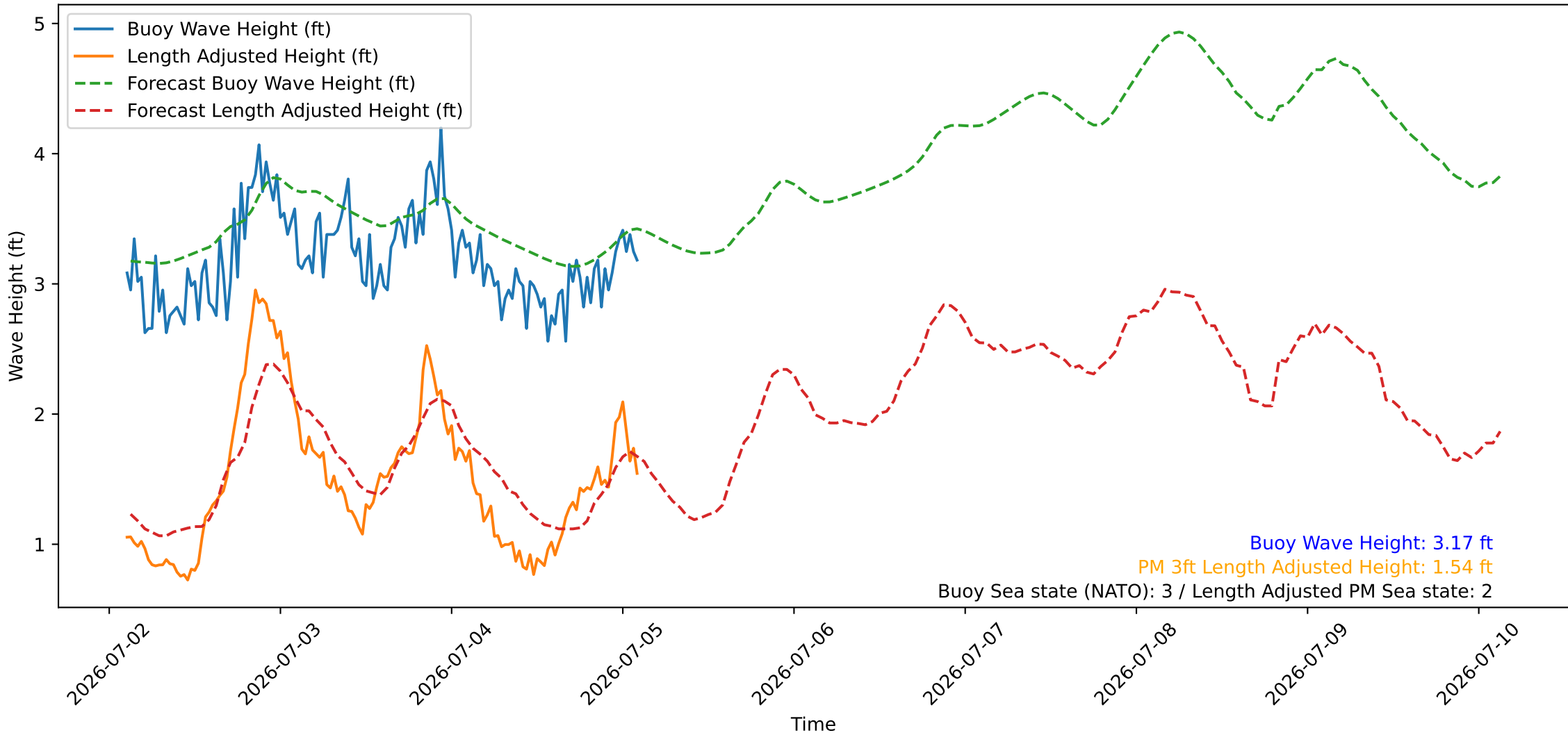
Wave Heights over Time for Green Beach at 2026-07-05 02:41:08
