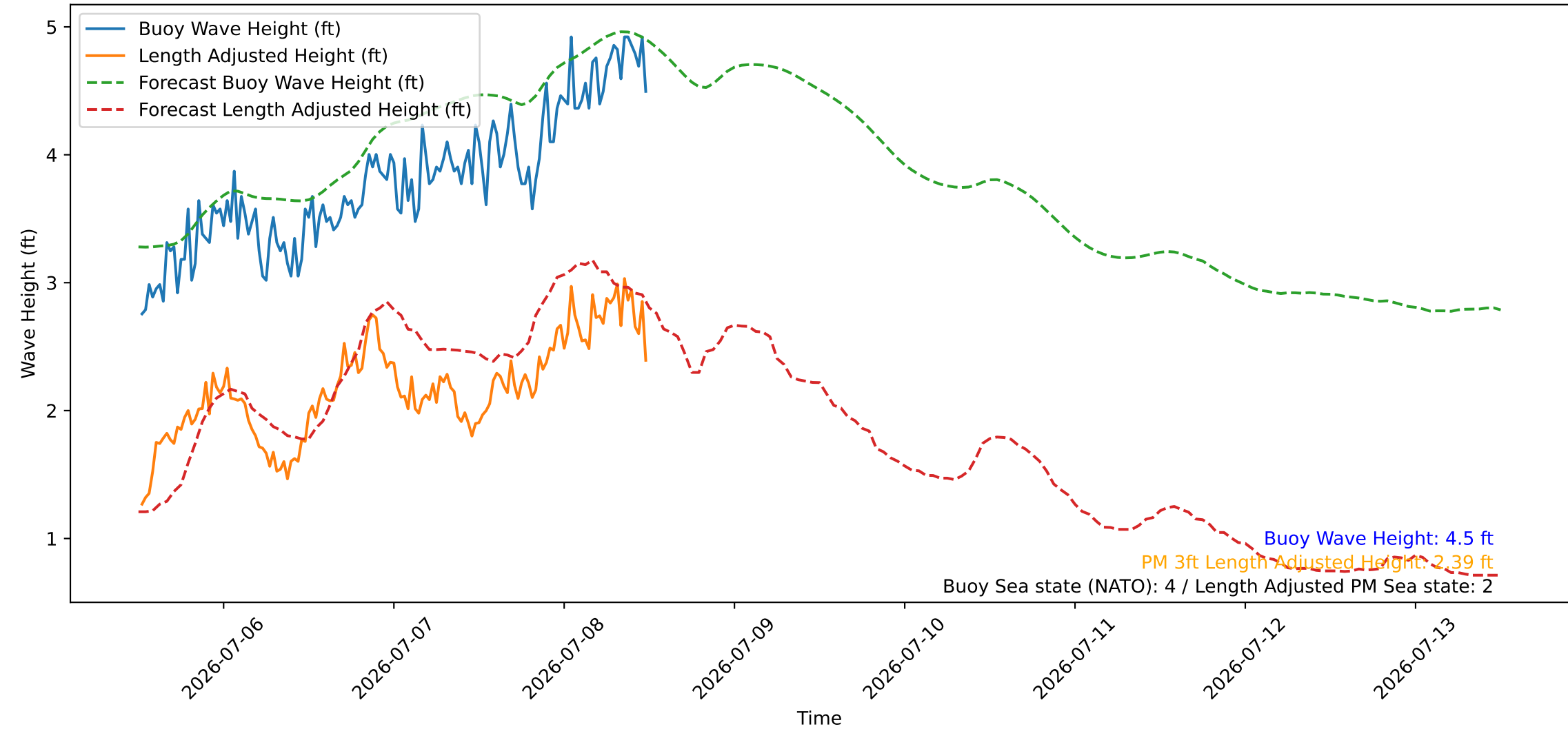
Wave Heights over Time for Oceanside Harbor at 2026-07-08 12:20:27
