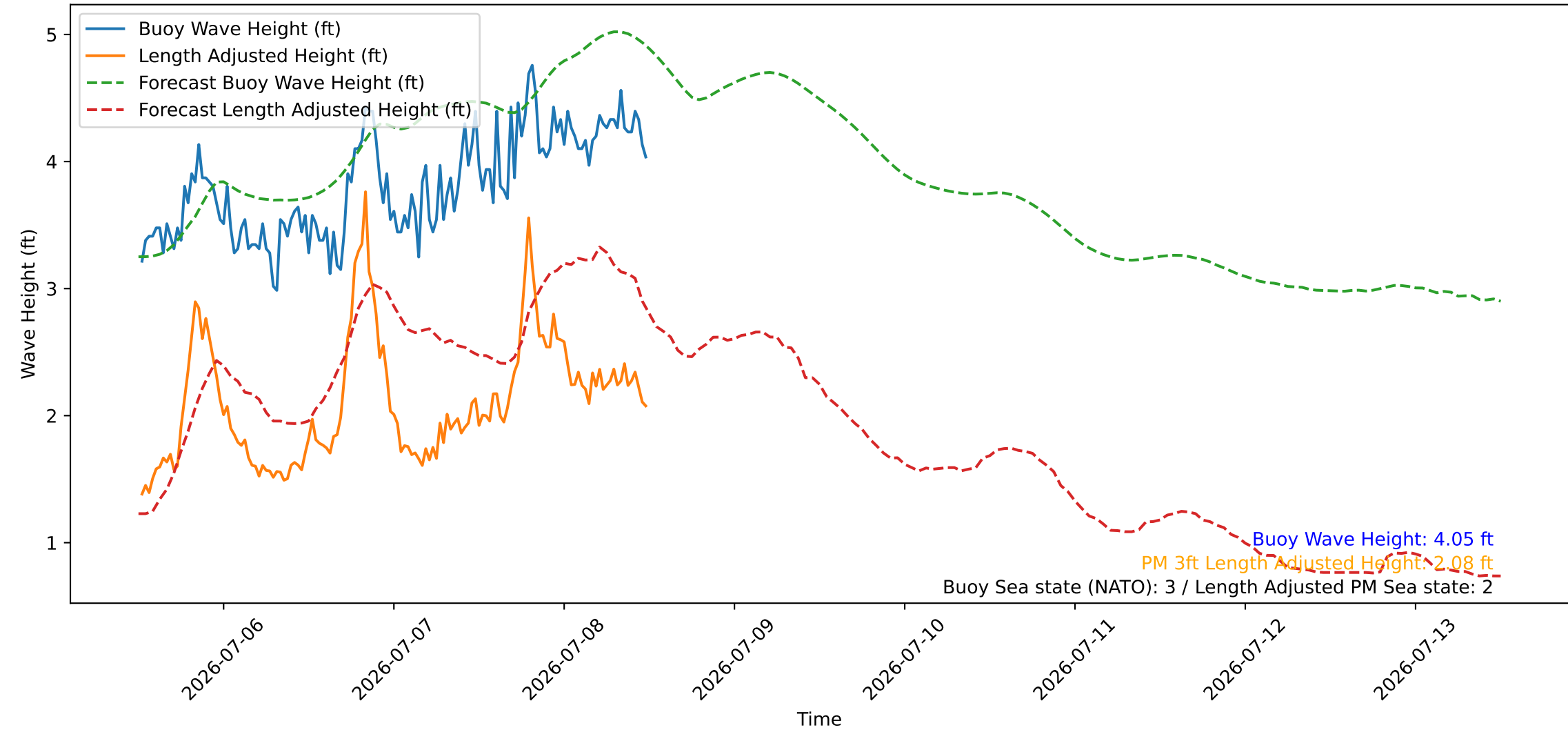
Wave Heights over Time for Green Beach at 2026-07-08 12:21:09
