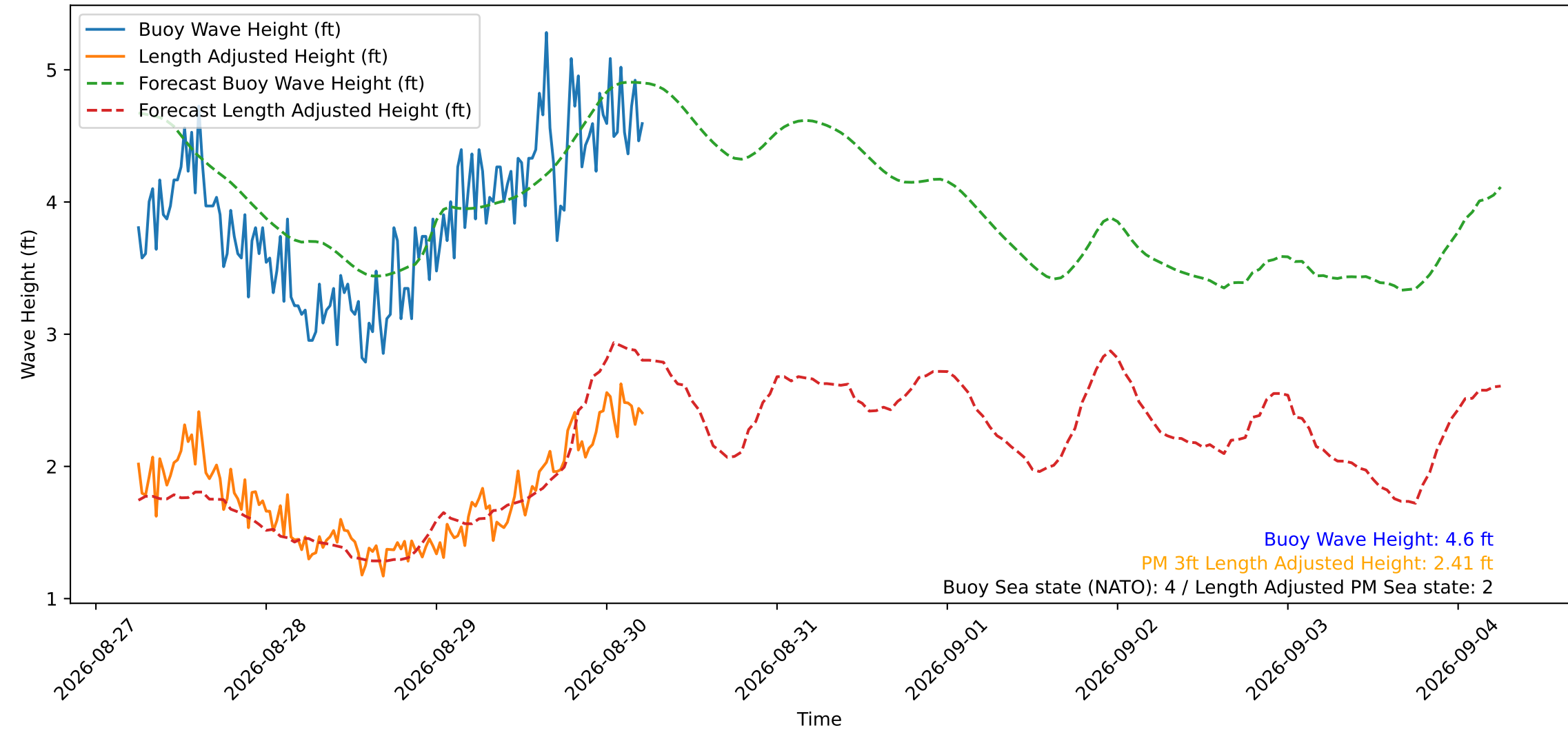
Wave Heights over Time for Oceanside Harbor at 2026-08-30 06:00:30
