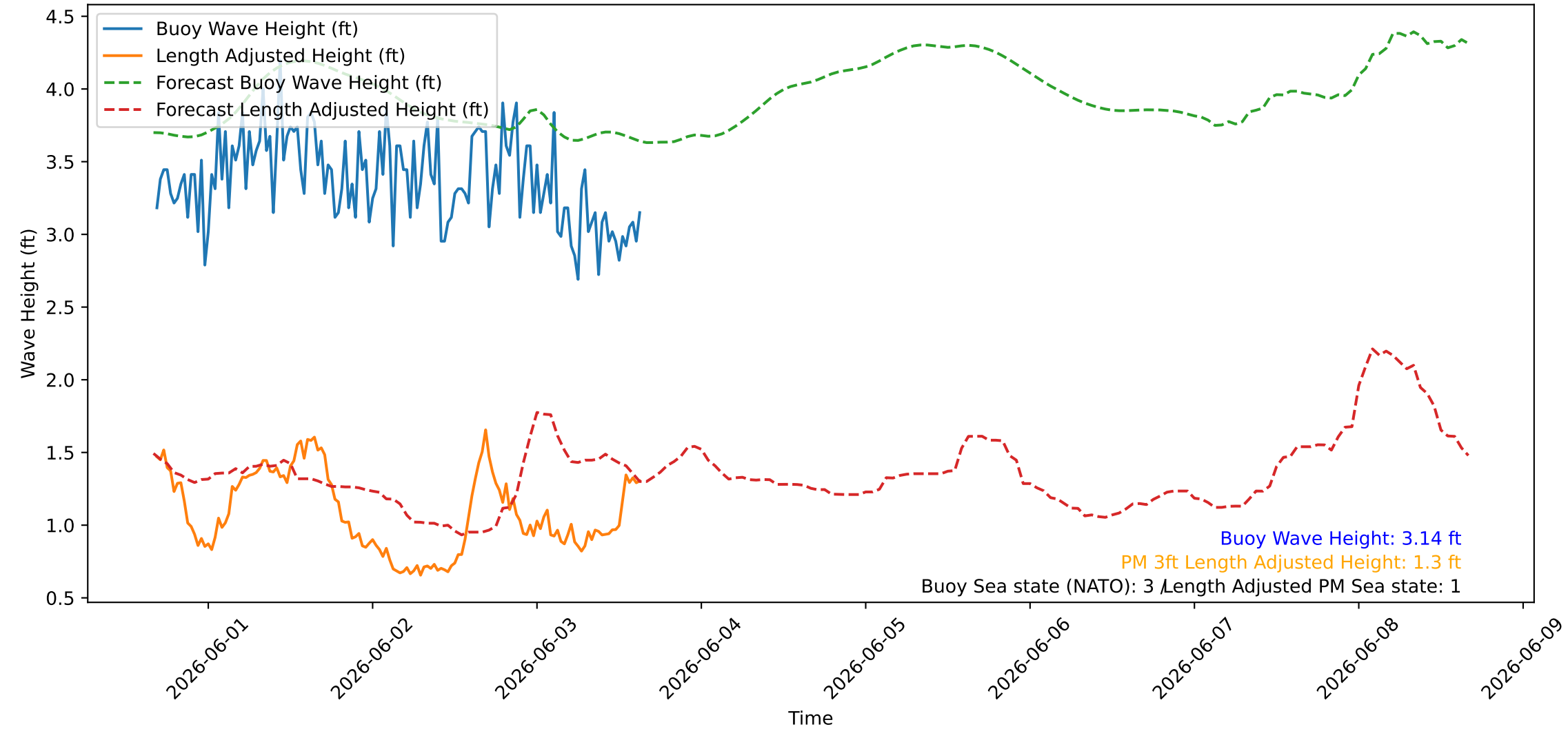
Wave Heights over Time for Red Beach at 2026-06-03 16:00:45
