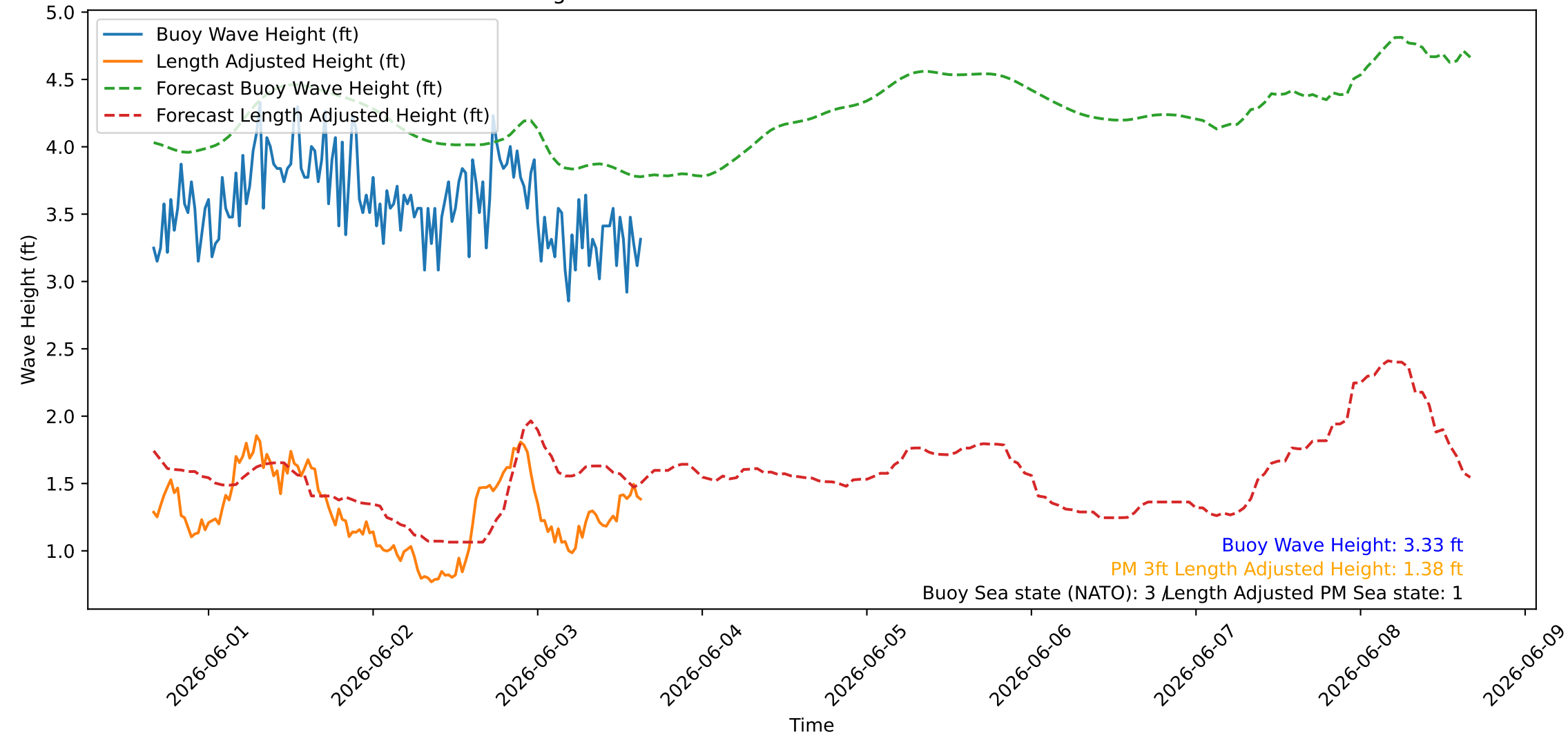
Wave Heights over Time for Green Beach at 2026-06-03 16:01:07
