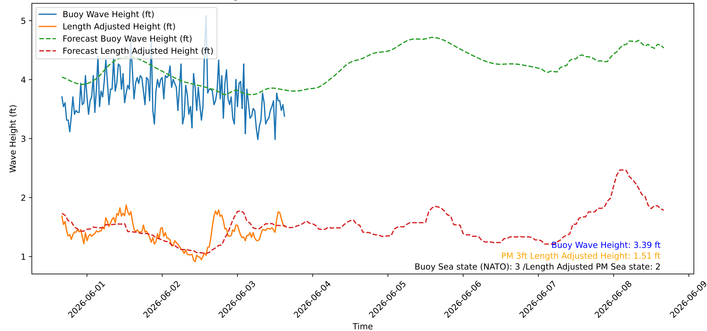
Wave Heights over Time for Oceanside Harbor at 2026-06-03 16:00:26
