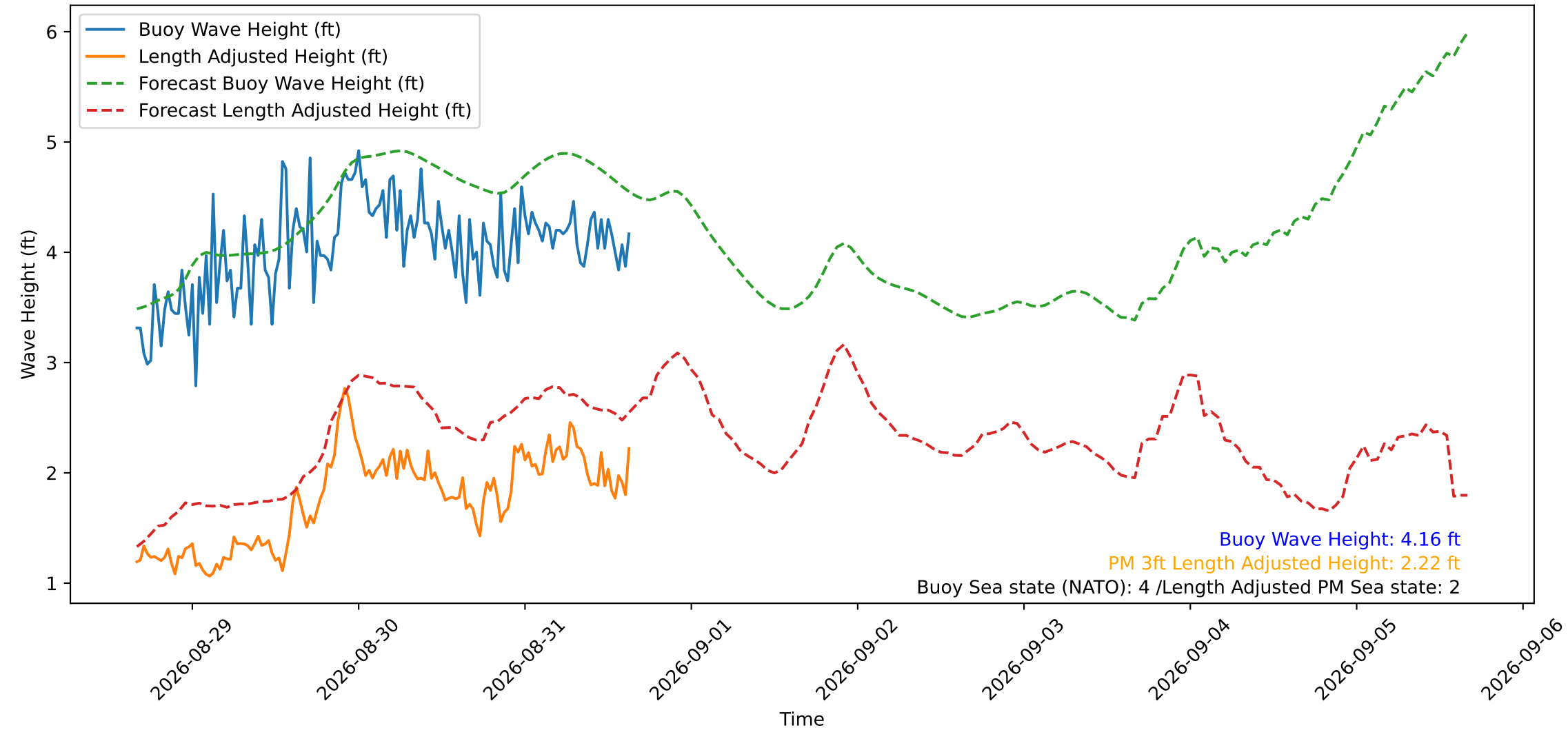
Wave Heights over Time for Green Beach at 2026-08-31 15:41:12
