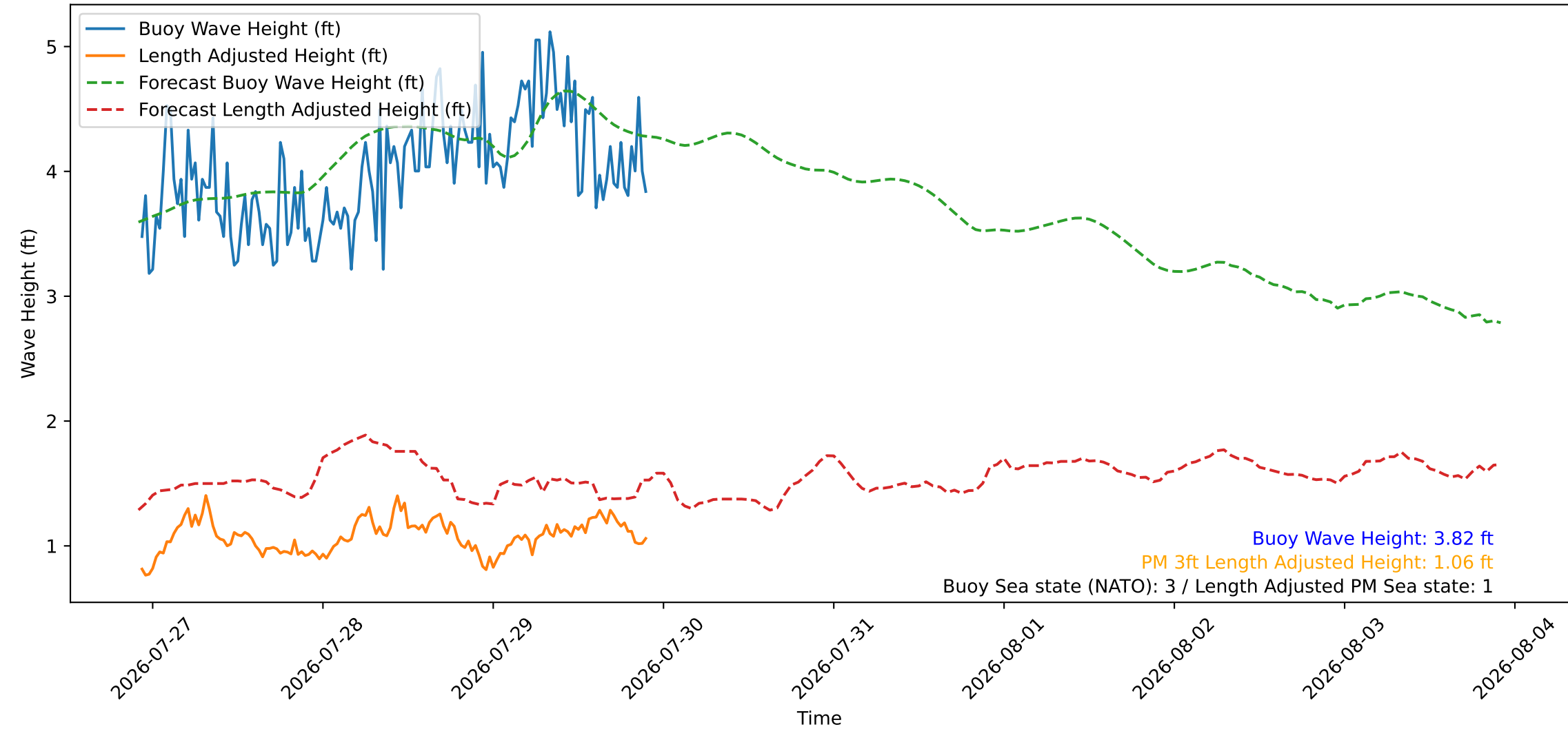
Wave Heights over Time for Red Beach at 2026-07-29 22:20:47
