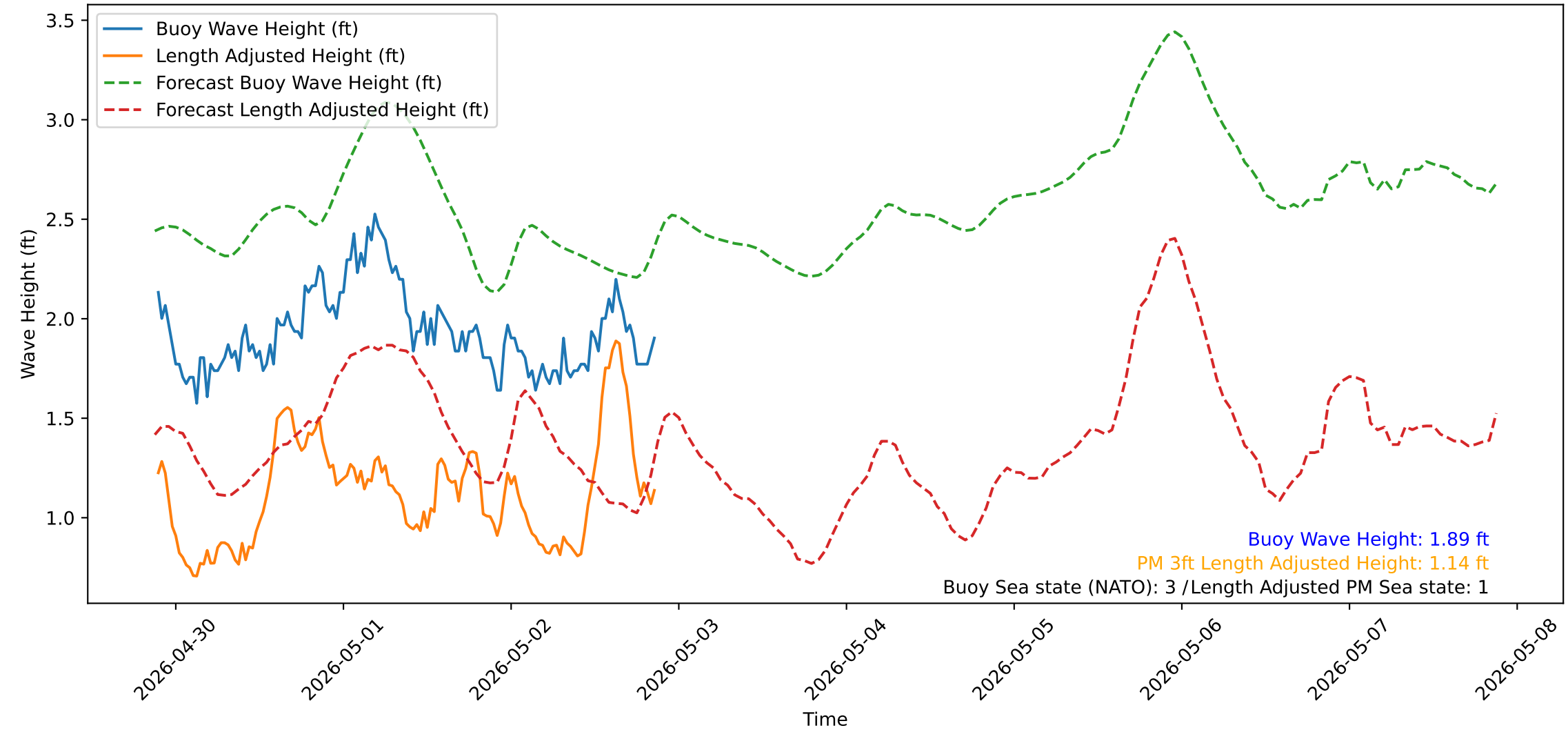
Wave Heights over Time for Red Beach at 2026-05-02 21:20:51
