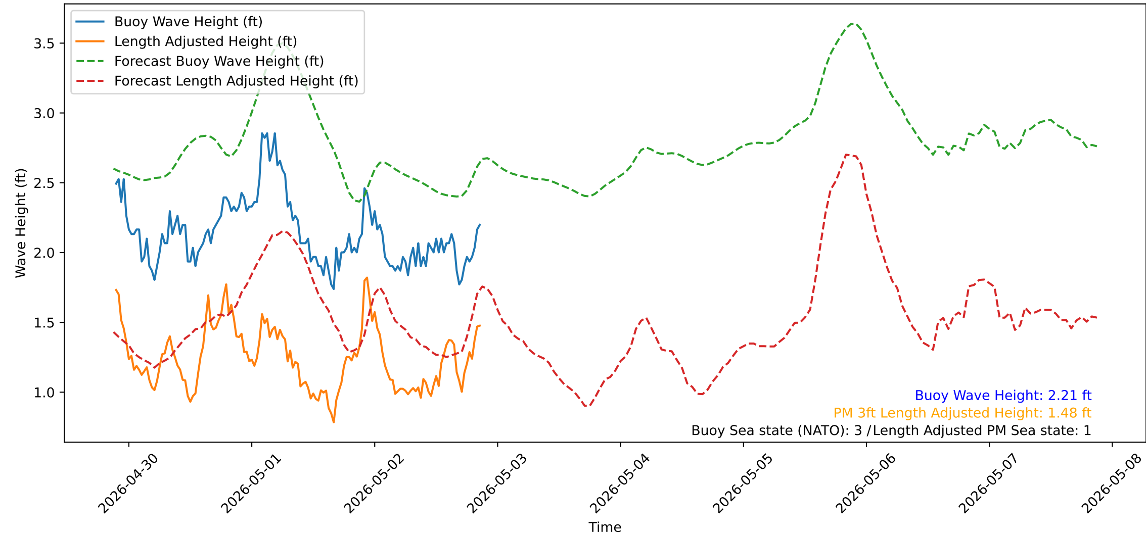
Wave Heights over Time for Green Beach at 2026-05-02 21:21:13
