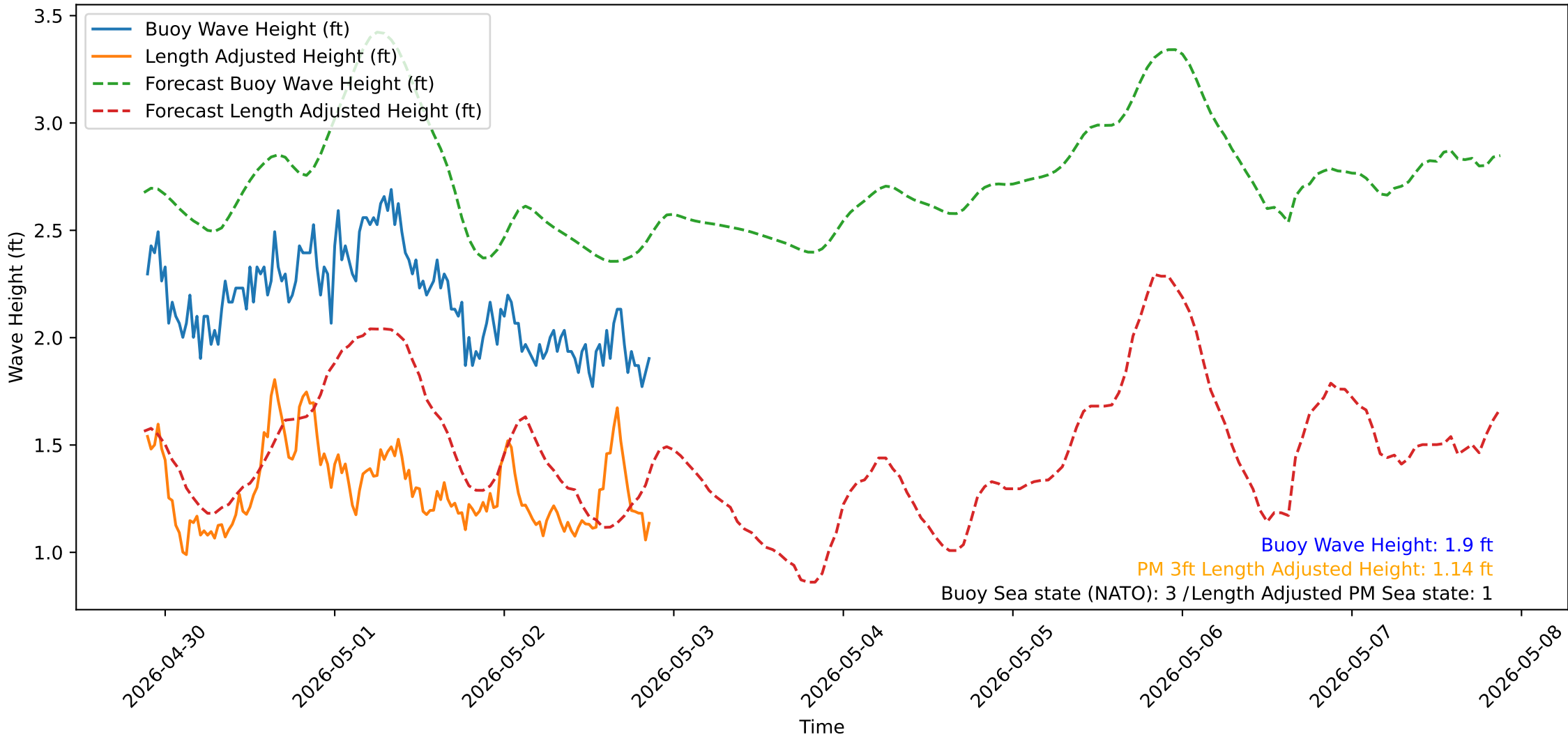
Wave Heights over Time for Oceanside Harbor at 2026-05-02 21:20:31
