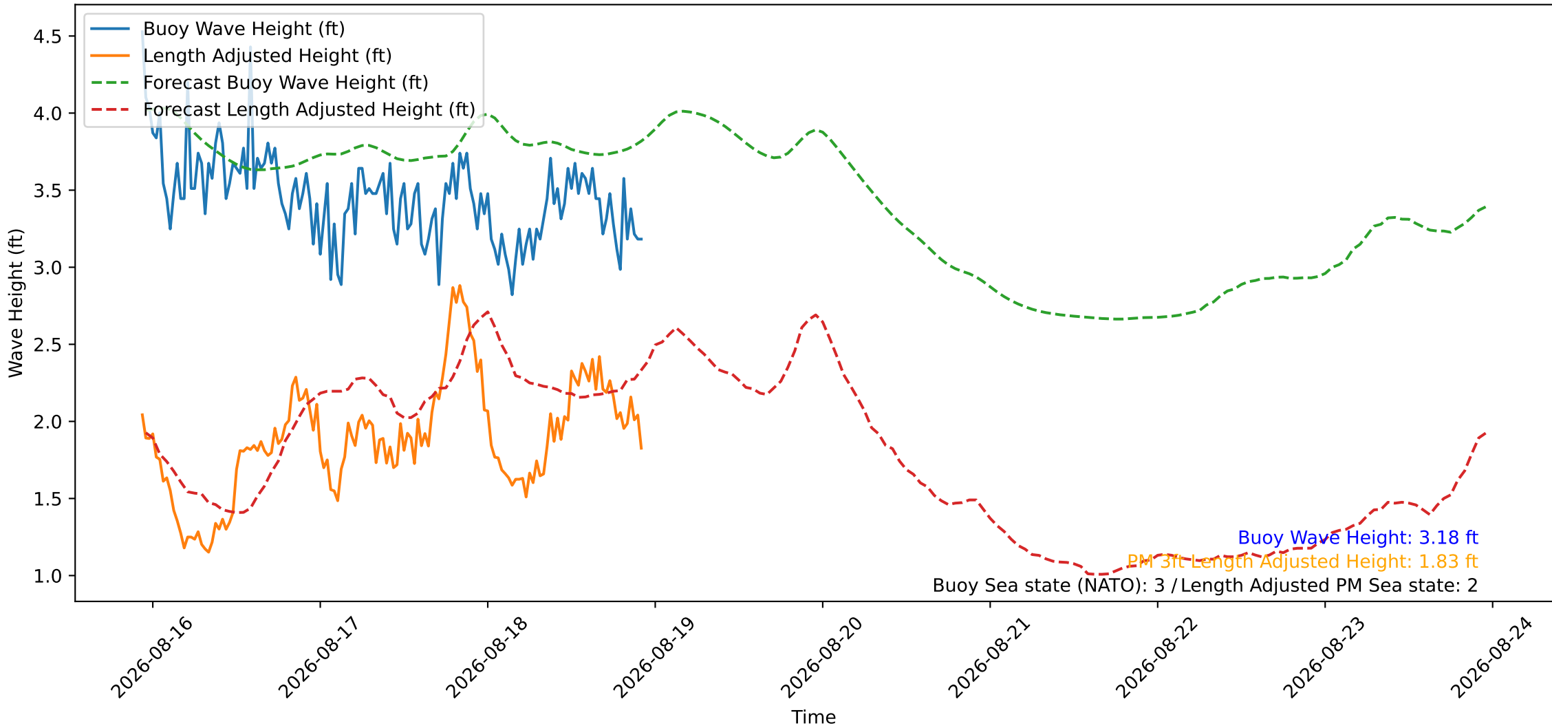
Wave Heights over Time for Oceanside Harbor at 2026-08-18 22:30:27
