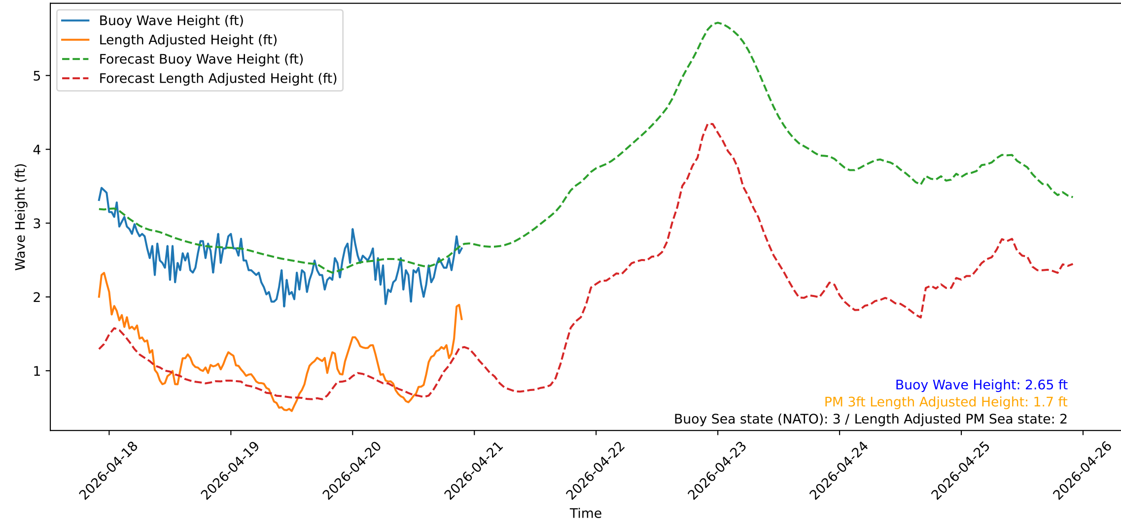
Wave Heights over Time for Green Beach at 2026-04-20 22:11:13
