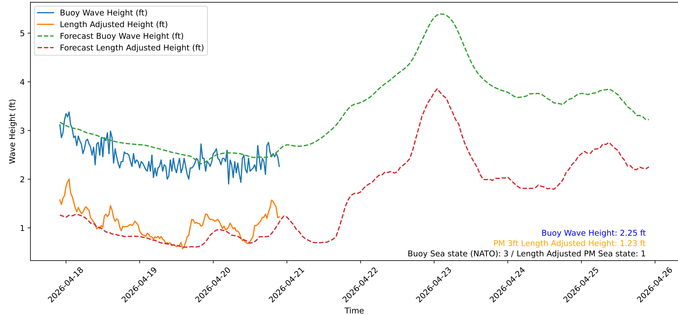
Wave Heights over Time for Oceanside Harbor at 2026-04-20 22:10:32
