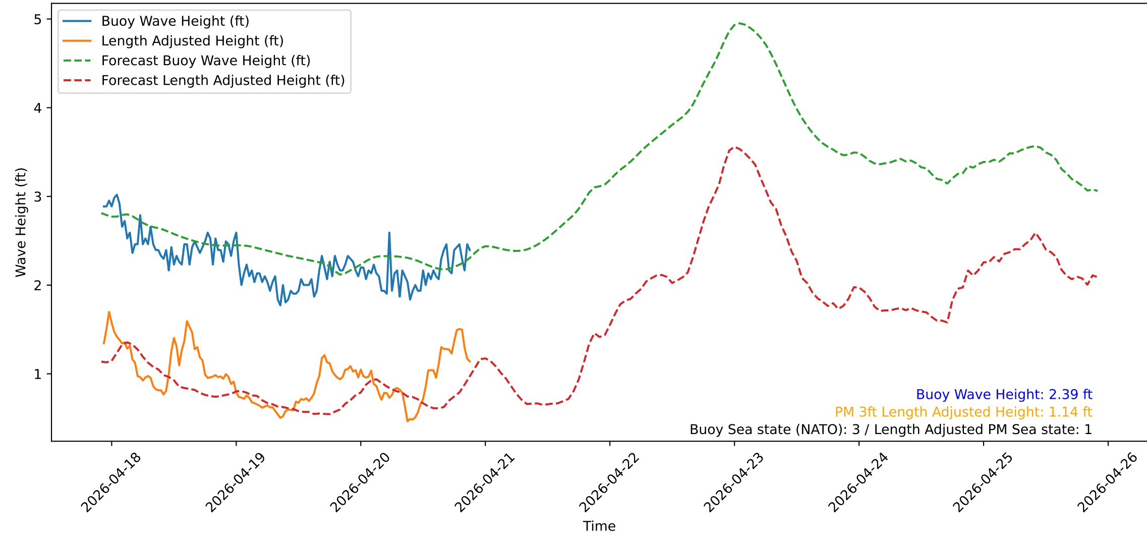
Wave Heights over Time for Red Beach at 2026-04-20 22:10:51
