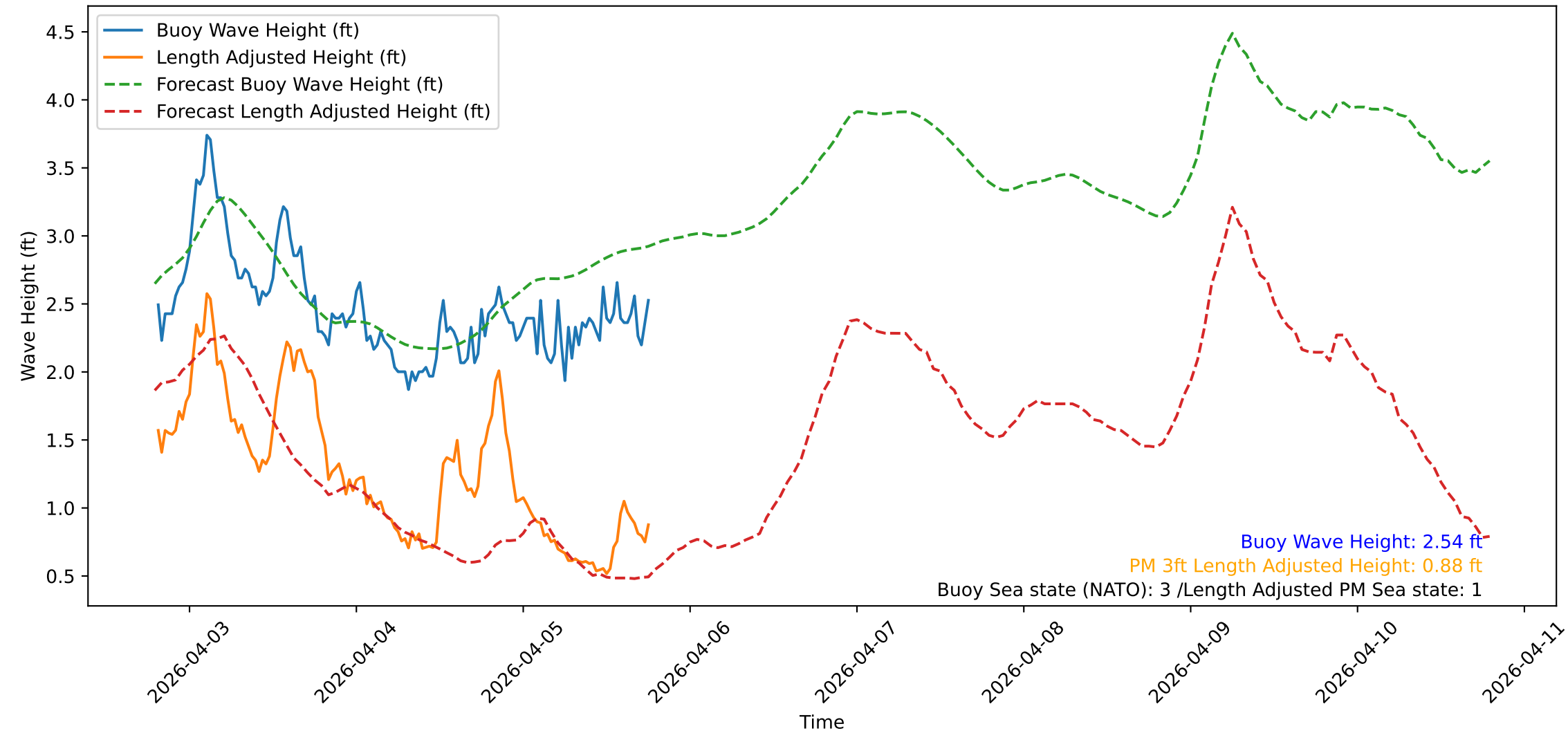
Wave Heights over Time for Red Beach at 2026-04-05 19:00:50
