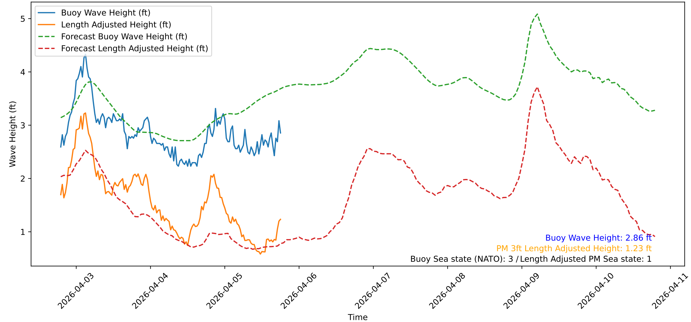
Wave Heights over Time for Green Beach at 2026-04-05 19:01:15
