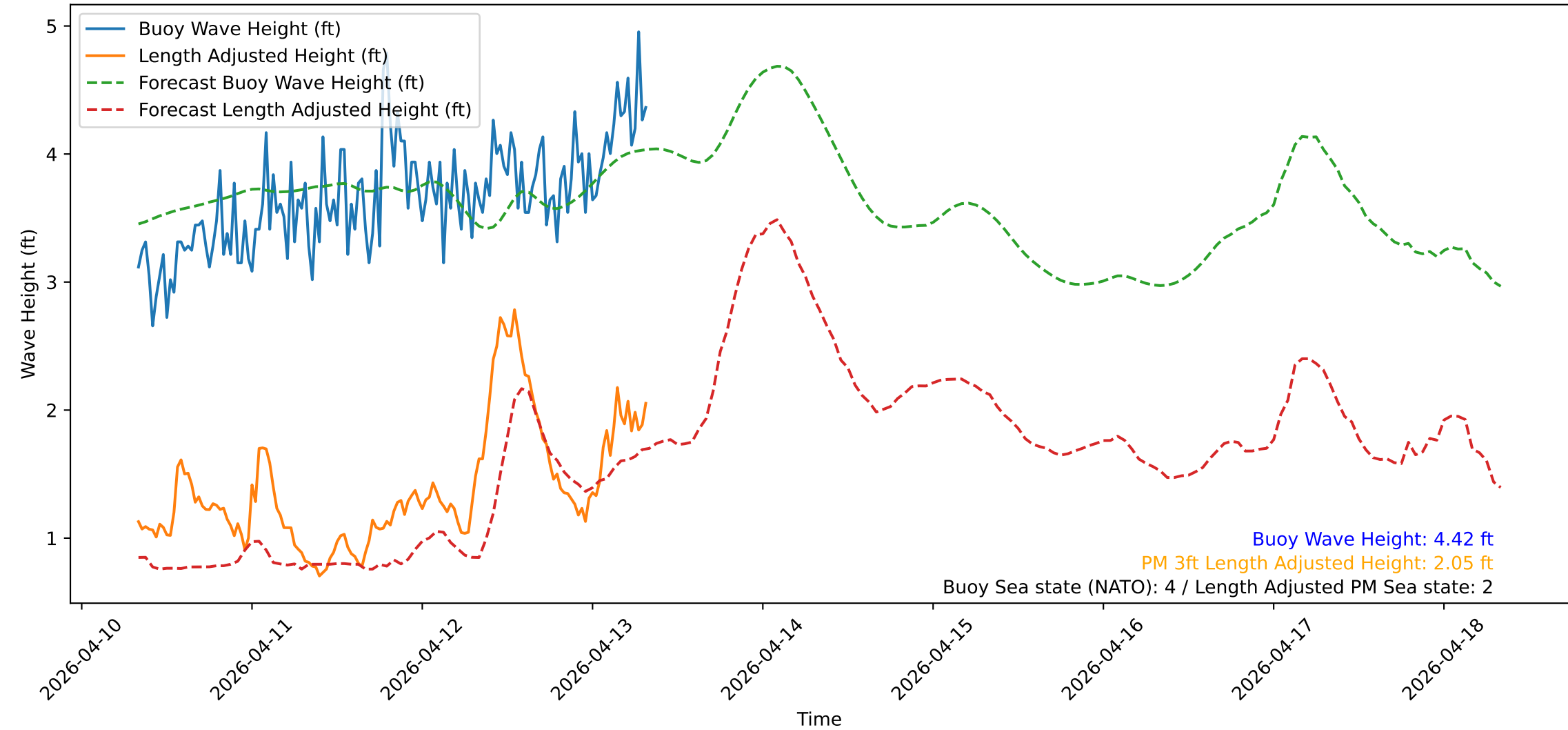
Wave Heights over Time for Oceanside Harbor at 2026-04-13 08:10:30
