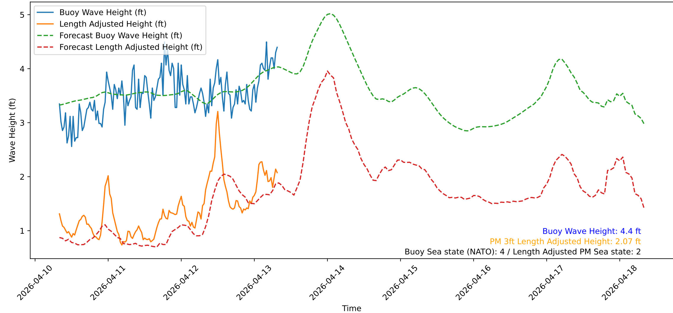
Wave Heights over Time for Green Beach at 2026-04-13 08:11:12
