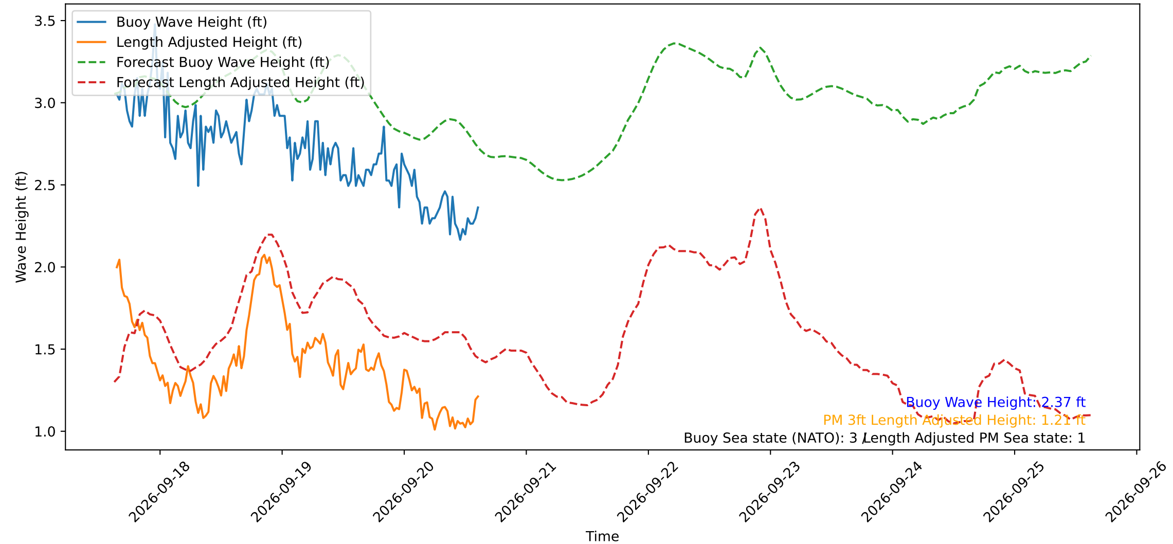
Wave Heights over Time for Green Beach at 2026-09-20 15:21:14
