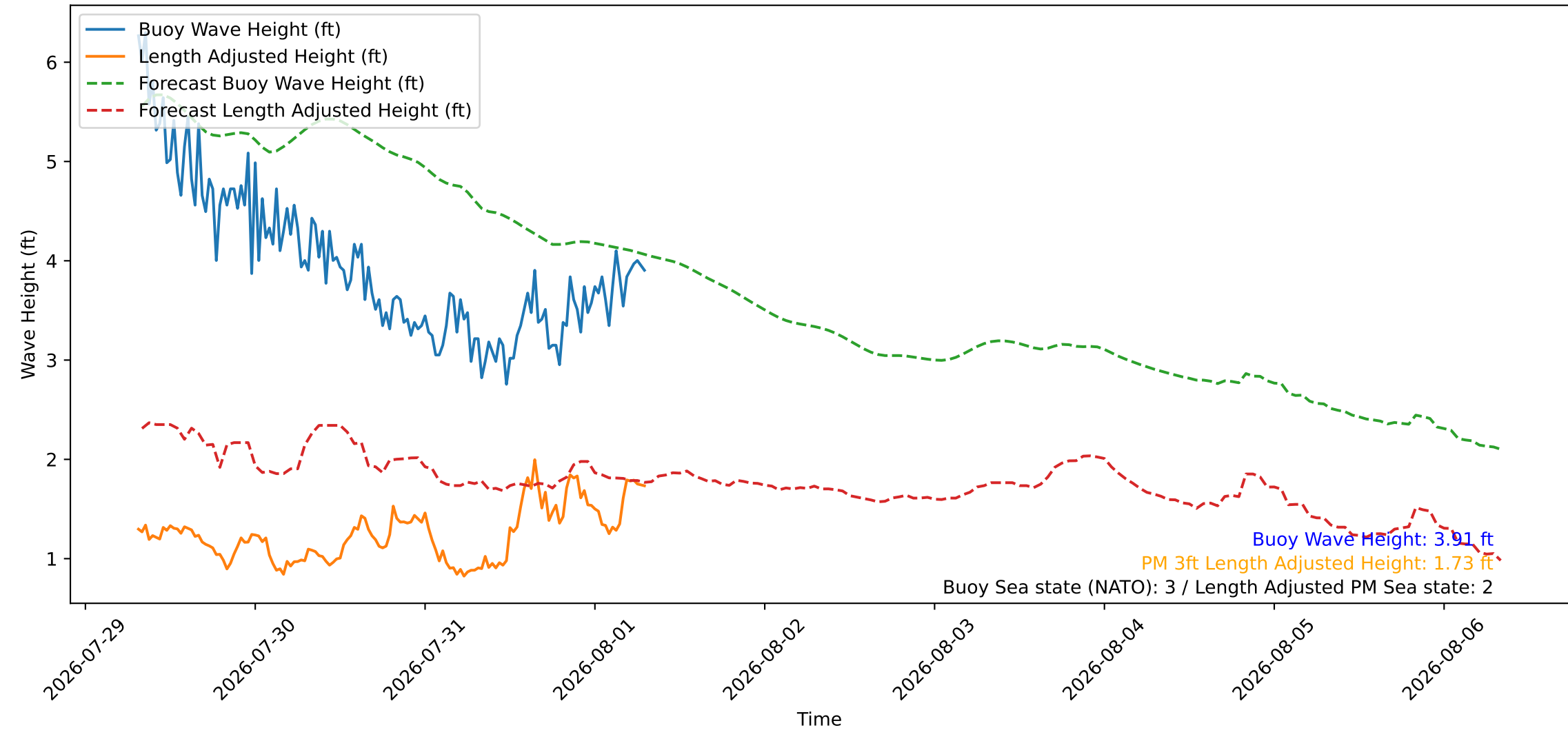
Wave Heights over Time for Green Beach at 2026-08-01 07:41:09
