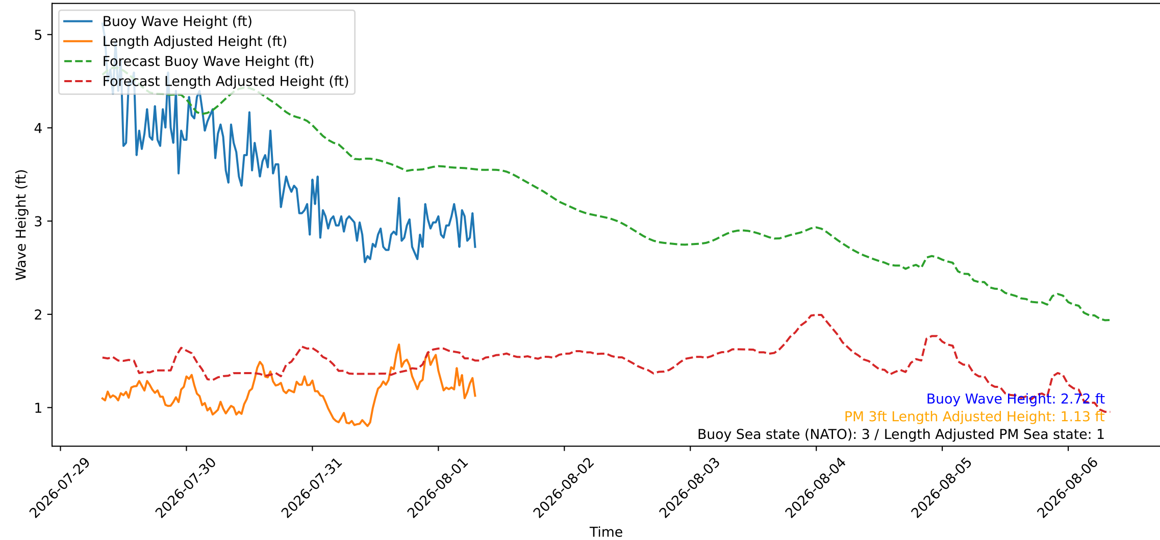
Wave Heights over Time for Red Beach at 2026-08-01 07:40:46
