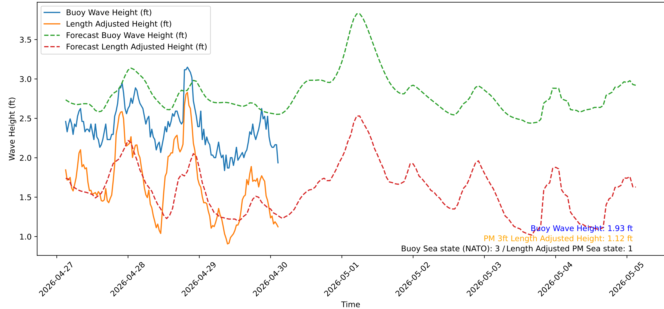
Wave Heights over Time for Green Beach at 2026-04-30 03:11:13
