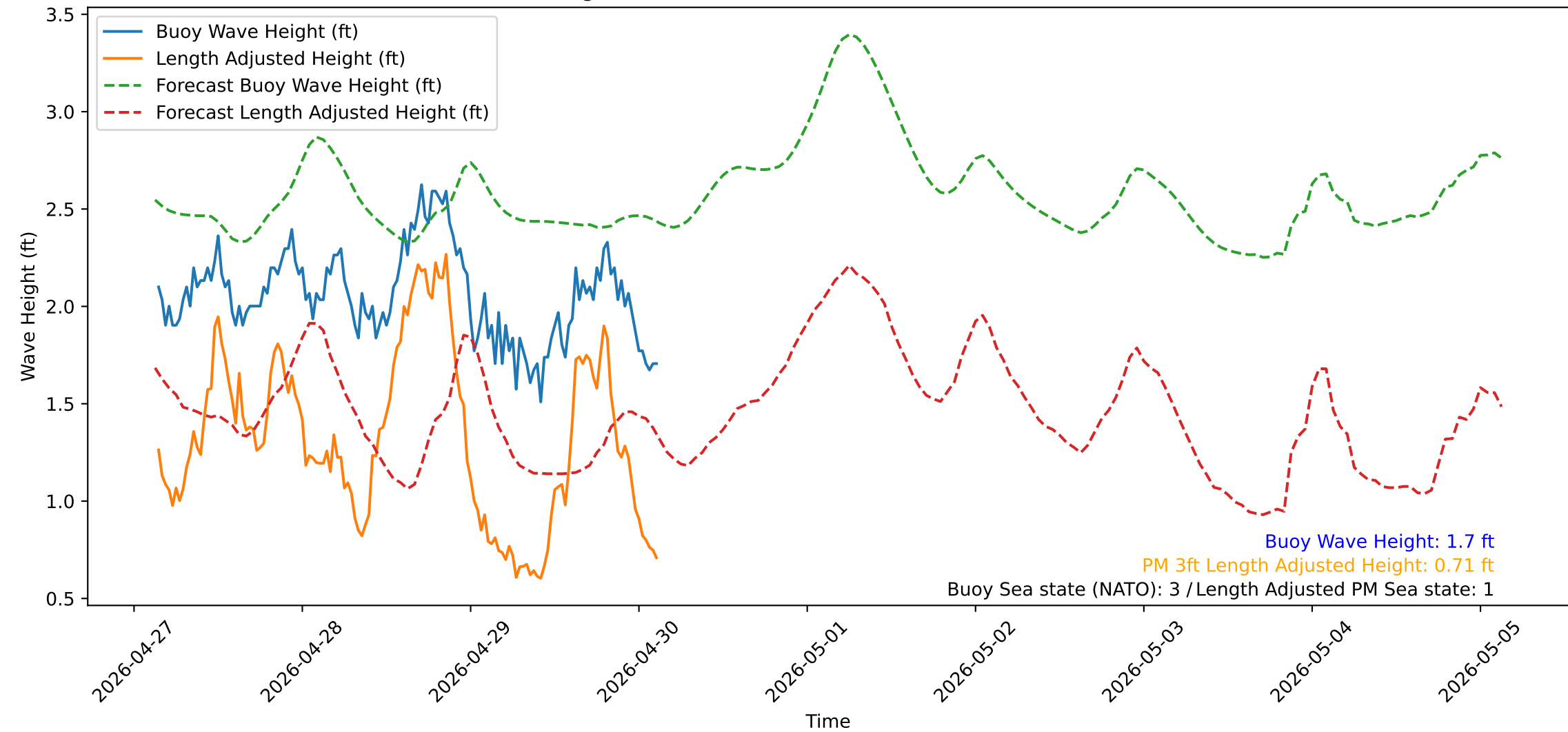
Wave Heights over Time for Red Beach at 2026-04-30 03:10:50
