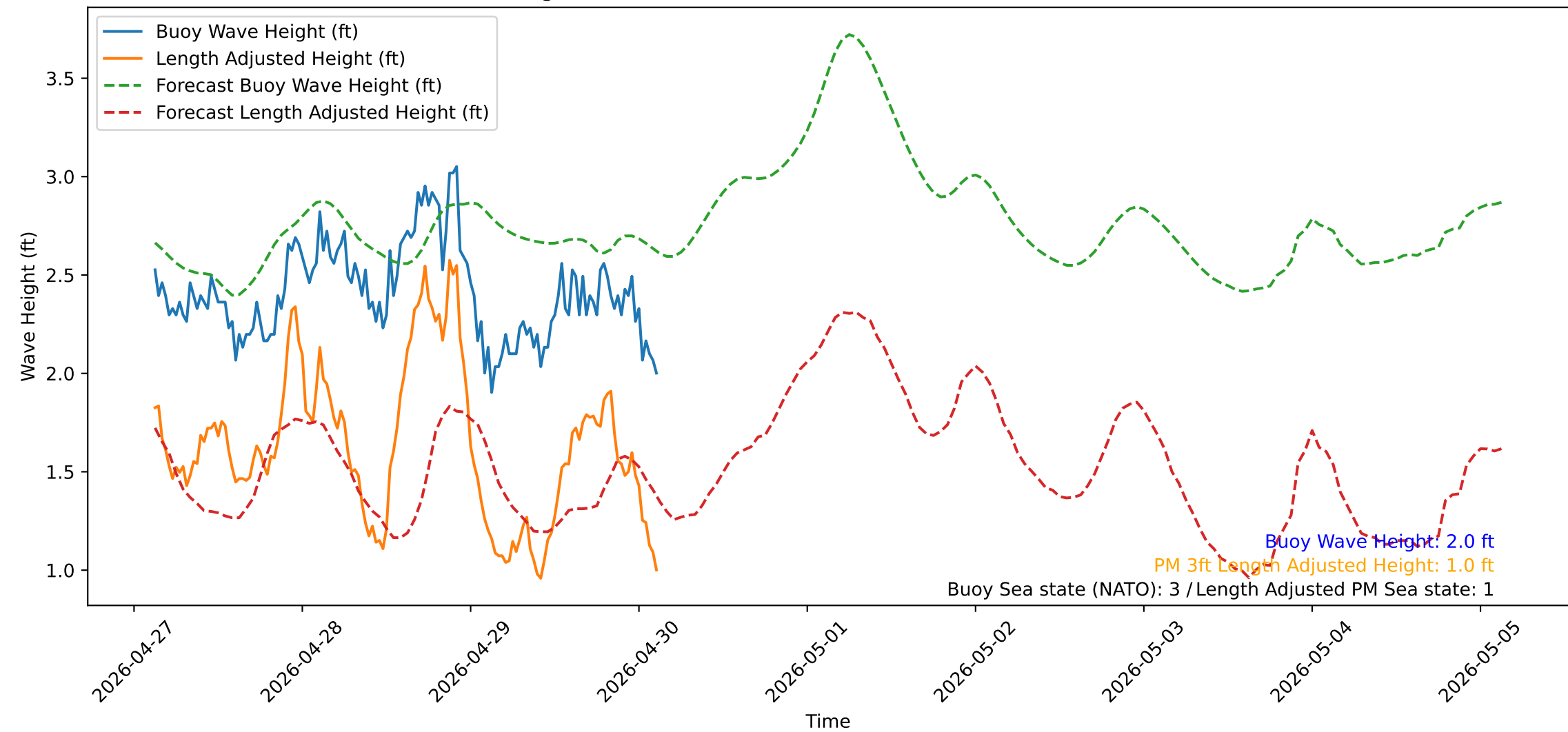
Wave Heights over Time for Oceanside Harbor at 2026-04-30 03:10:31
