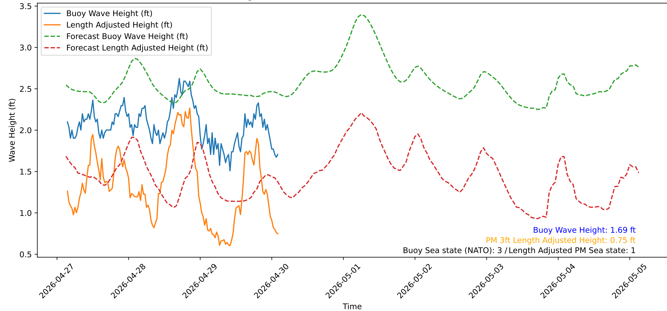
Wave Heights over Time for Red Beach at 2026-04-30 03:00:50
