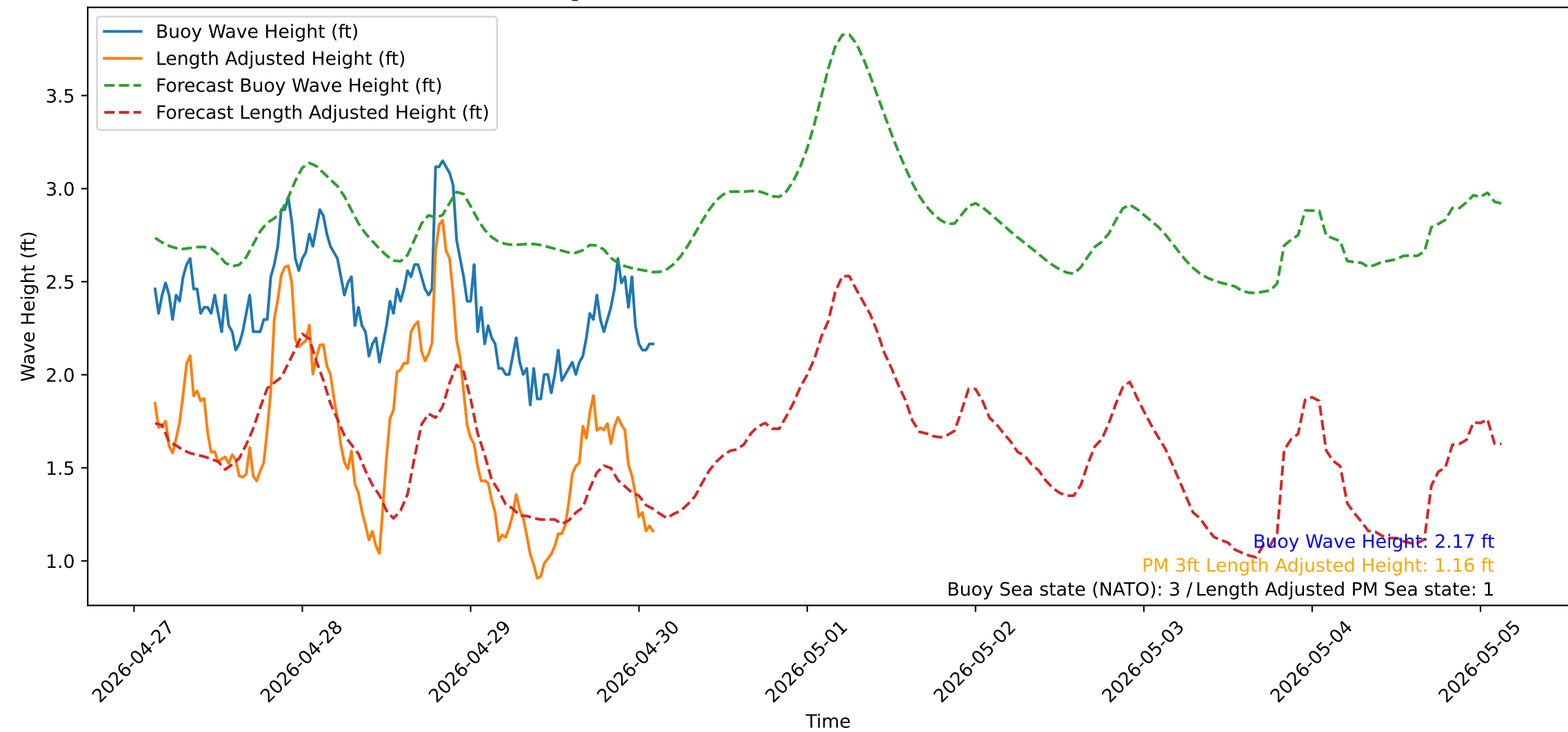
Wave Heights over Time for Green Beach at 2026-04-30 03:01:13
