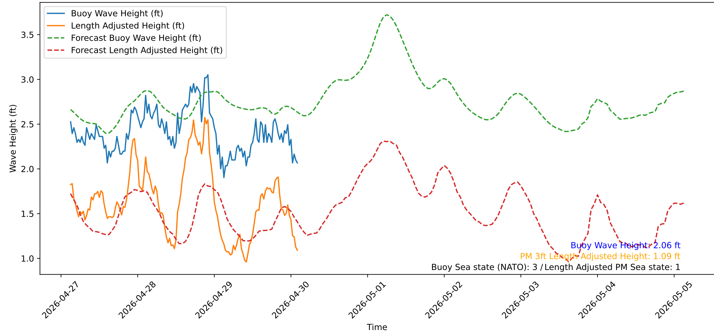
Wave Heights over Time for Oceanside Harbor at 2026-04-30 03:00:31
