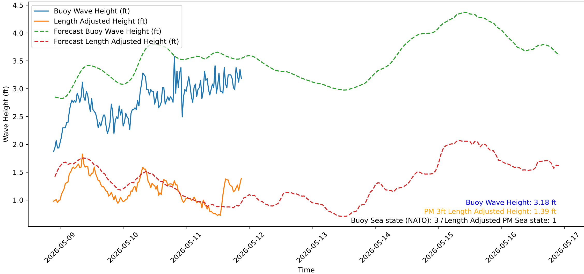
Wave Heights over Time for Oceanside Harbor at 2026-05-11 21:40:31
