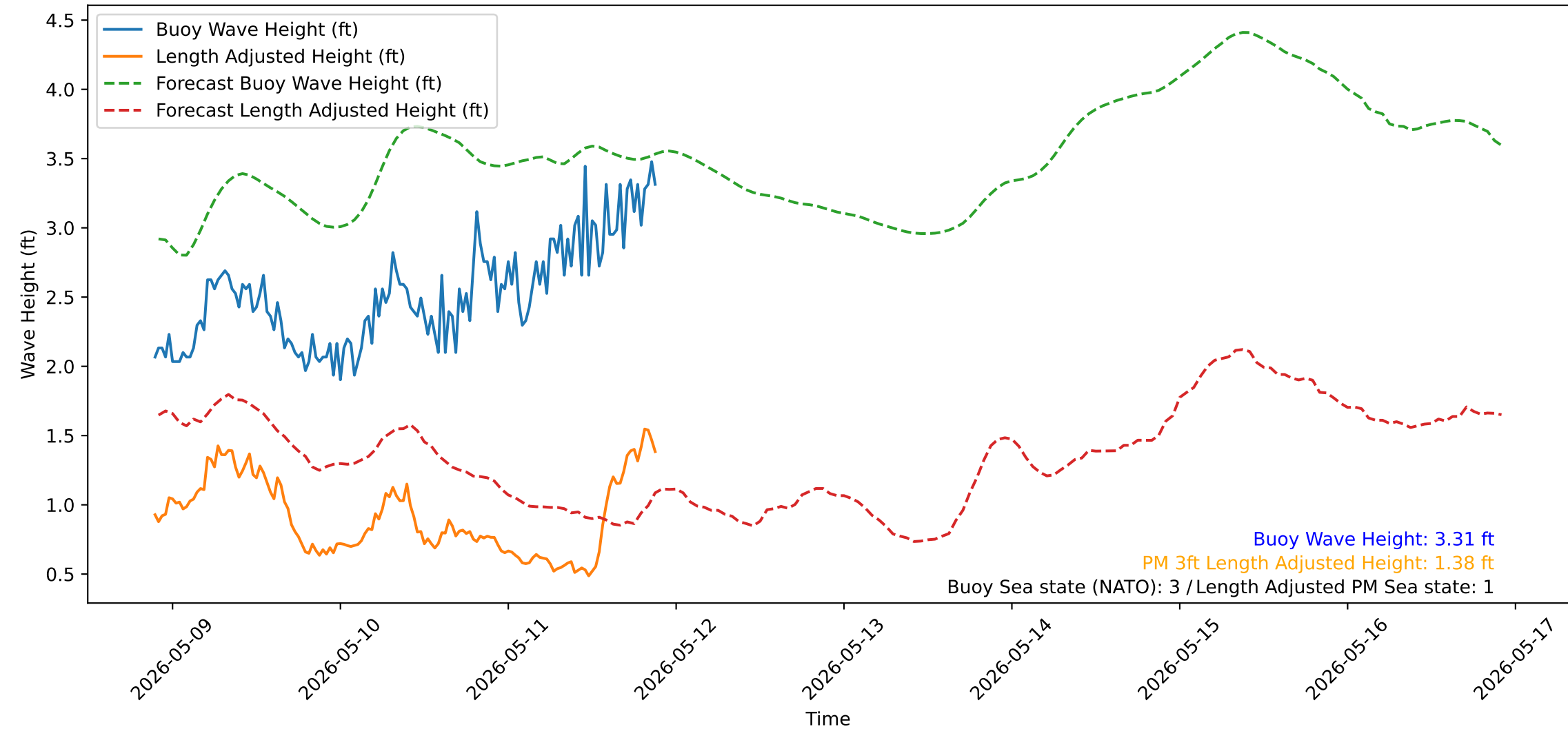
Wave Heights over Time for Green Beach at 2026-05-11 21:41:13
