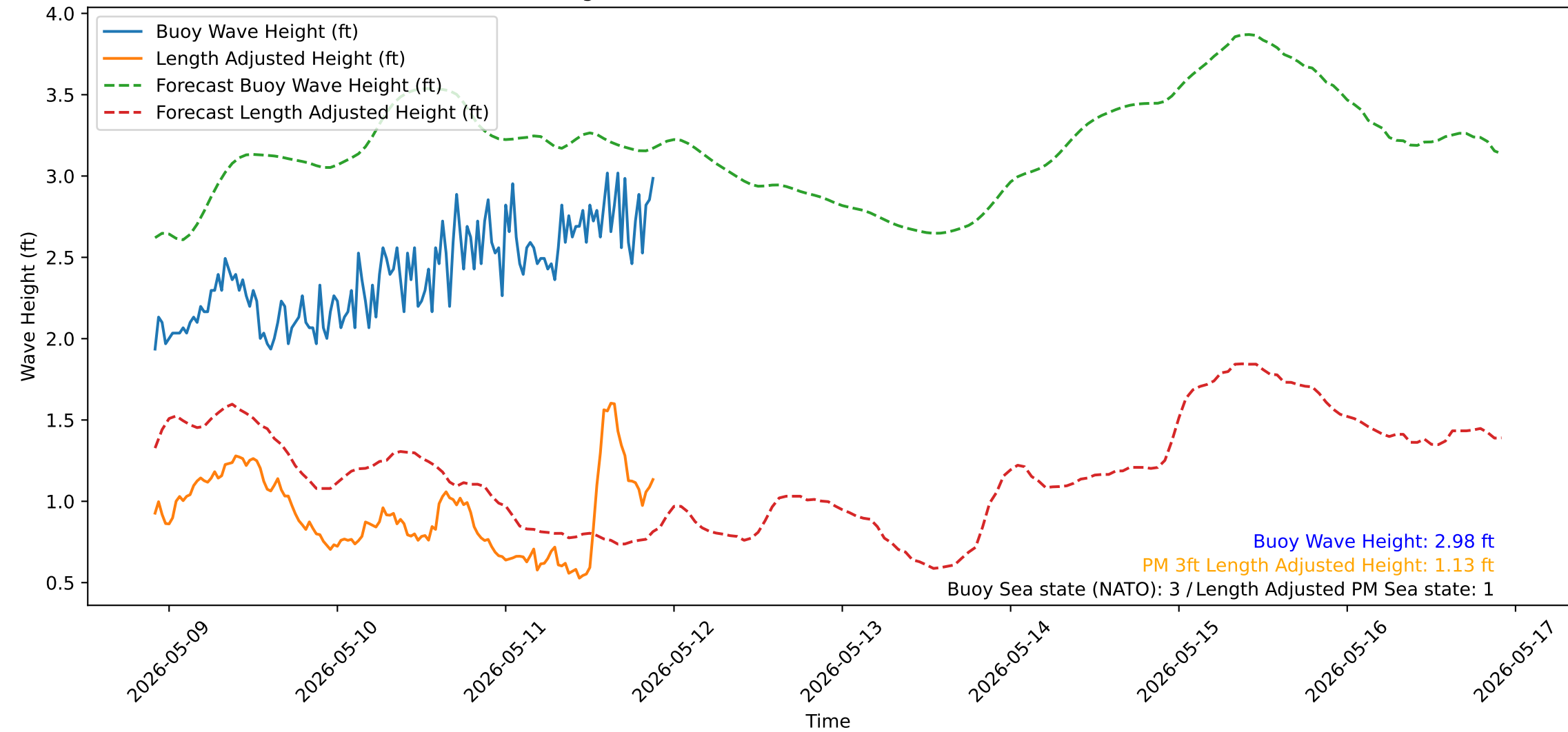
Wave Heights over Time for Red Beach at 2026-05-11 21:40:50
