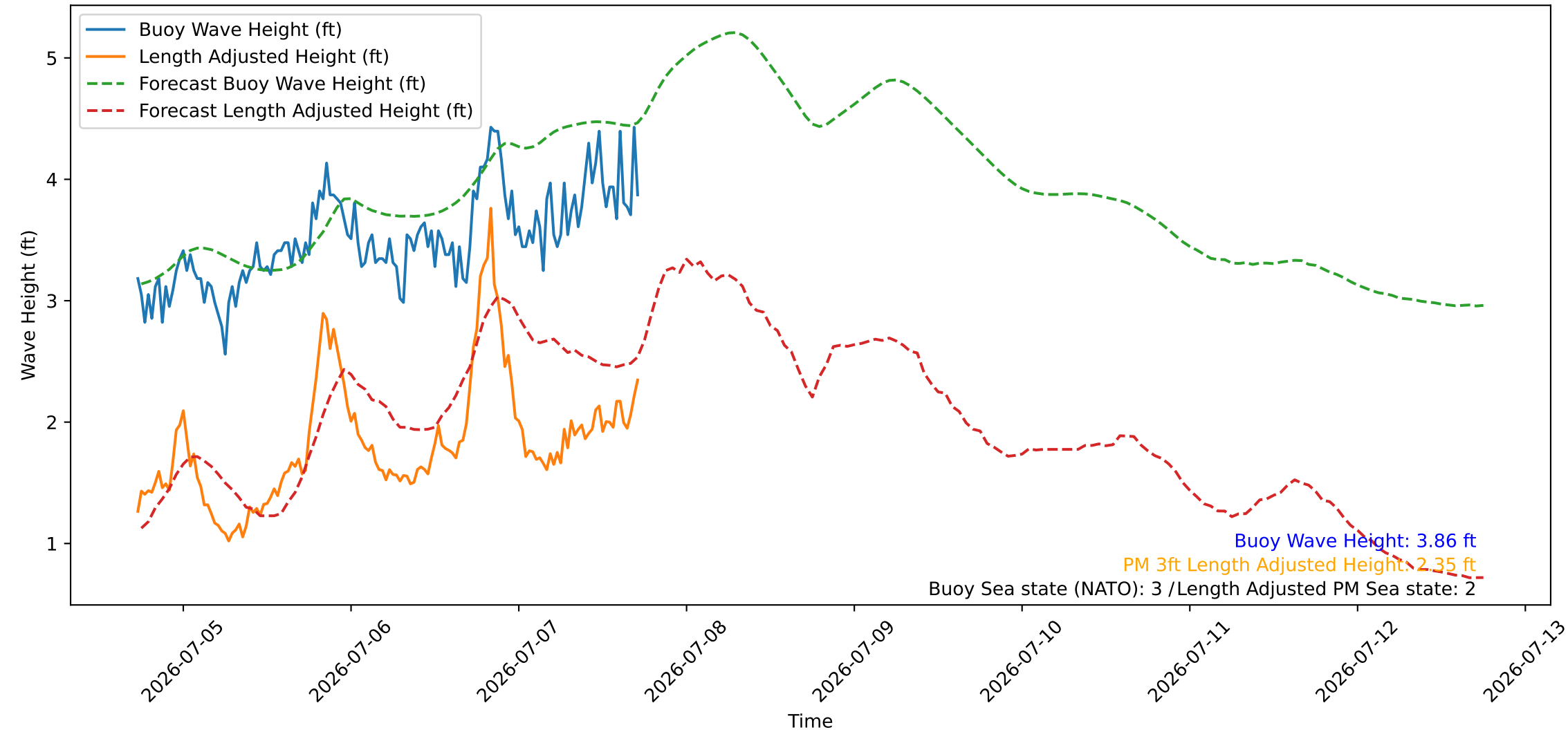
Wave Heights over Time for Green Beach at 2026-07-07 17:41:08
