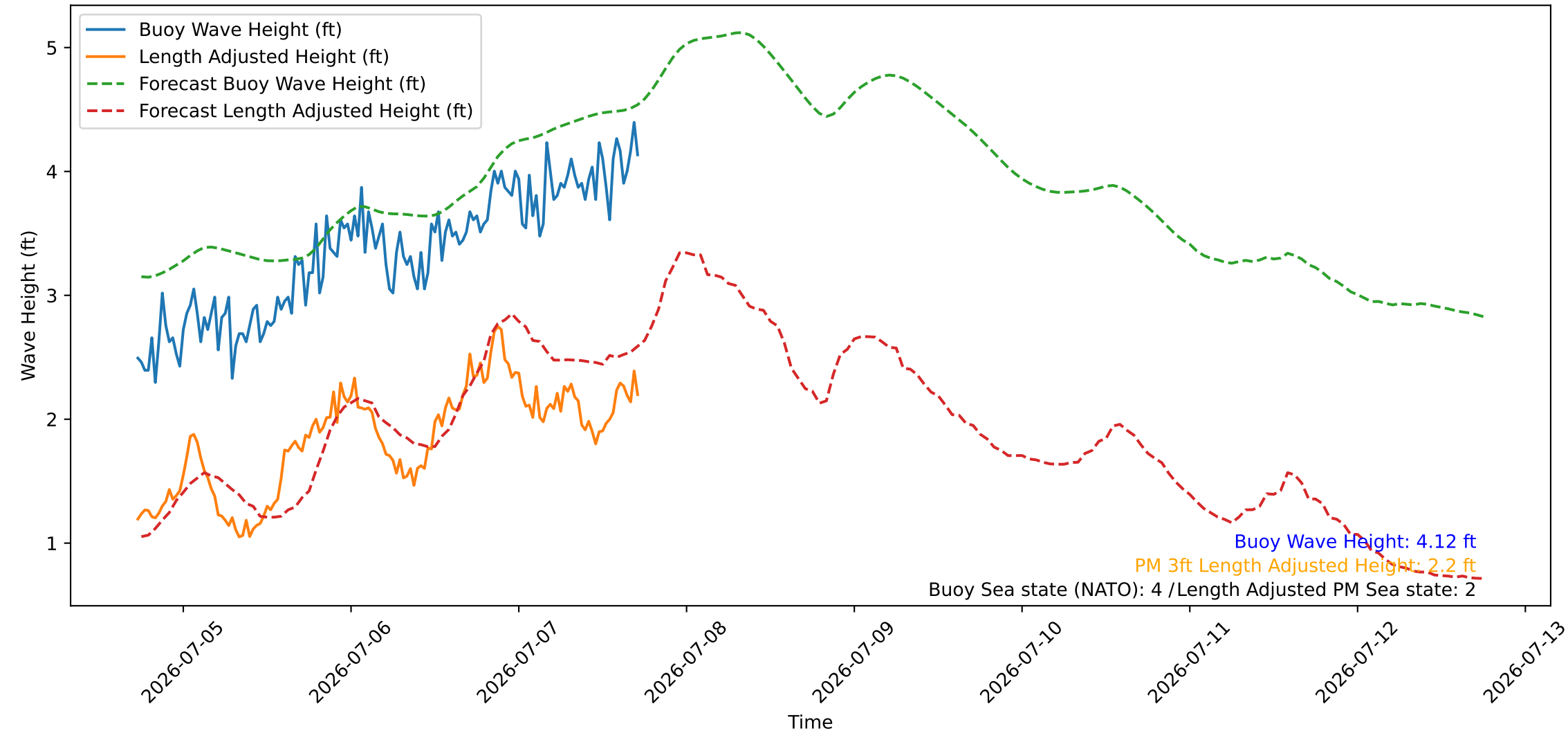
Wave Heights over Time for Oceanside Harbor at 2026-07-07 17:40:26
