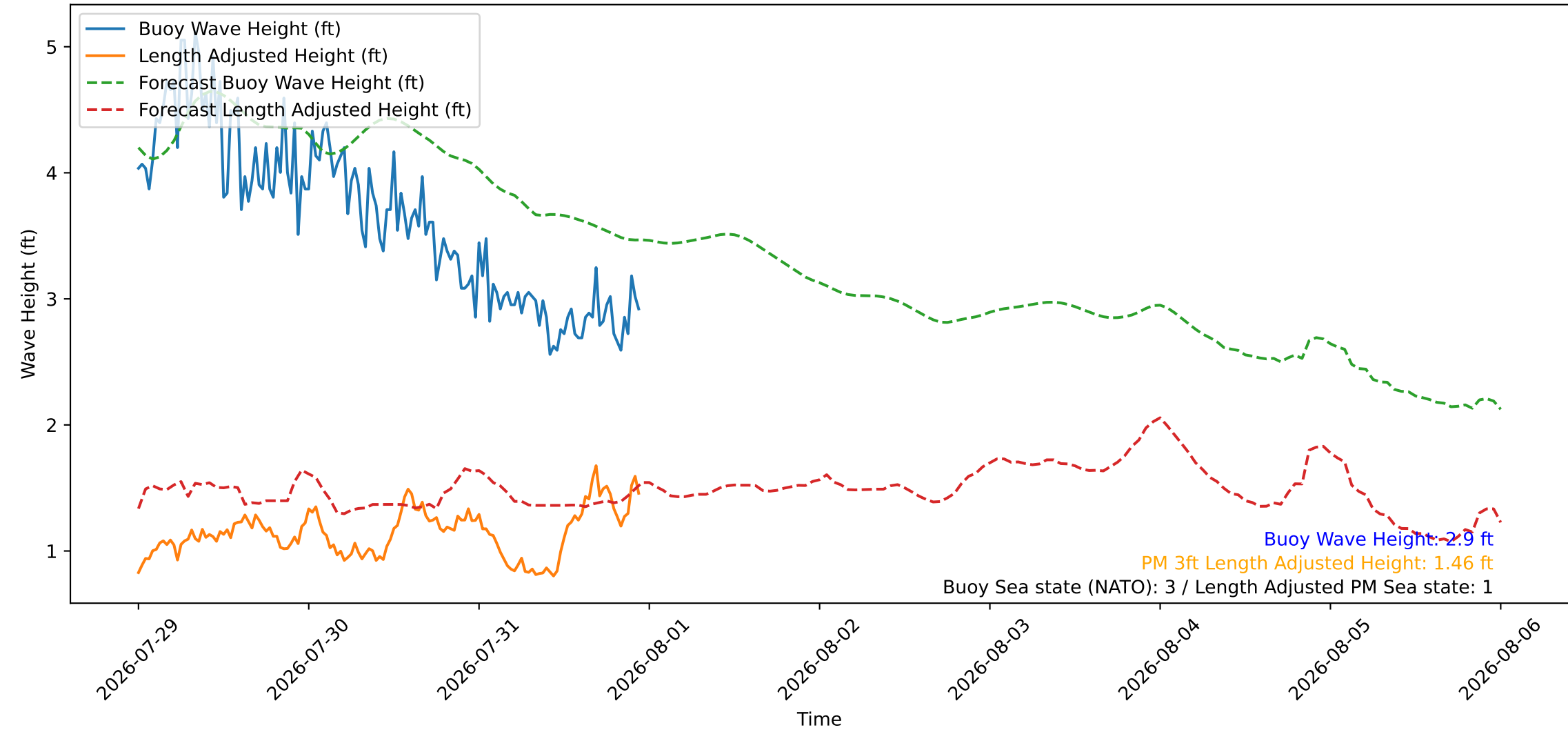
Wave Heights over Time for Red Beach at 2026-07-31 23:30:47
