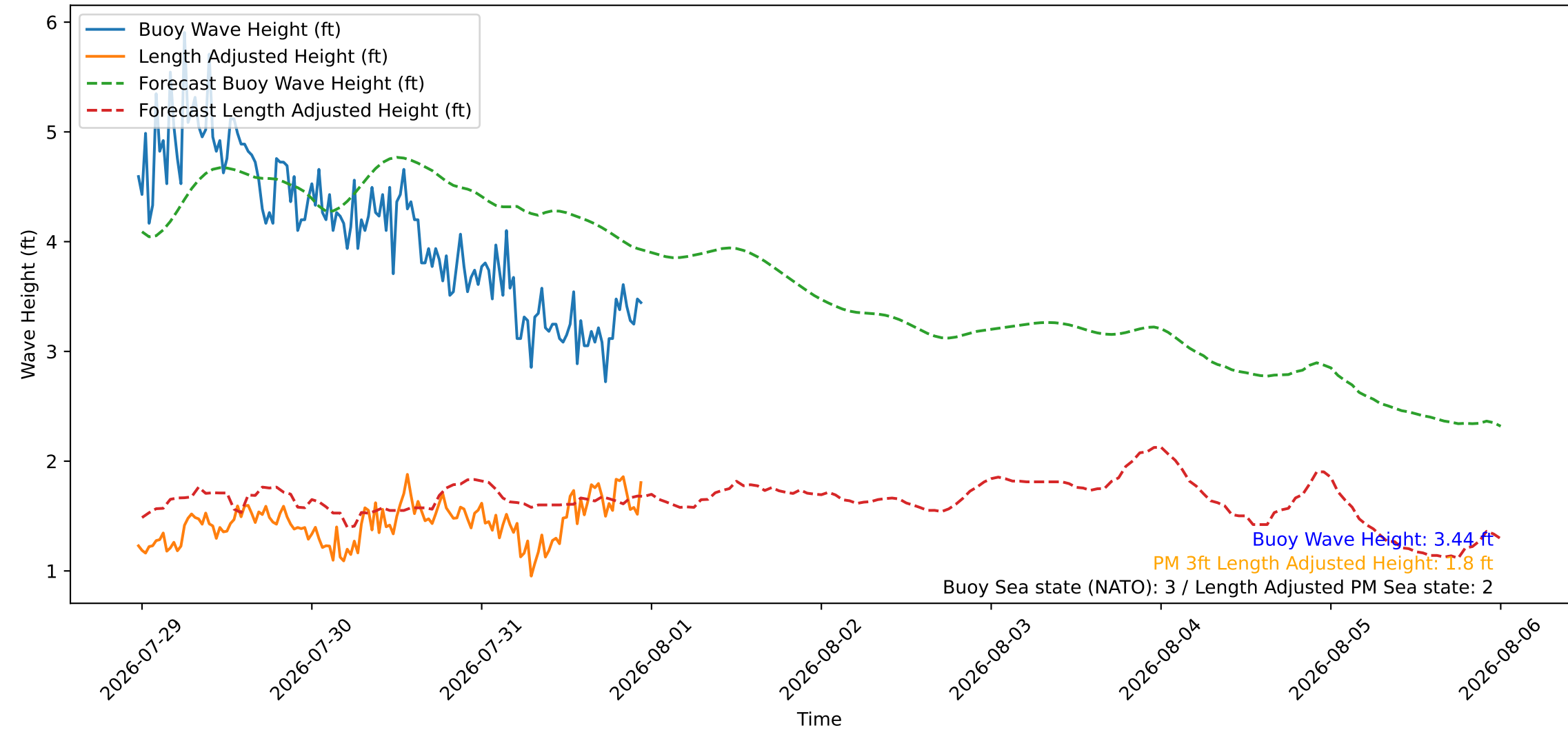
Wave Heights over Time for Oceanside Harbor at 2026-07-31 23:30:27
