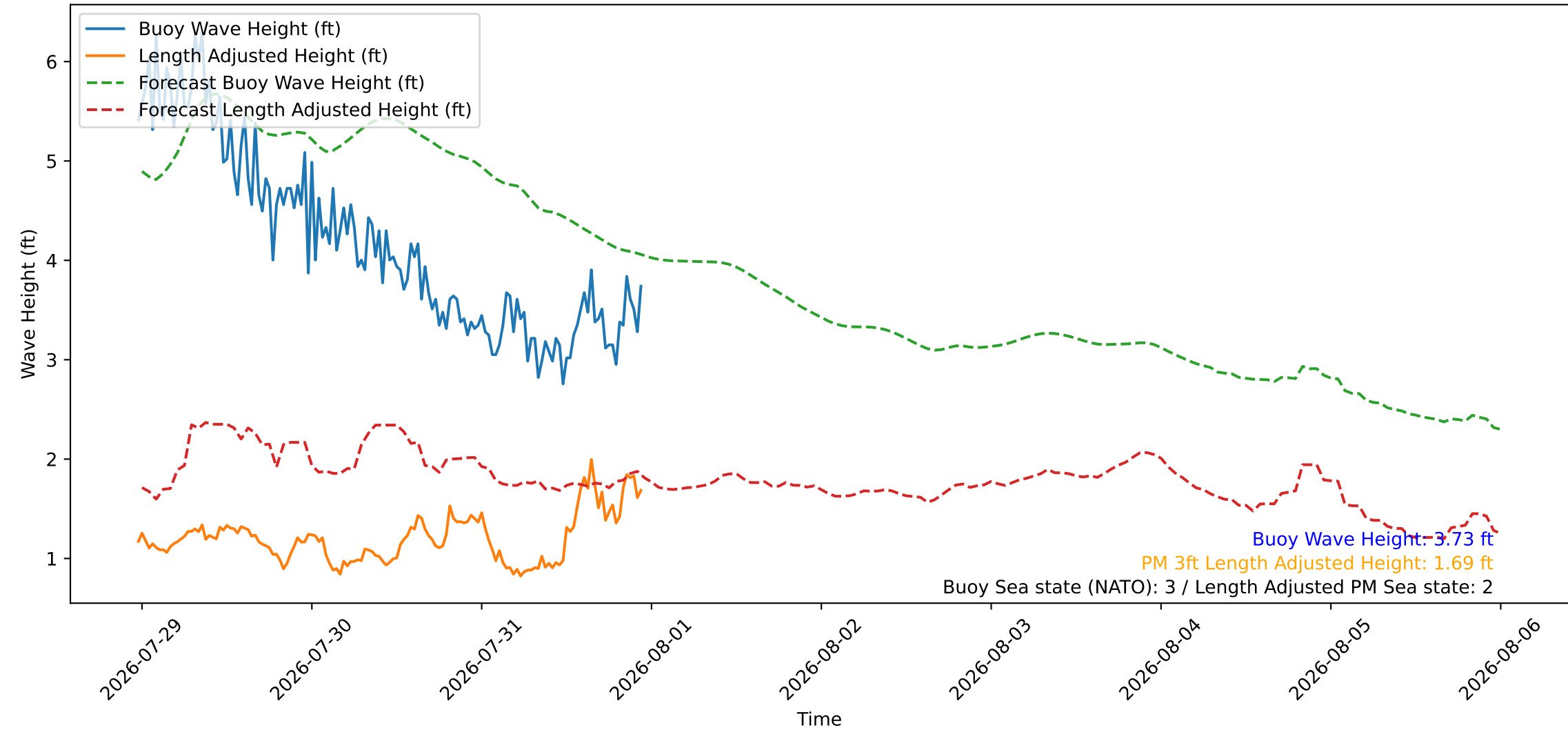
Wave Heights over Time for Green Beach at 2026-07-31 23:31:09
