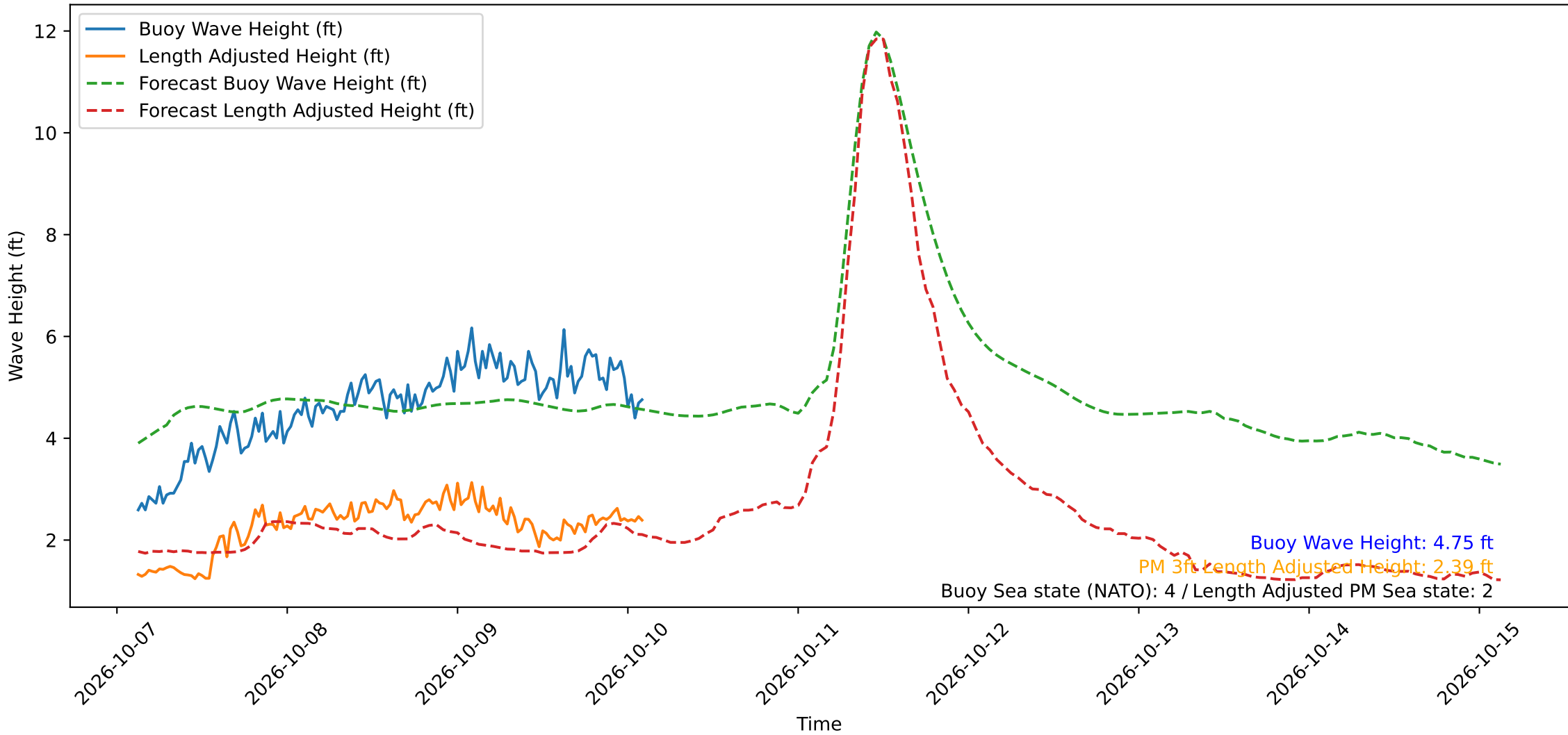
Wave Heights over Time for Green Beach at 2026-10-10 02:41:11
