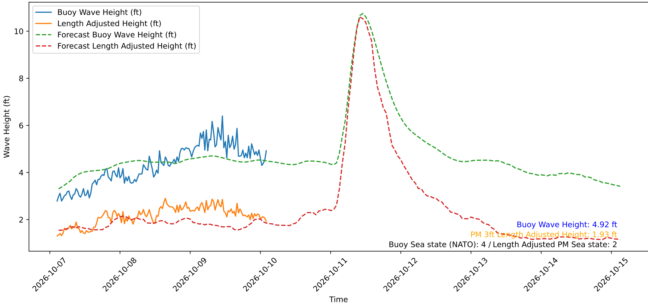
Wave Heights over Time for Oceanside Harbor at 2026-10-10 02:40:29
