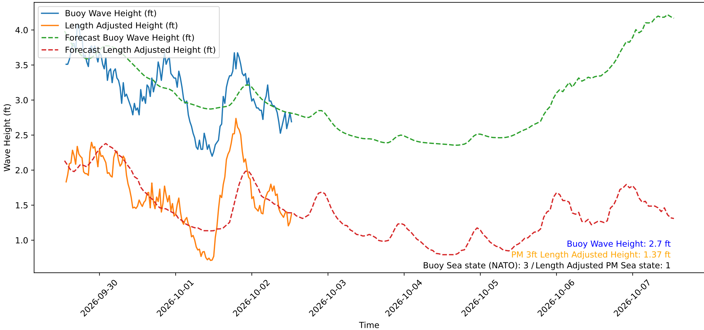
Wave Heights over Time for Green Beach at 2026-10-02 13:11:12
