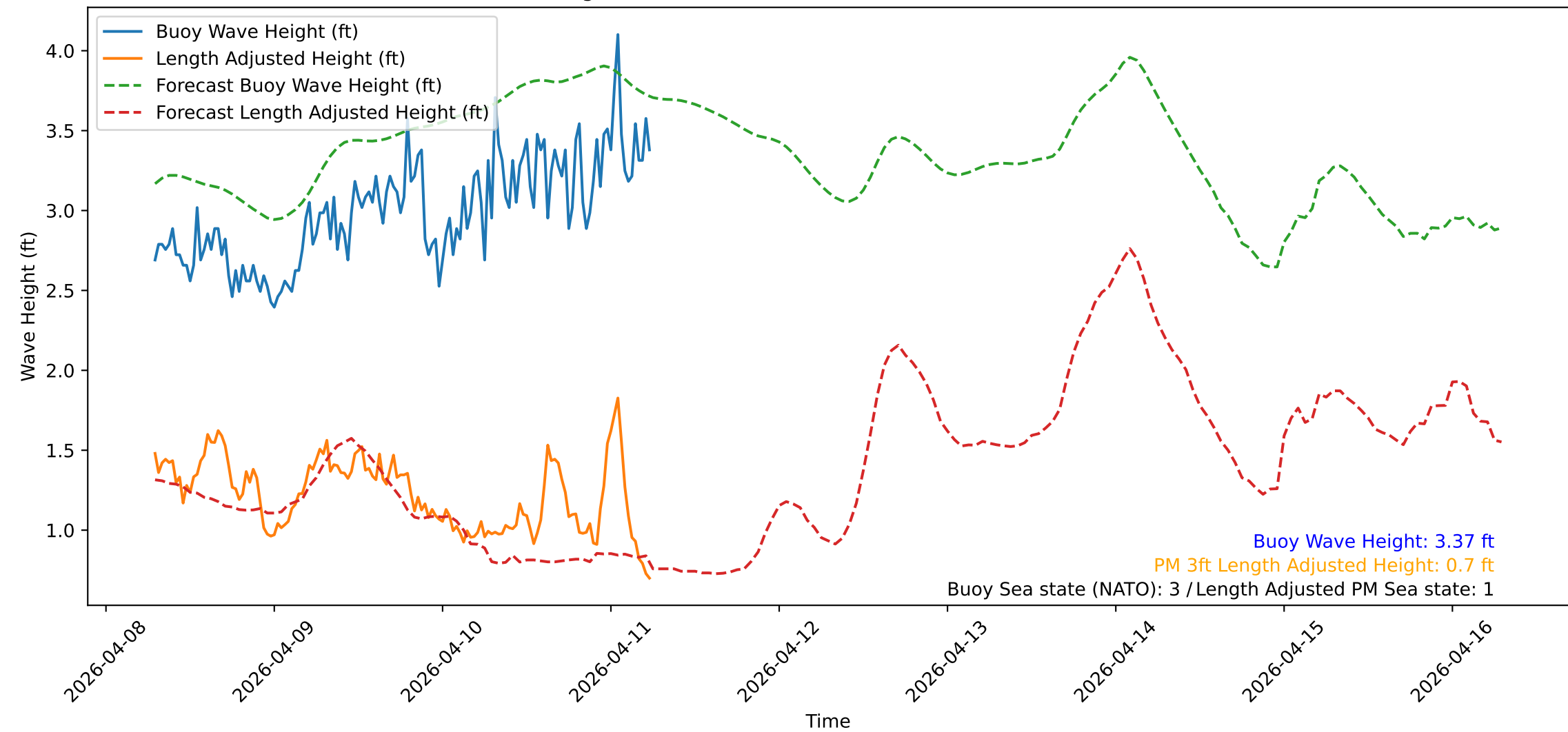
Wave Heights over Time for Red Beach at 2026-04-11 06:40:51
