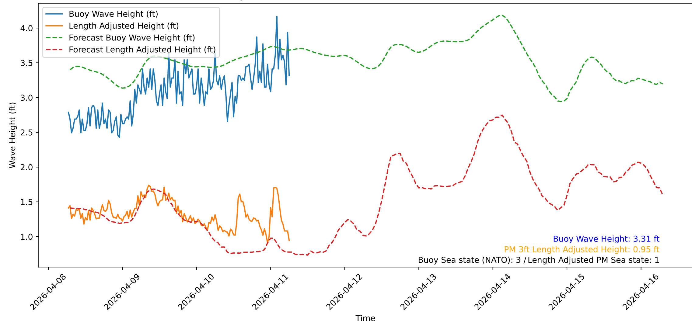
Wave Heights over Time for Oceanside Harbor at 2026-04-11 06:40:32
