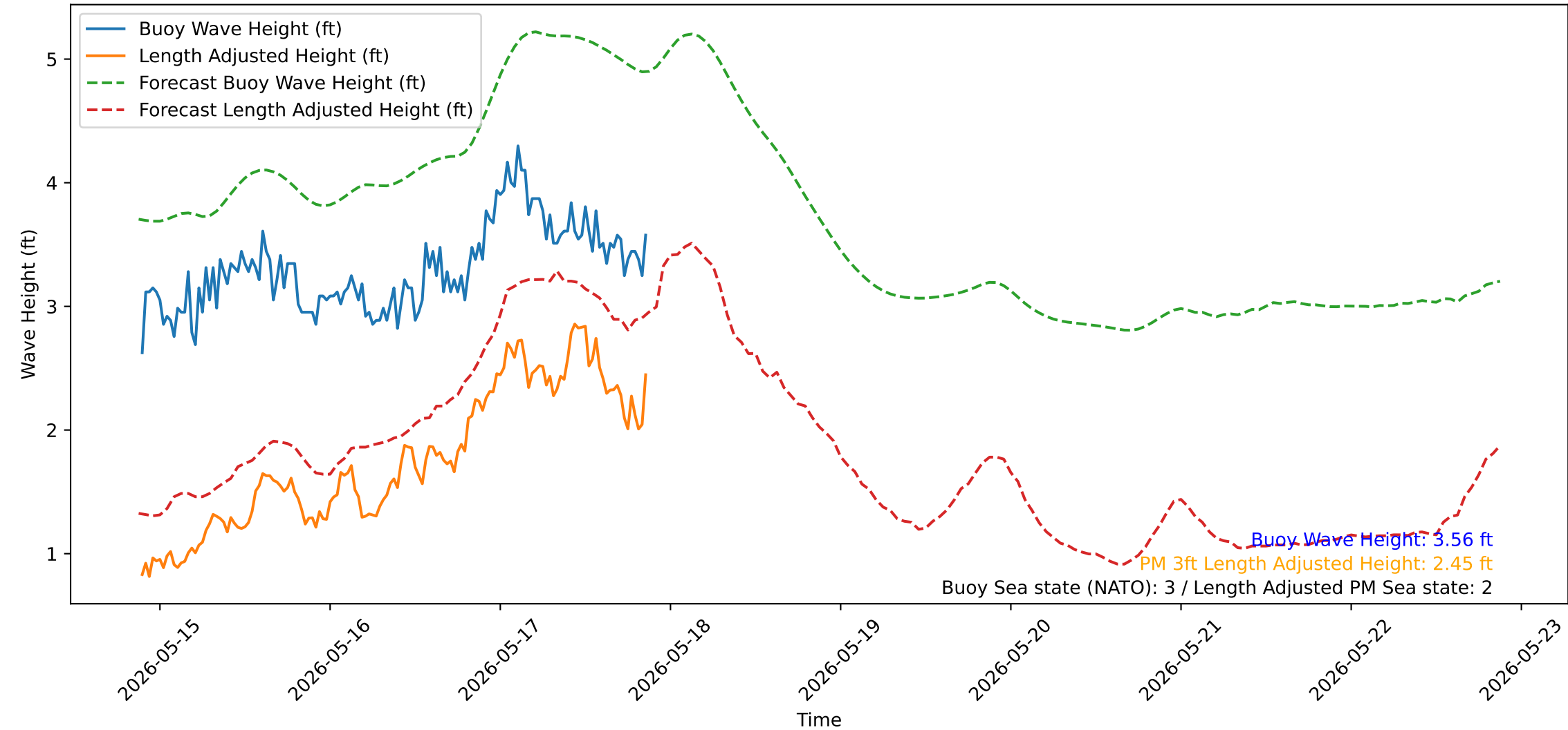
Wave Heights over Time for Oceanside Harbor at 2026-05-17 21:20:32
