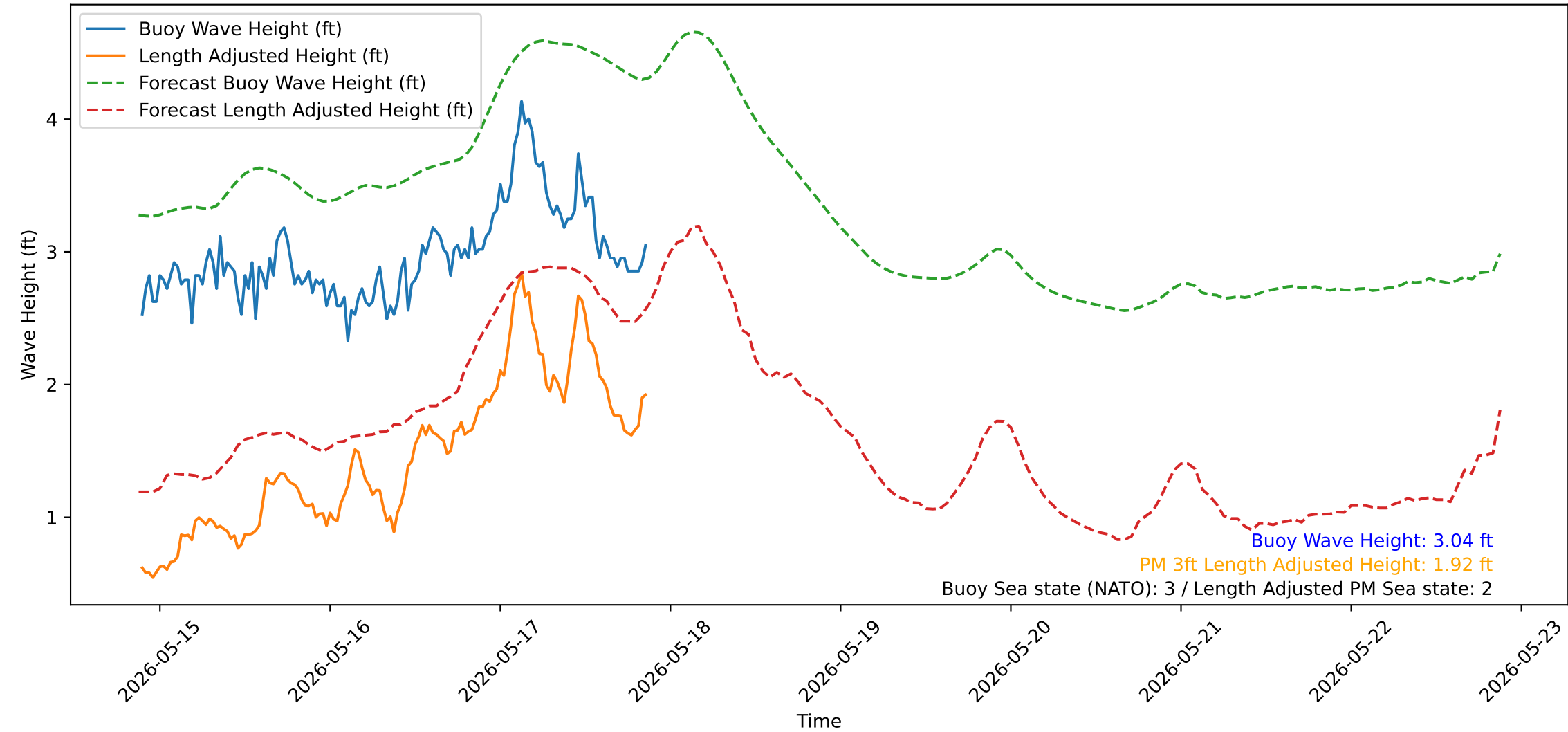
Wave Heights over Time for Red Beach at 2026-05-17 21:20:52
