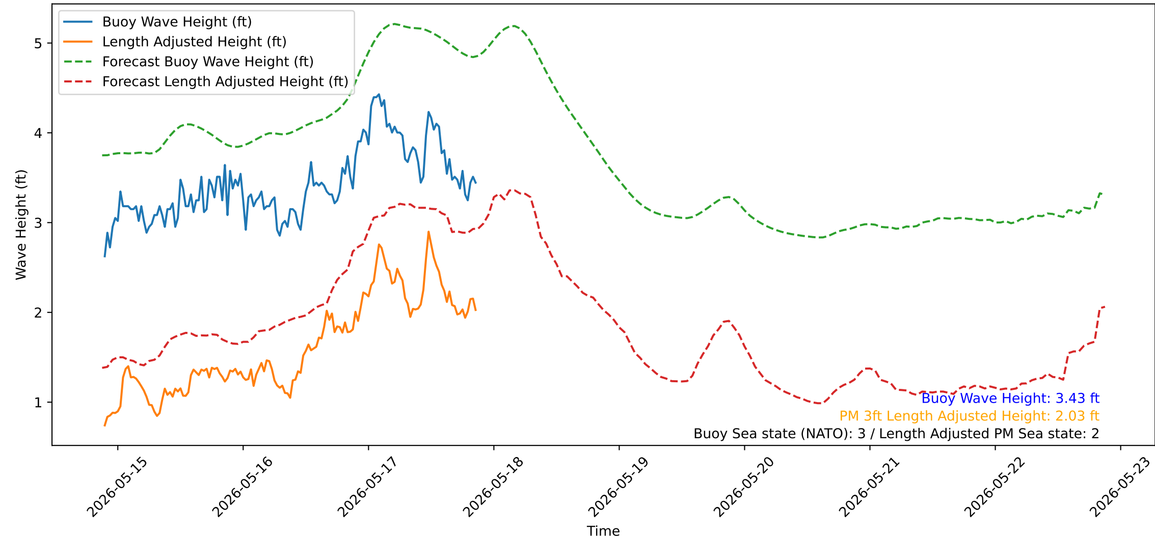
Wave Heights over Time for Green Beach at 2026-05-17 21:21:15
