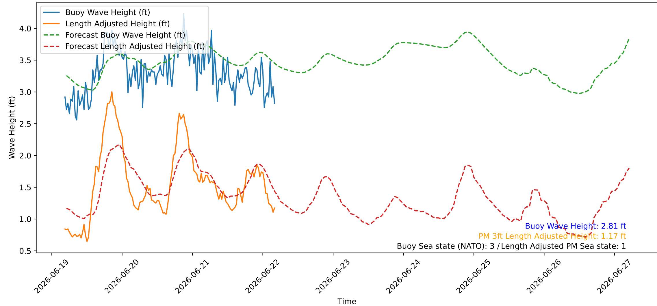
Wave Heights over Time for Green Beach at 2026-06-22 04:41:08
