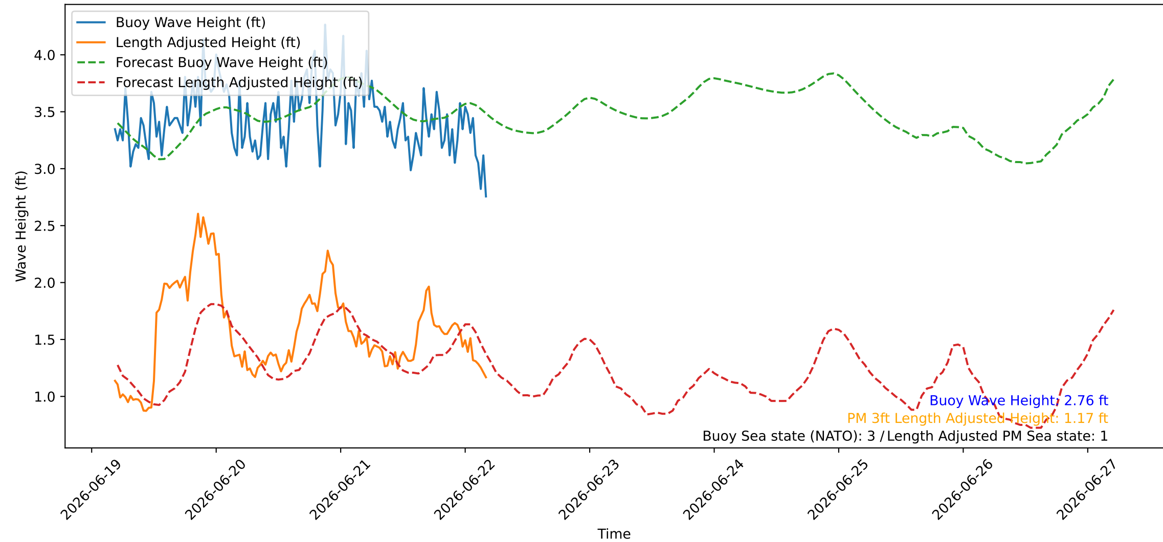
Wave Heights over Time for Oceanside Harbor at 2026-06-22 04:40:26
