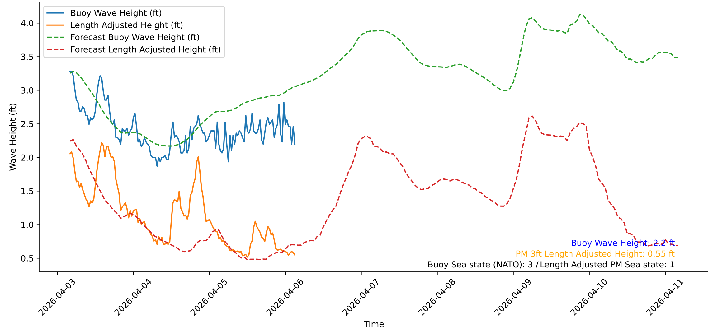
Wave Heights over Time for Red Beach at 2026-04-06 03:40:47
