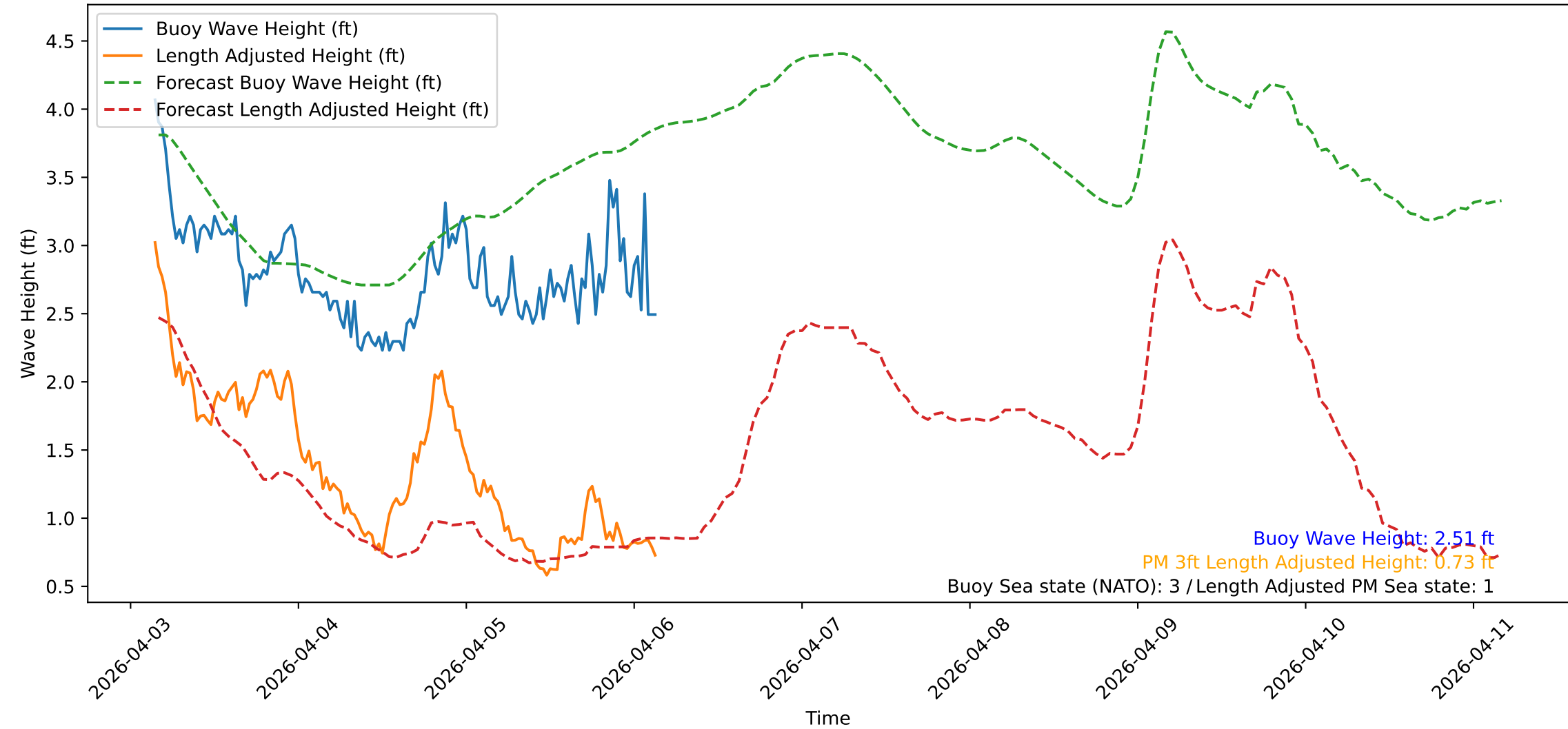
Wave Heights over Time for Green Beach at 2026-04-06 03:41:09
