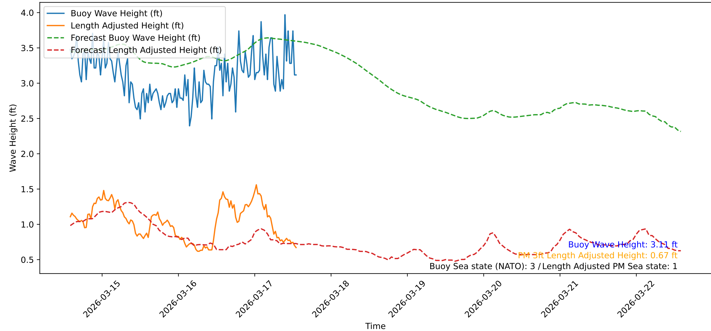
Wave Heights over Time for Oceanside Harbor at 2026-03-17 14:10:43
