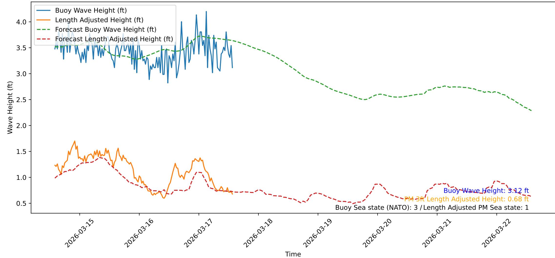
Wave Heights over Time for Green Beach at 2026-03-17 14:11:39
