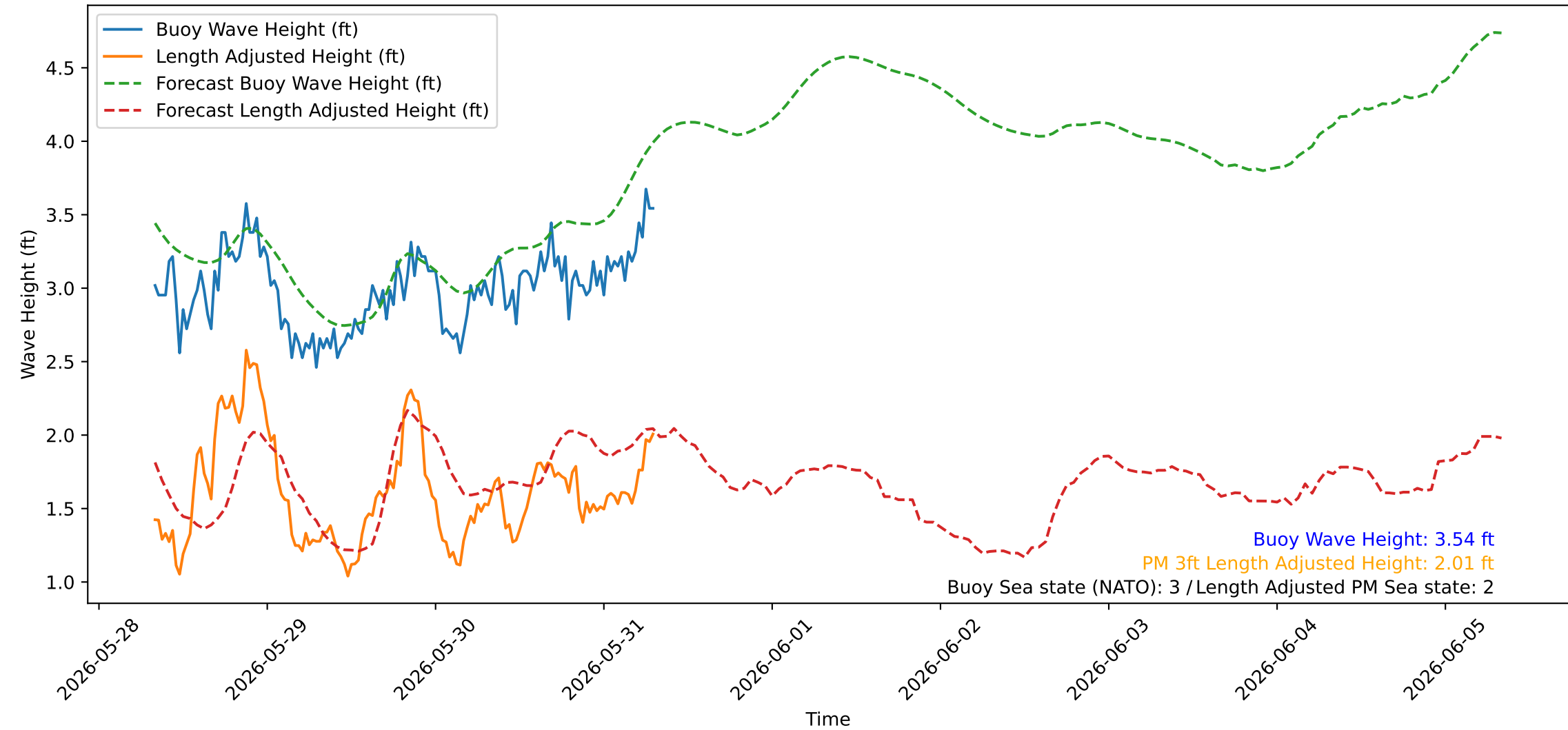
Wave Heights over Time for Green Beach at 2026-05-31 08:01:08
