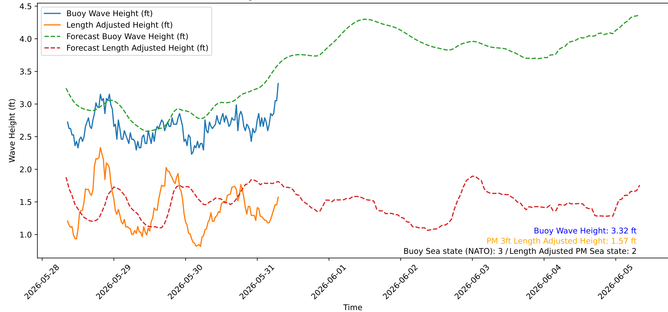
Wave Heights over Time for Red Beach at 2026-05-31 08:00:45
