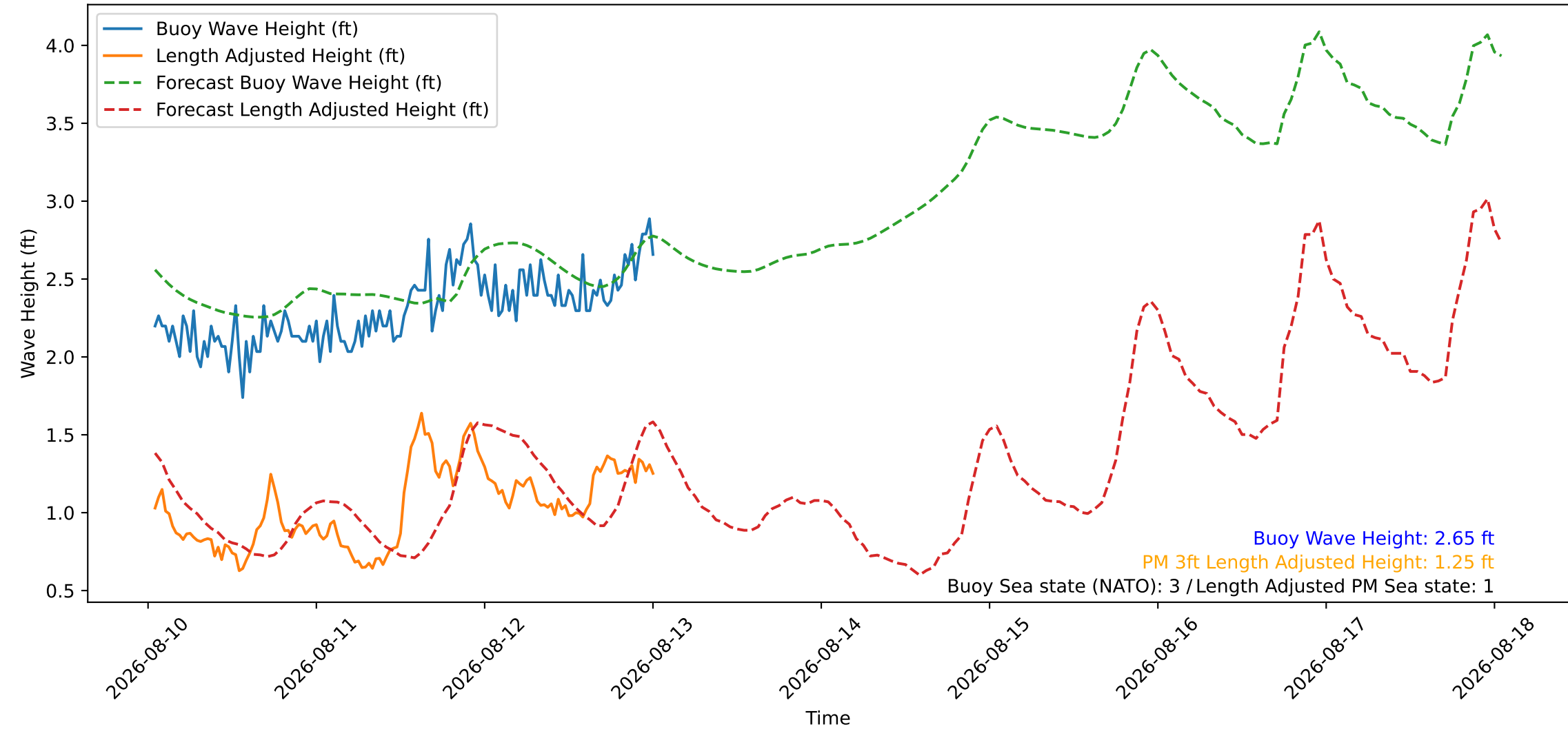
Wave Heights over Time for Red Beach at 2026-08-13 00:50:47
