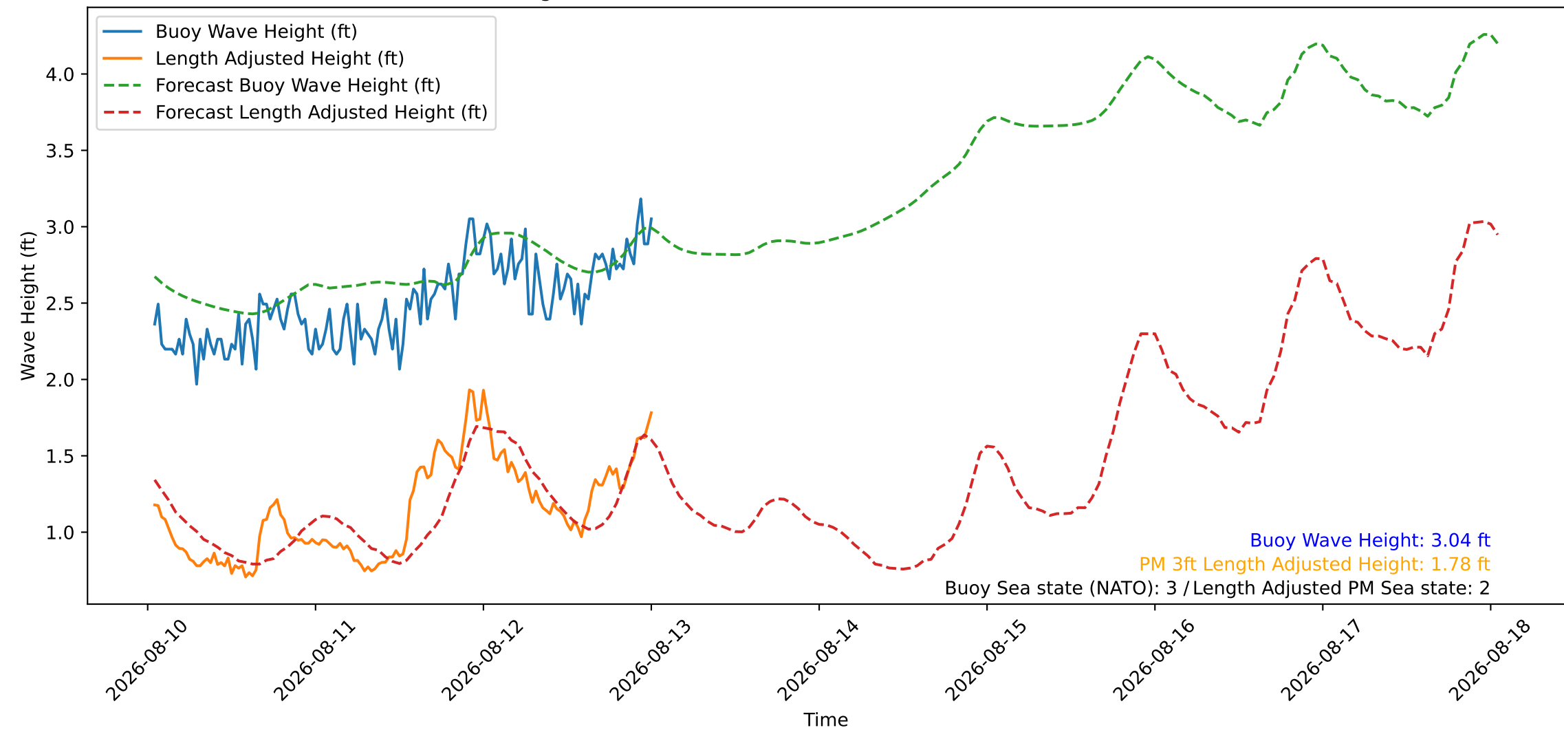
Wave Heights over Time for Oceanside Harbor at 2026-08-13 00:50:26
