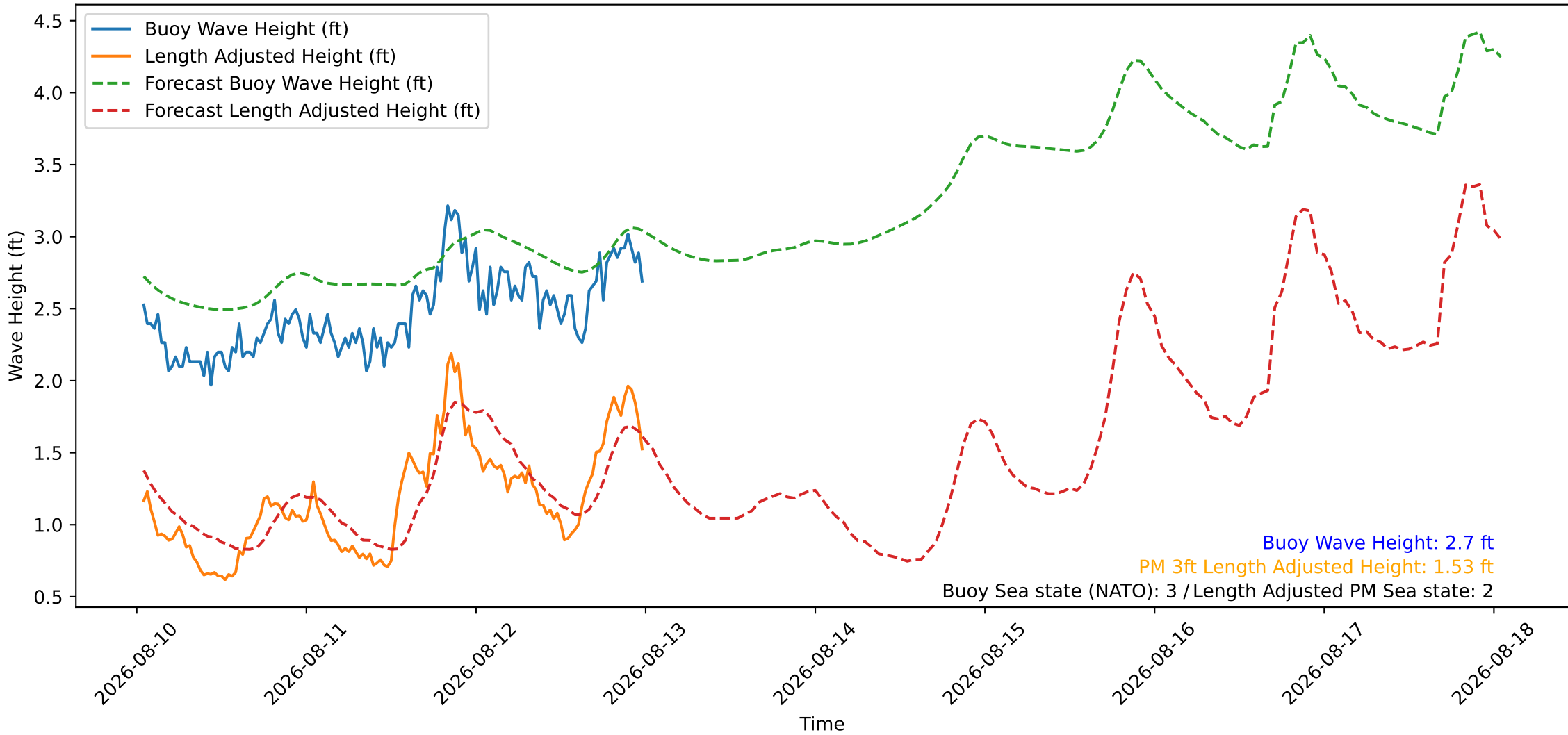
Wave Heights over Time for Green Beach at 2026-08-13 00:51:09
