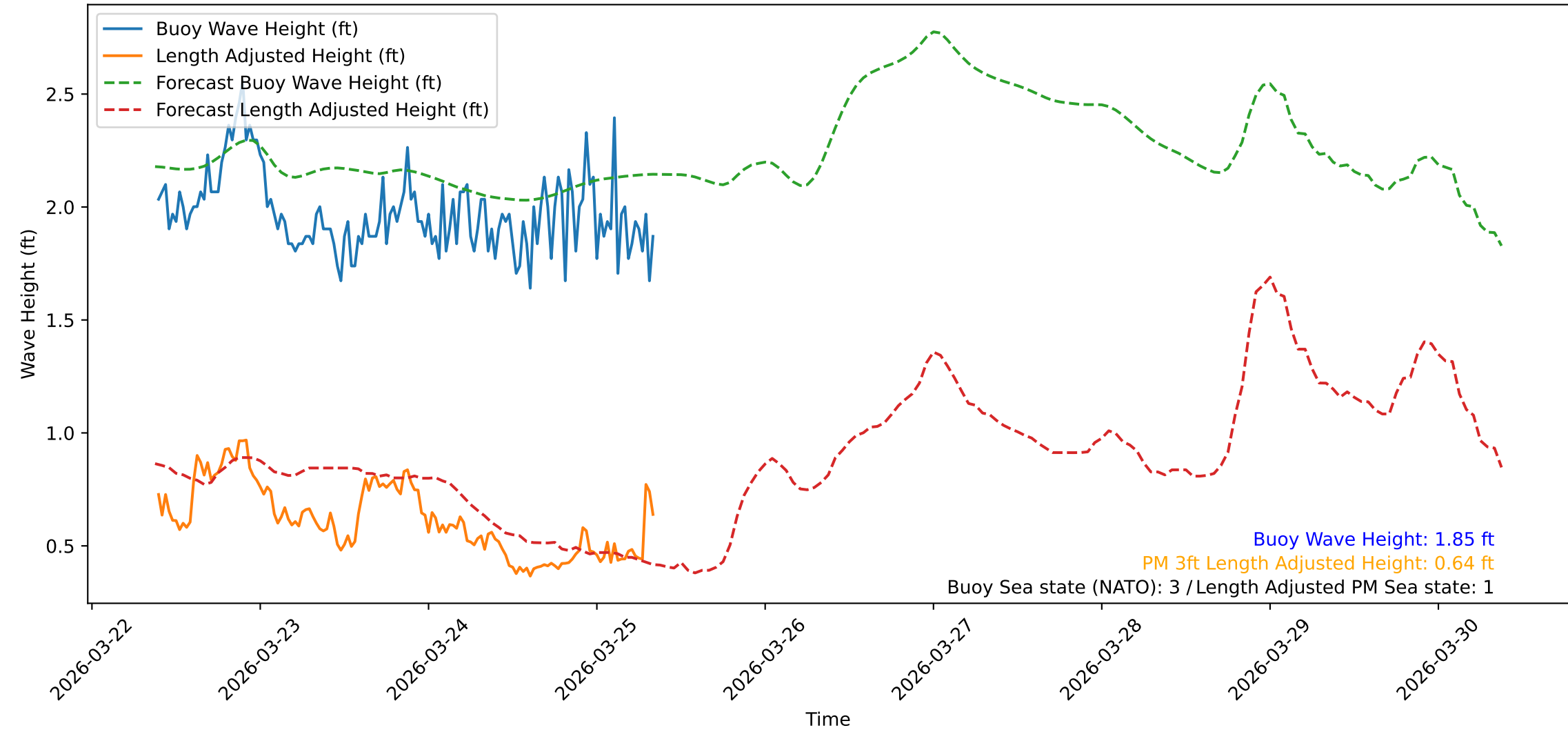
Wave Heights over Time for Red Beach at 2026-03-25 09:00:47
