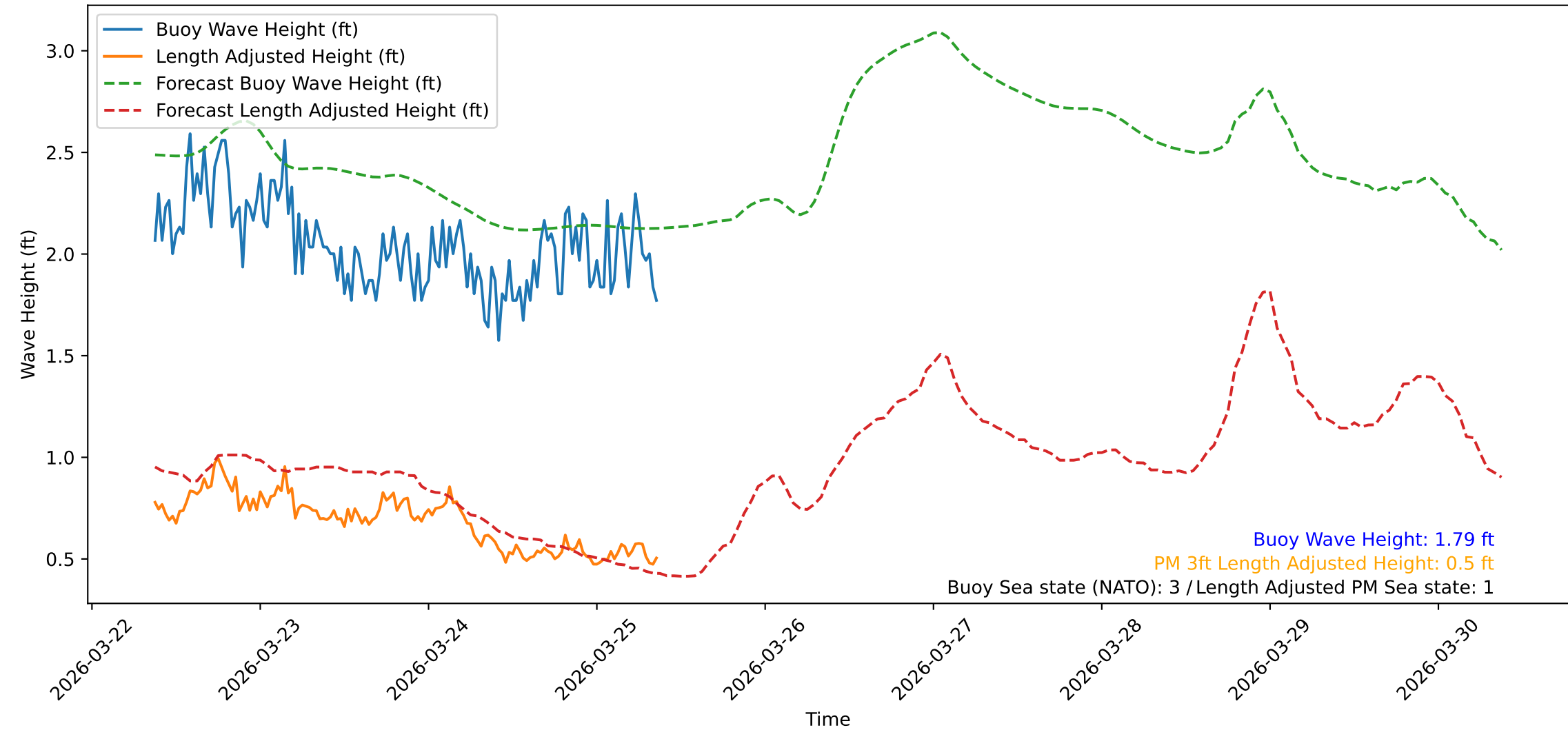
Wave Heights over Time for Oceanside Harbor at 2026-03-25 09:00:31
