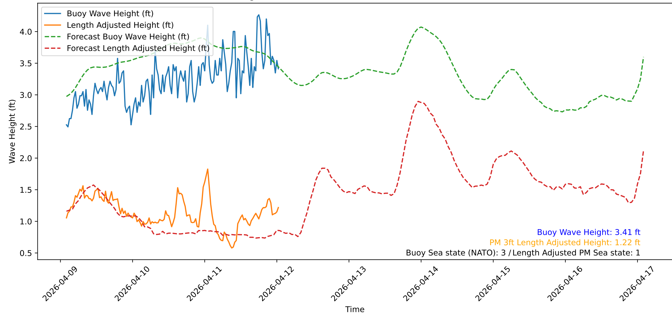
Wave Heights over Time for Red Beach at 2026-04-12 01:30:52
