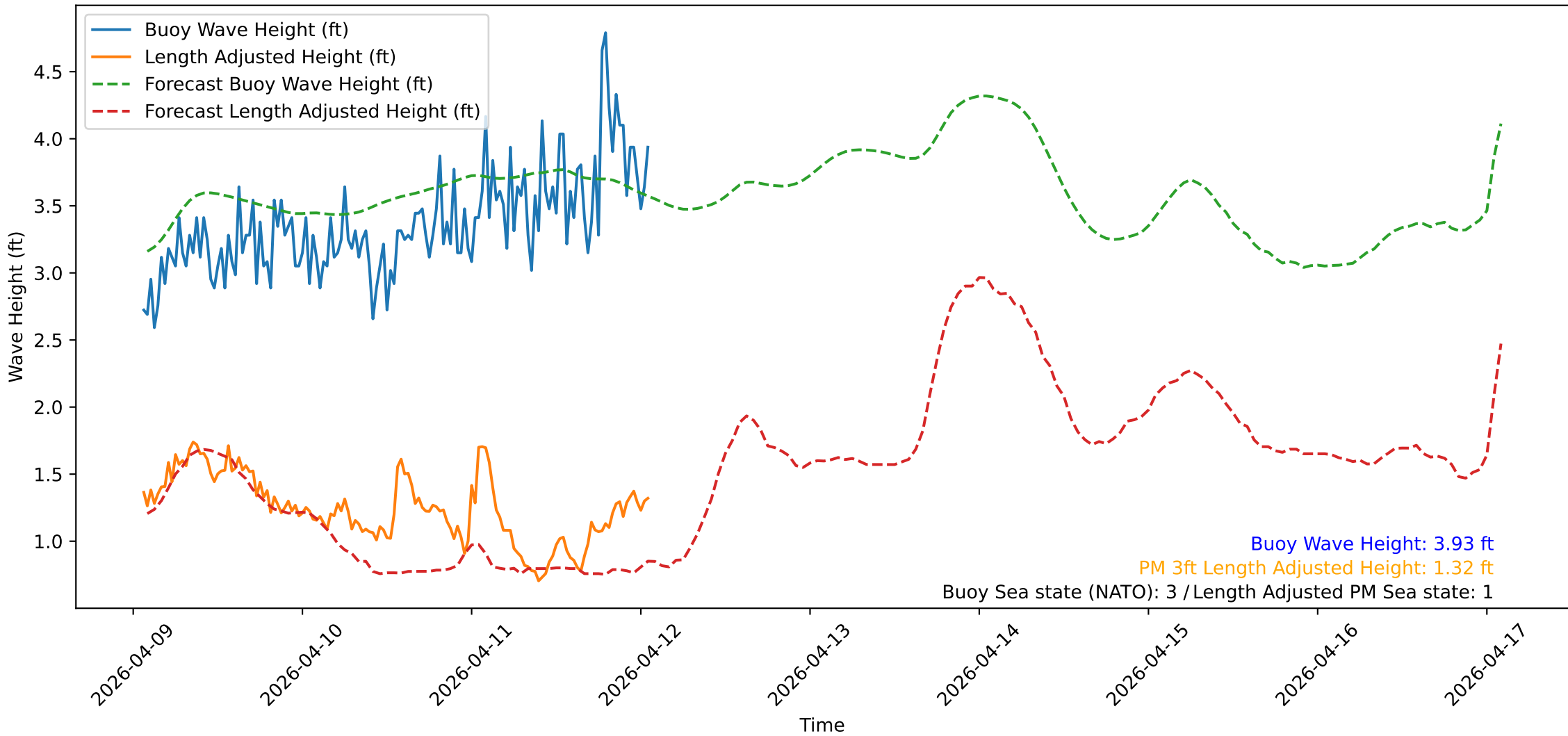
Wave Heights over Time for Oceanside Harbor at 2026-04-12 01:30:32
