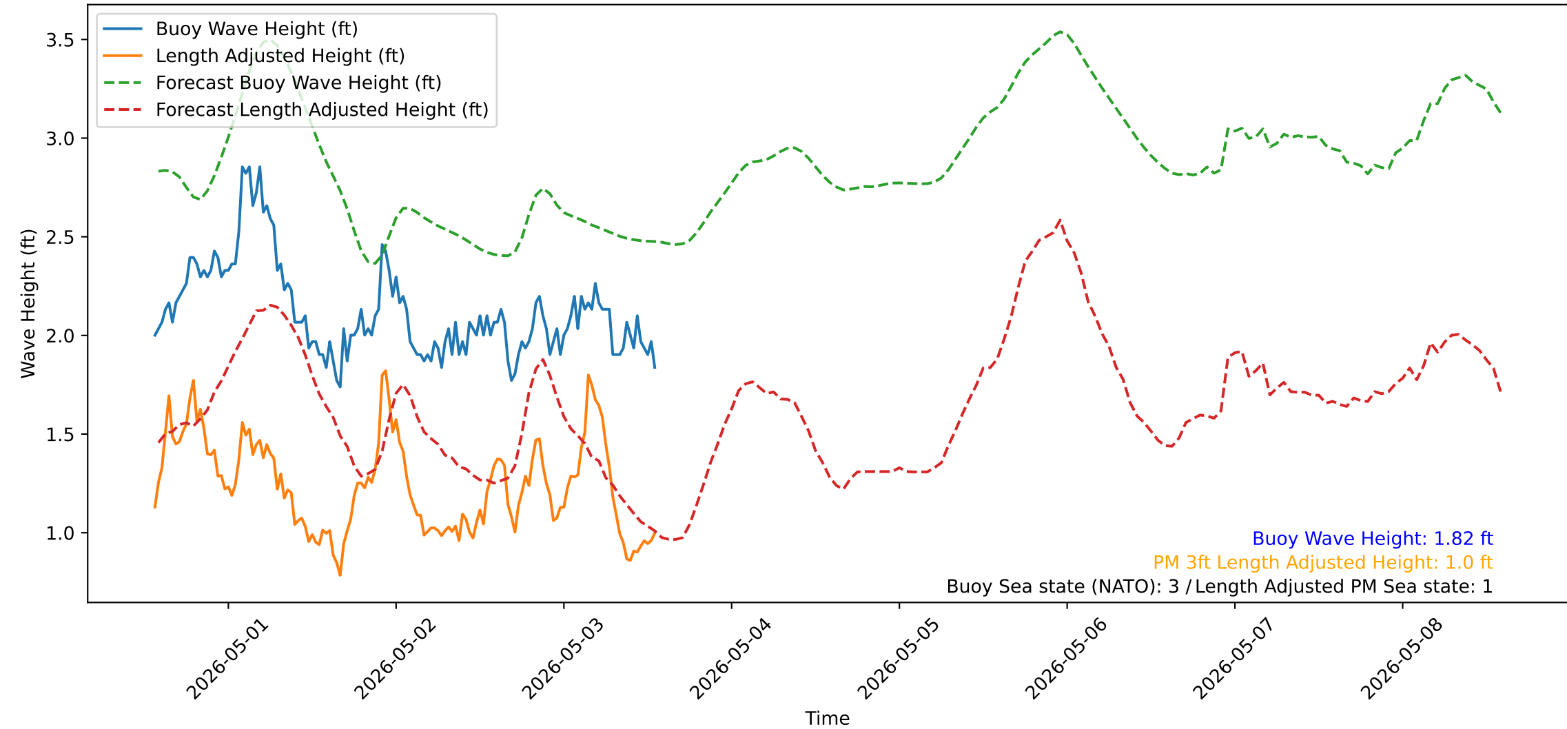
Wave Heights over Time for Green Beach at 2026-05-03 13:41:13
