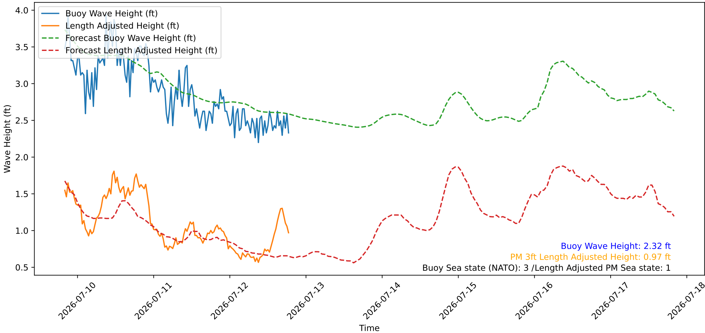
Wave Heights over Time for Red Beach at 2026-07-12 19:30:47
