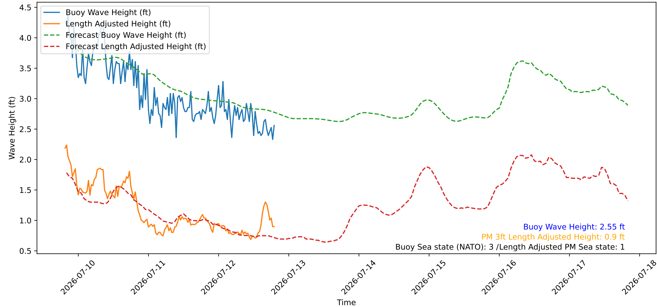
Wave Heights over Time for Oceanside Harbor at 2026-07-12 19:30:27
