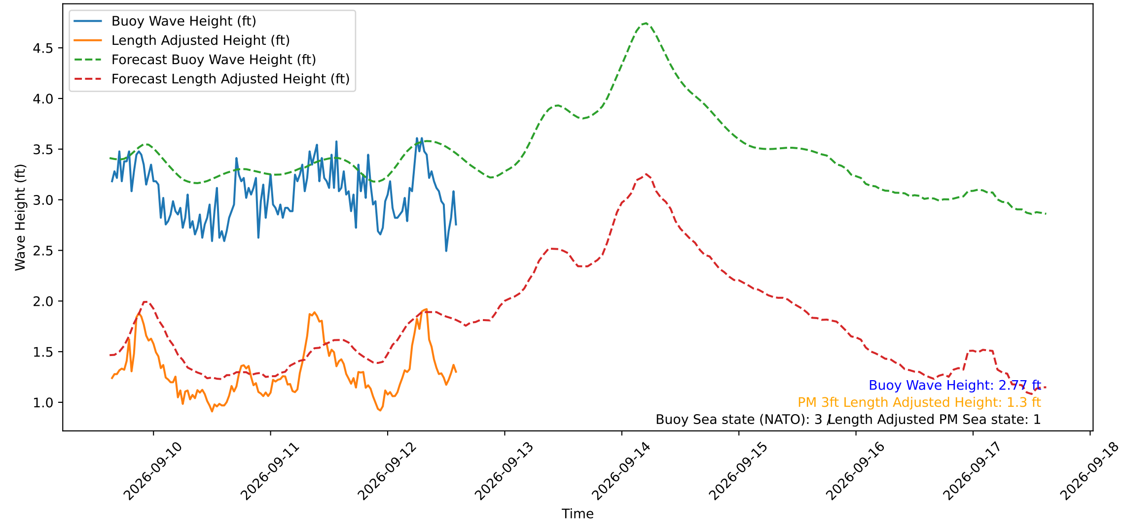
Wave Heights over Time for Green Beach at 2026-09-12 15:01:12
