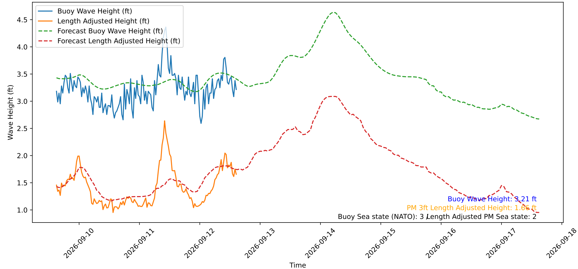
Wave Heights over Time for Oceanside Harbor at 2026-09-12 15:00:30
