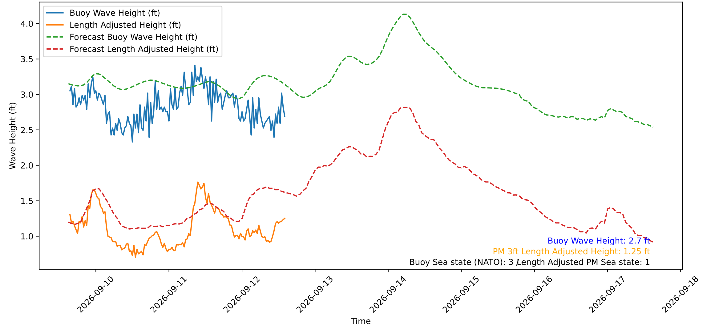
Wave Heights over Time for Red Beach at 2026-09-12 15:00:50
