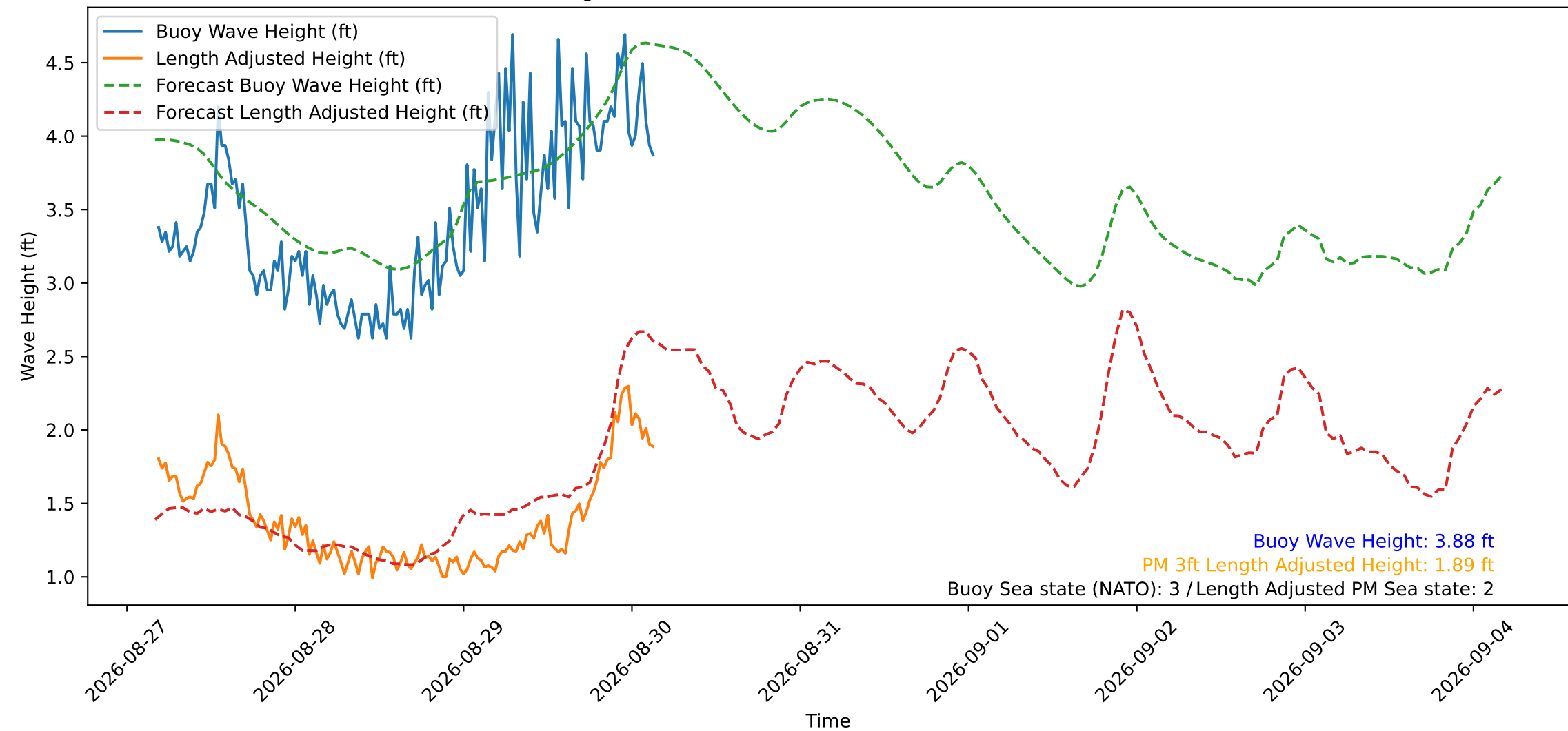
Wave Heights over Time for Red Beach at 2026-08-30 04:00:49
