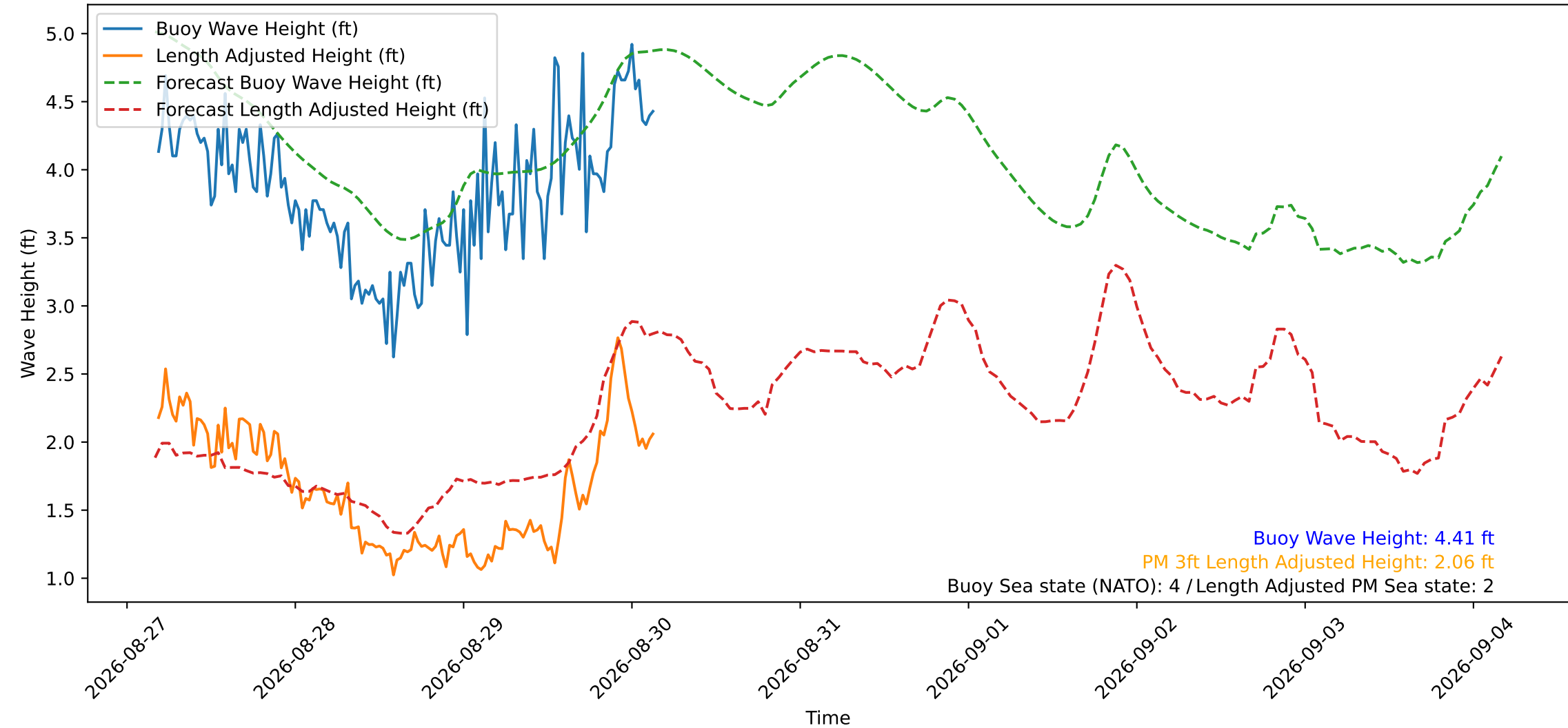
Wave Heights over Time for Green Beach at 2026-08-30 04:01:12
