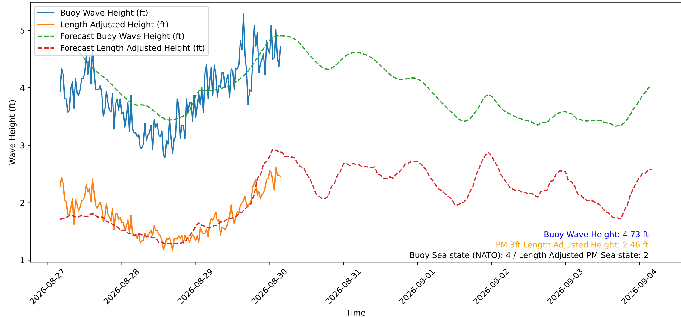
Wave Heights over Time for Oceanside Harbor at 2026-08-30 04:00:30
