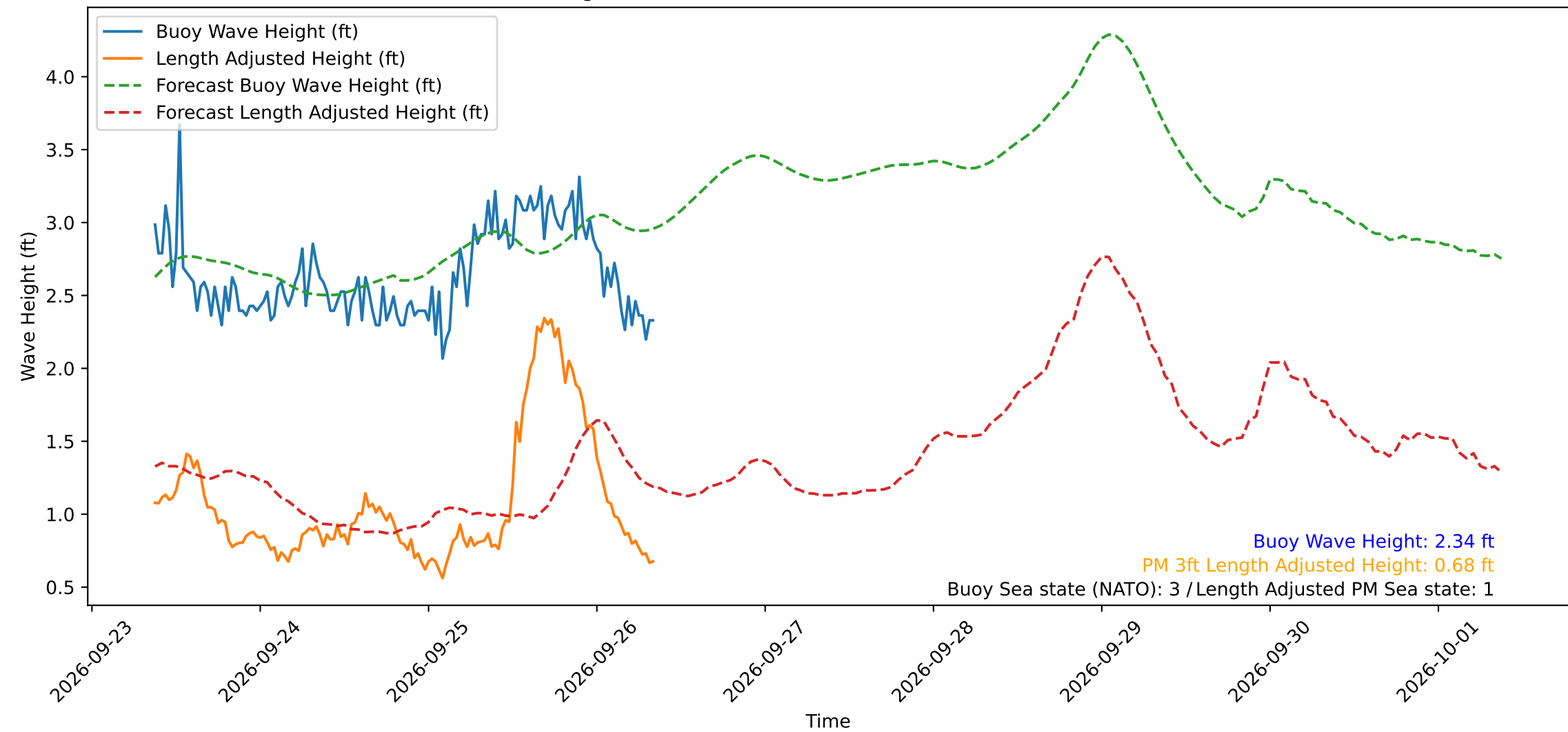
Wave Heights over Time for Red Beach at 2026-09-26 08:50:50
