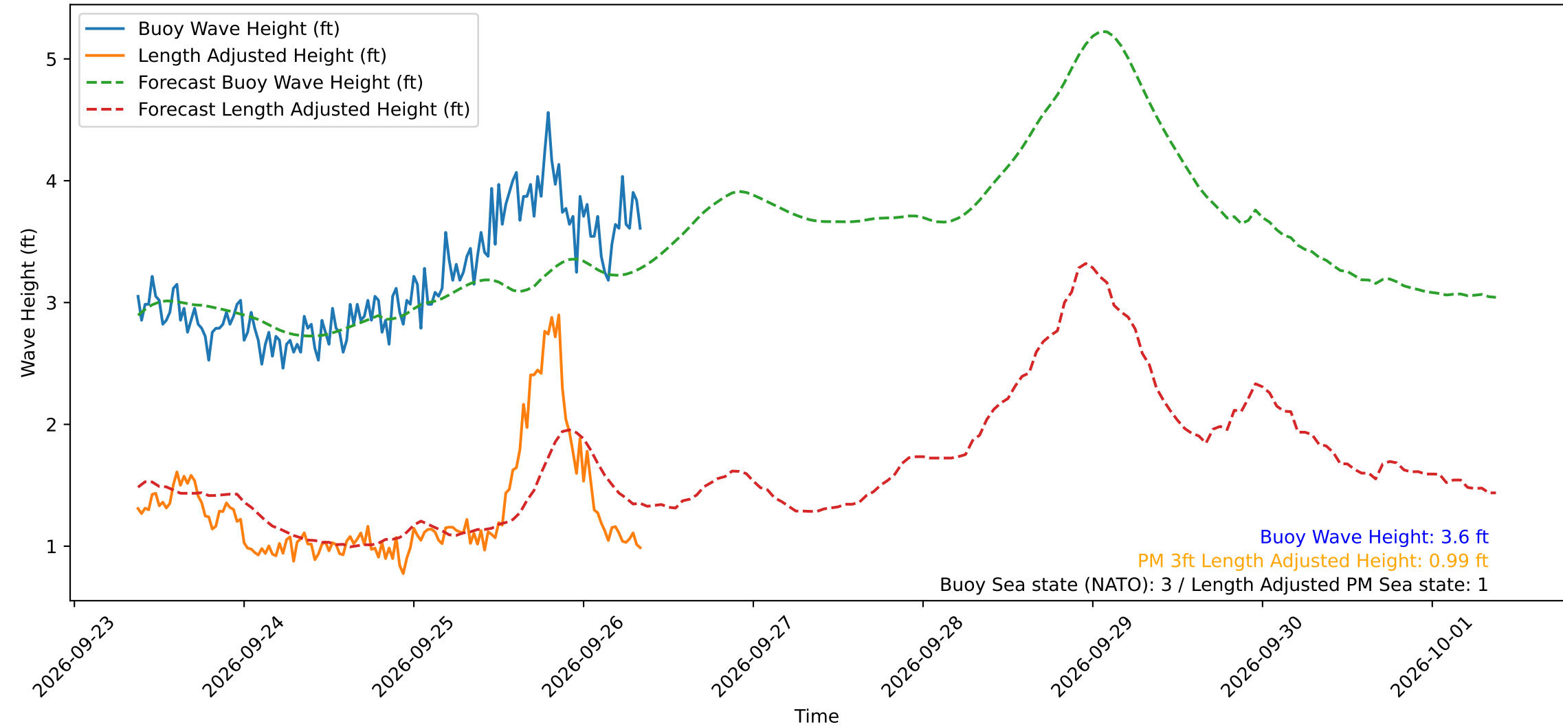
Wave Heights over Time for Green Beach at 2026-09-26 08:51:14
