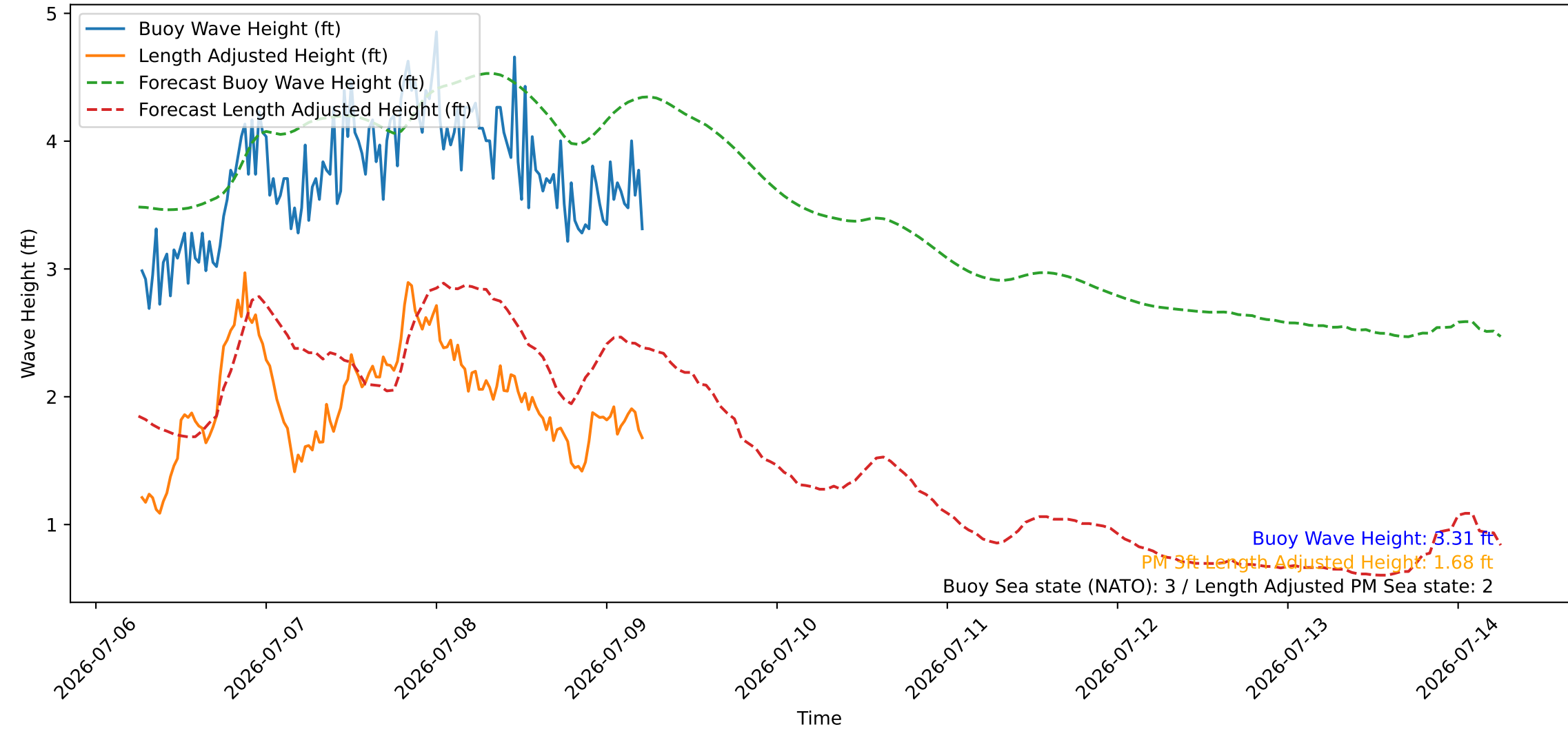
Wave Heights over Time for Red Beach at 2026-07-09 06:00:45
