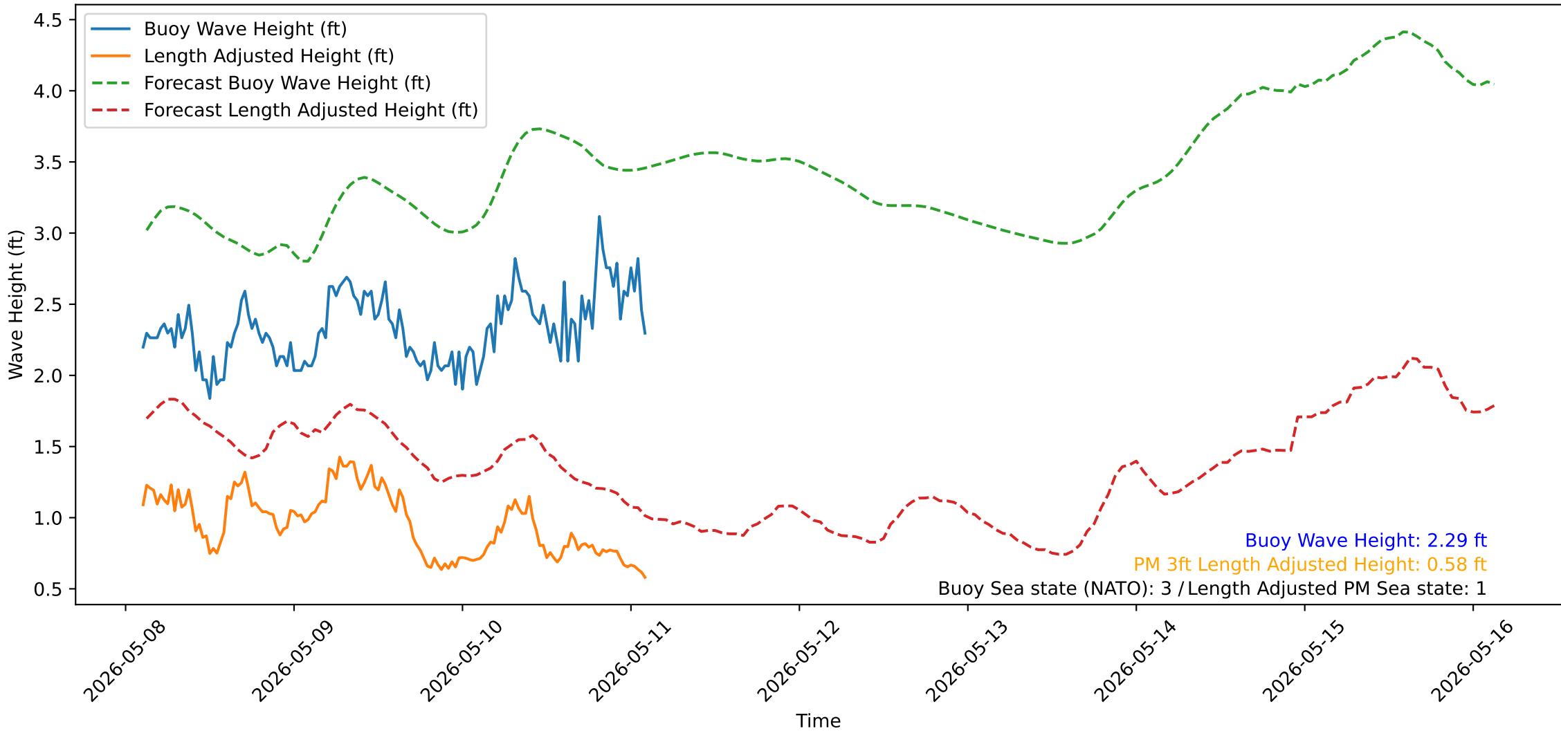
Wave Heights over Time for Green Beach at 2026-05-11 02:41:12
