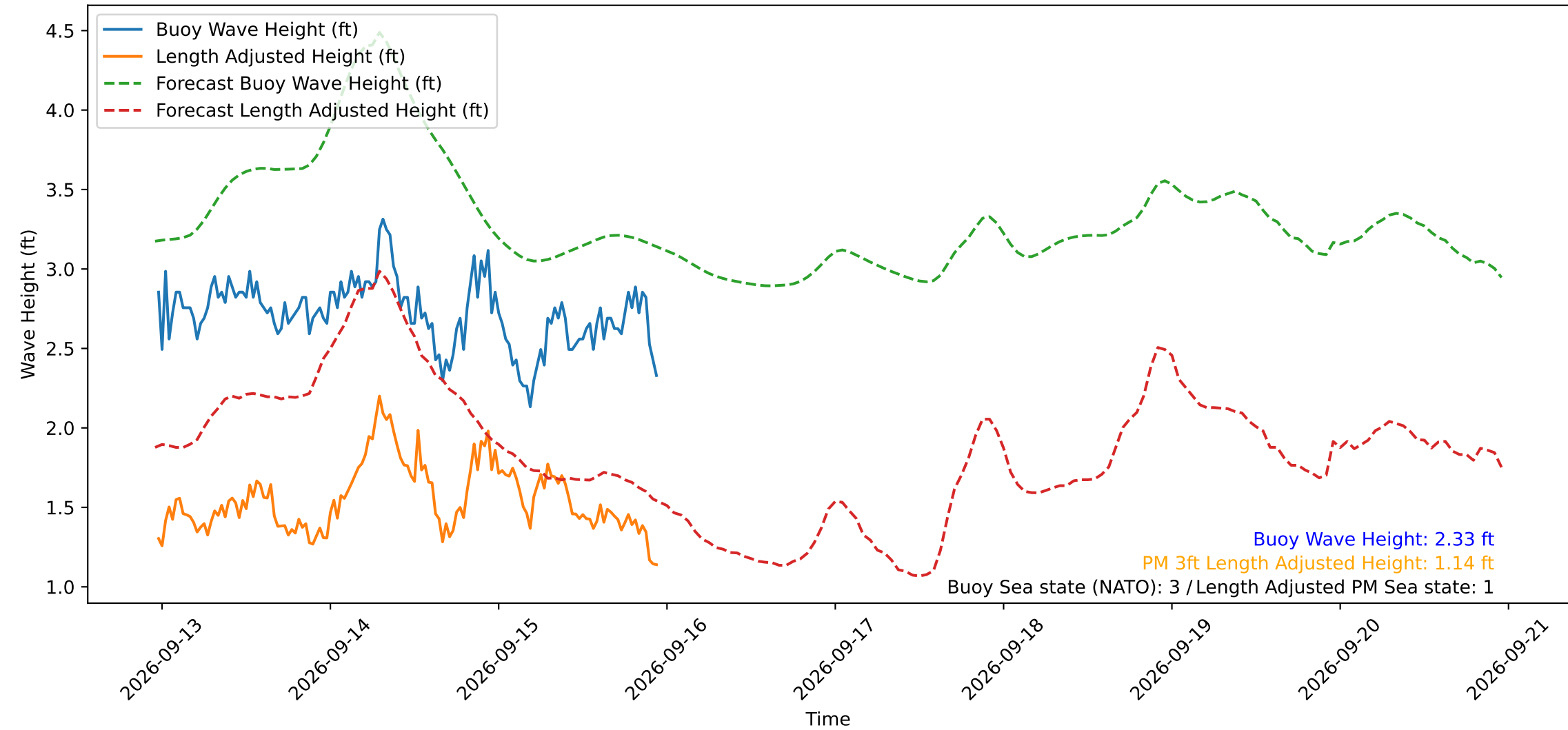
Wave Heights over Time for Green Beach at 2026-09-15 23:11:11
