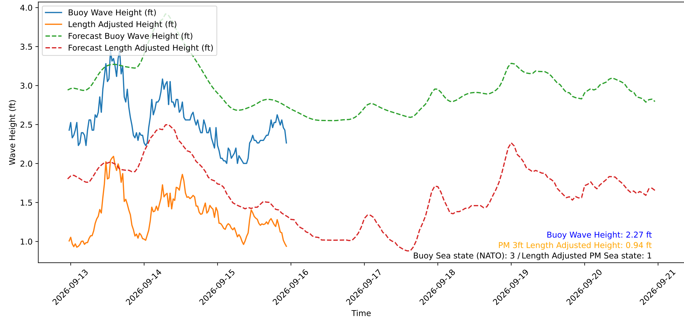
Wave Heights over Time for Red Beach at 2026-09-15 23:10:49
