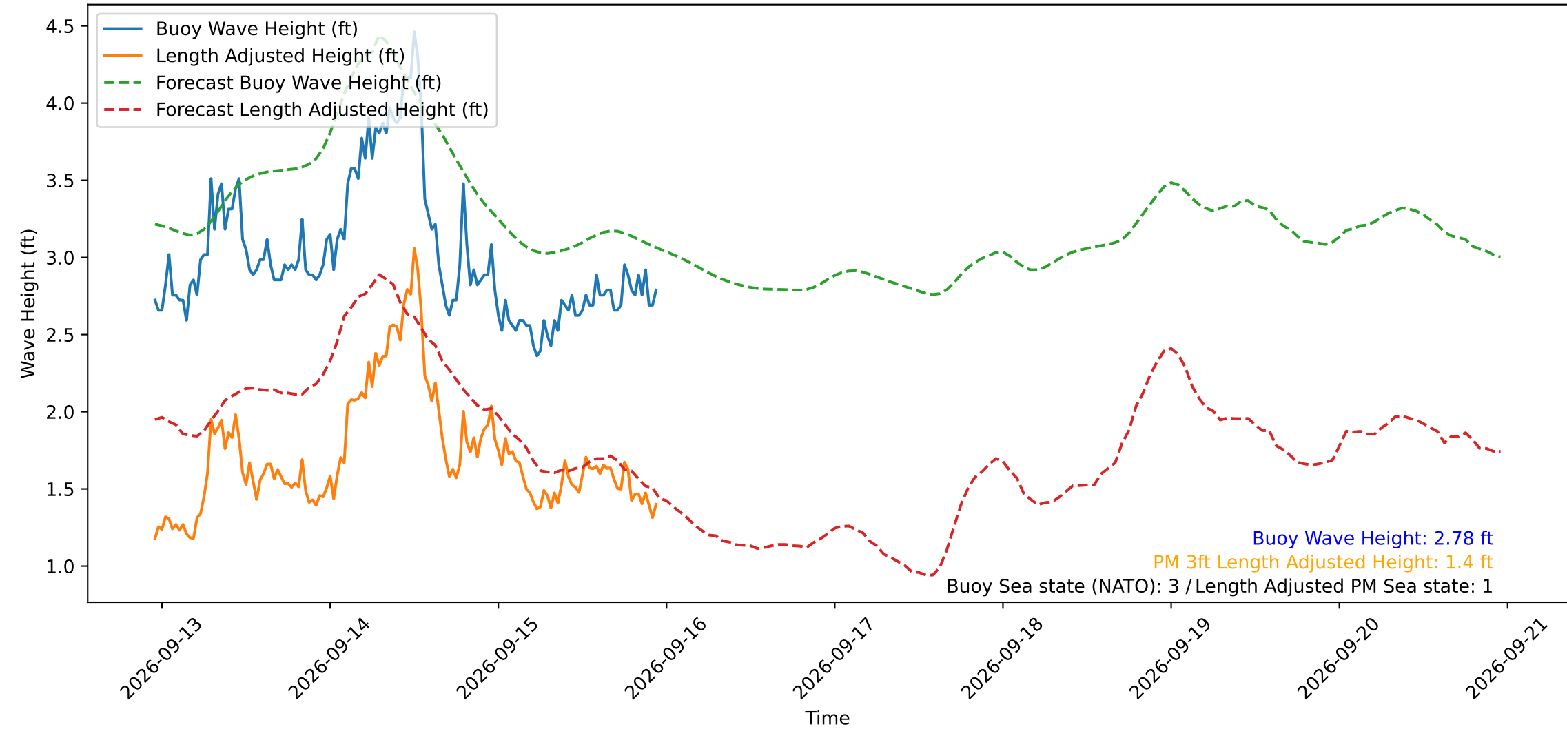
Wave Heights over Time for Oceanside Harbor at 2026-09-15 23:10:30
