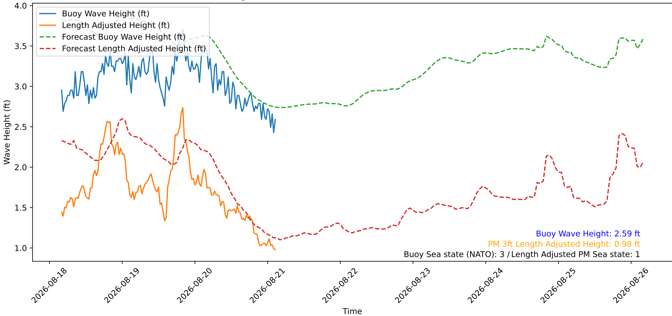
Wave Heights over Time for Green Beach at 2026-08-21 03:31:07
