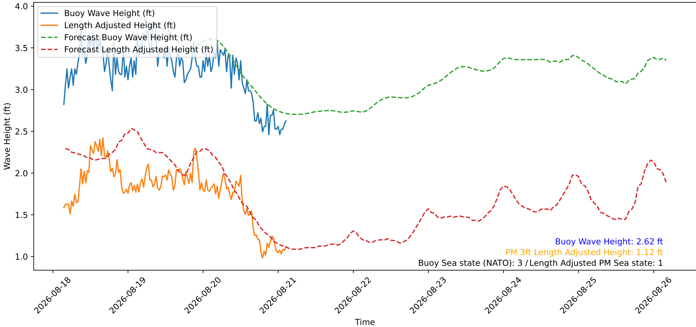
Wave Heights over Time for Oceanside Harbor at 2026-08-21 03:30:26
