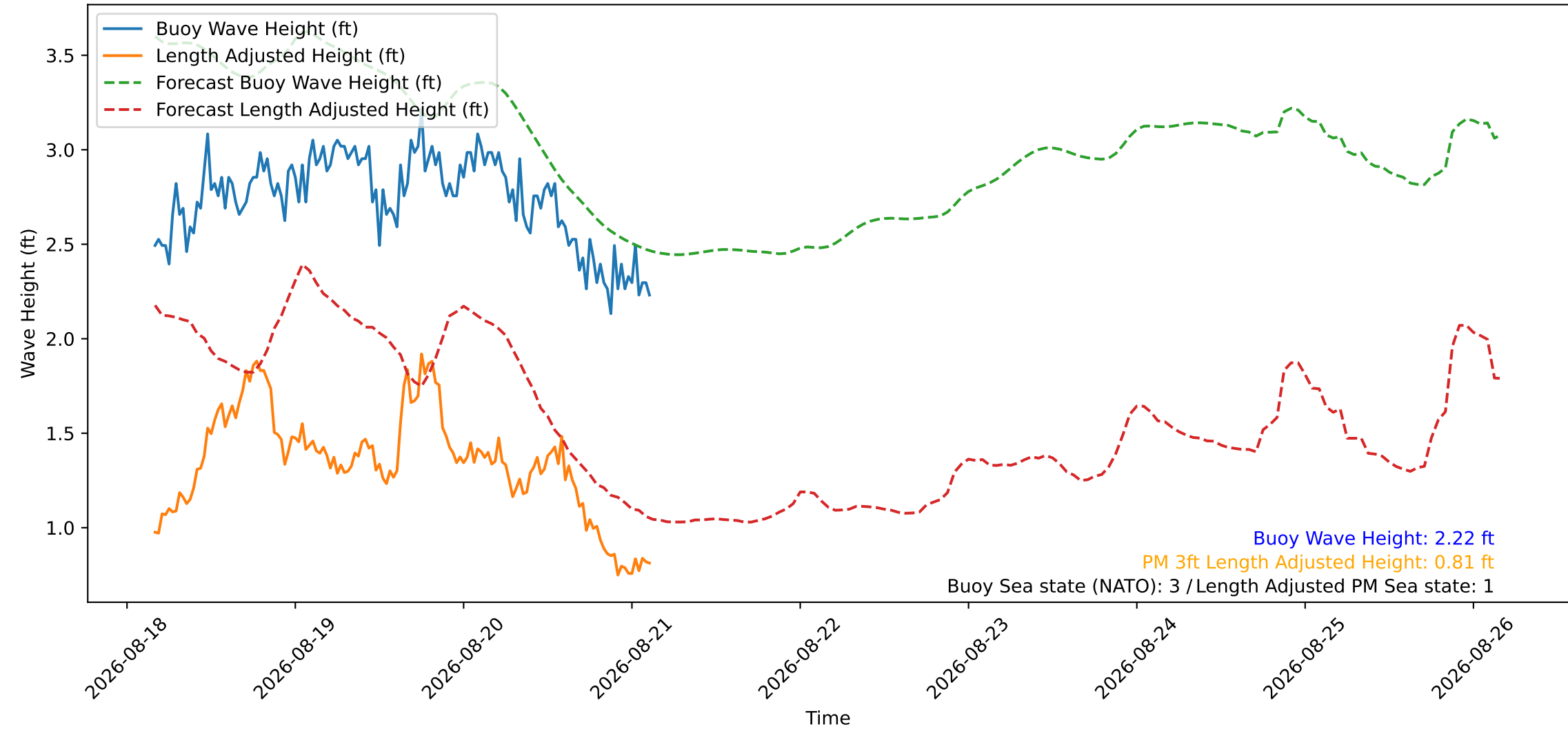
Wave Heights over Time for Red Beach at 2026-08-21 03:30:45
