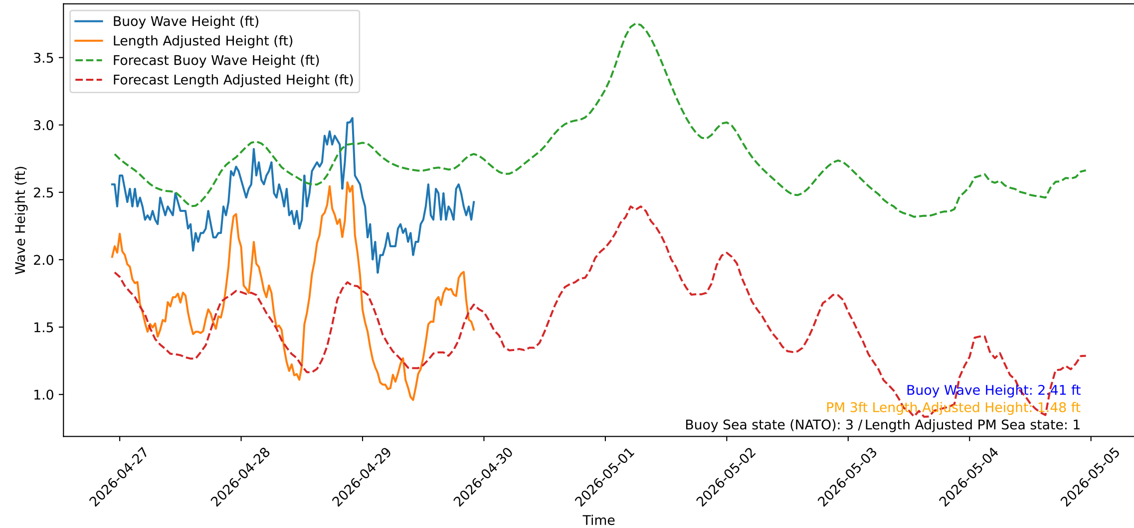
Wave Heights over Time for Oceanside Harbor at 2026-04-29 22:40:31
