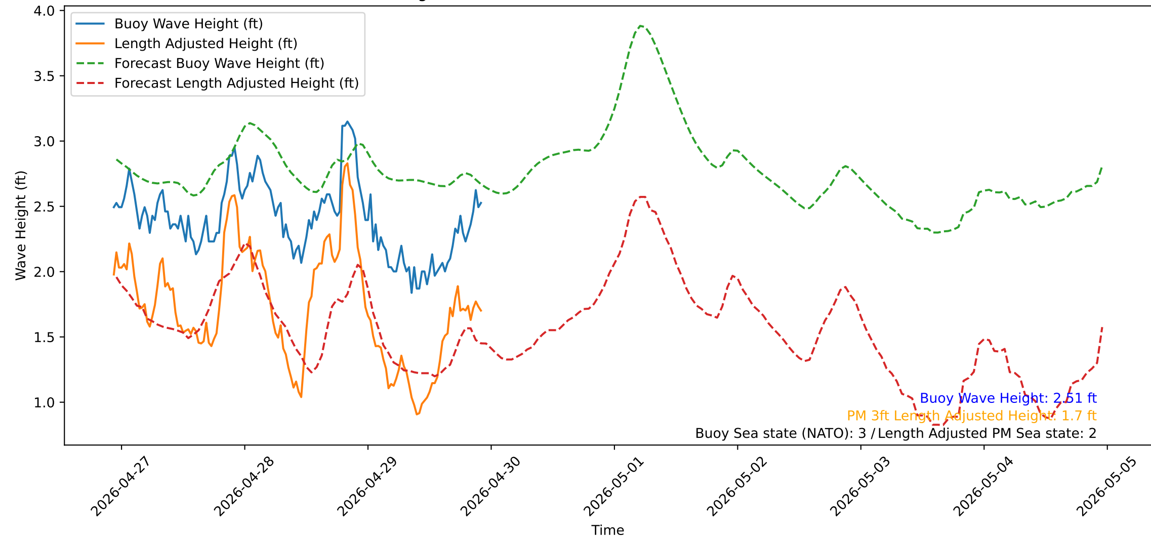
Wave Heights over Time for Green Beach at 2026-04-29 22:41:13
