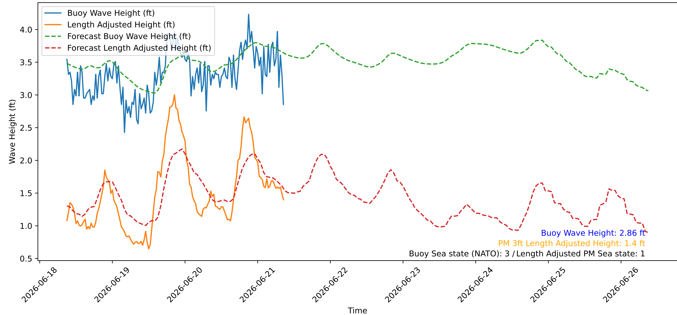
Wave Heights over Time for Green Beach at 2026-06-21 09:11:08
