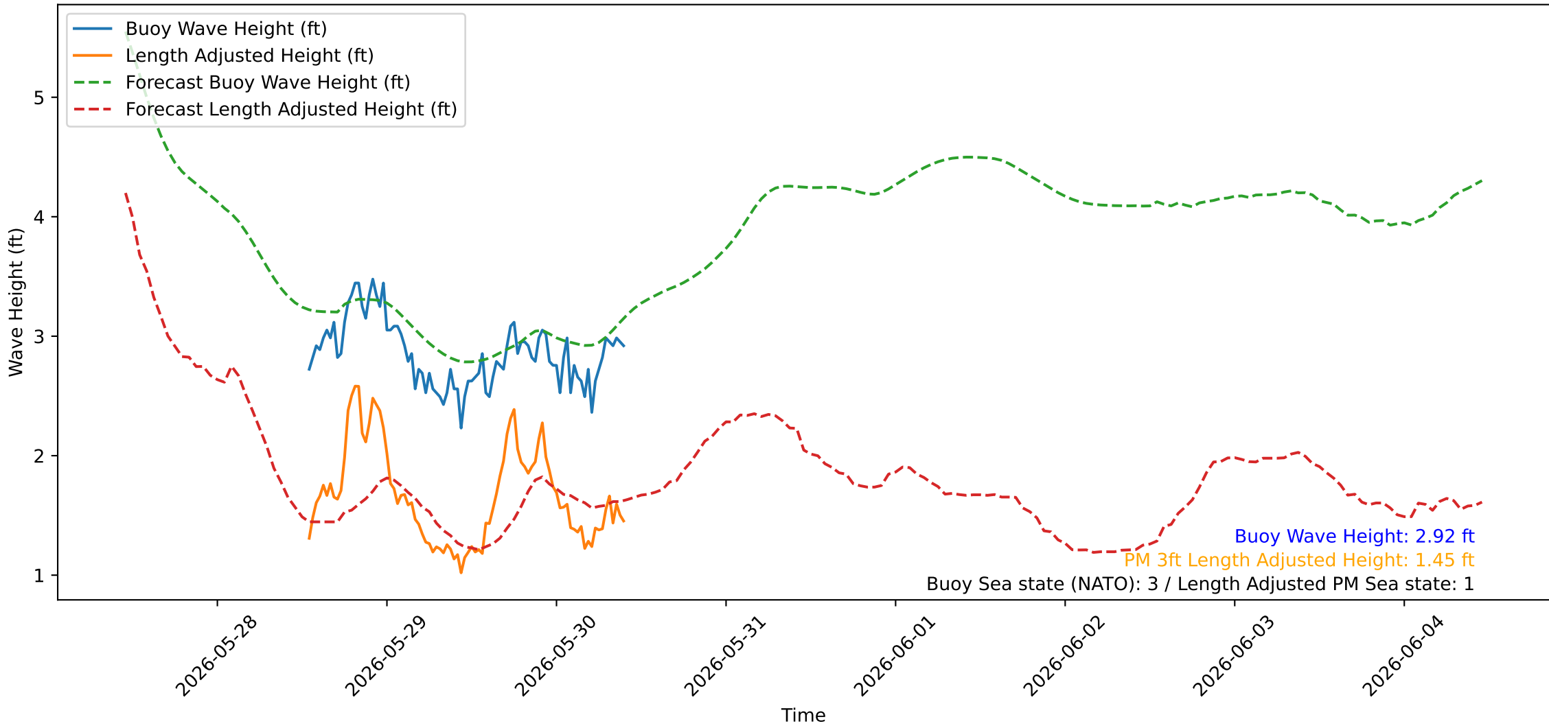
Wave Heights over Time for Oceanside Harbor at 2026-05-30 10:30:23
