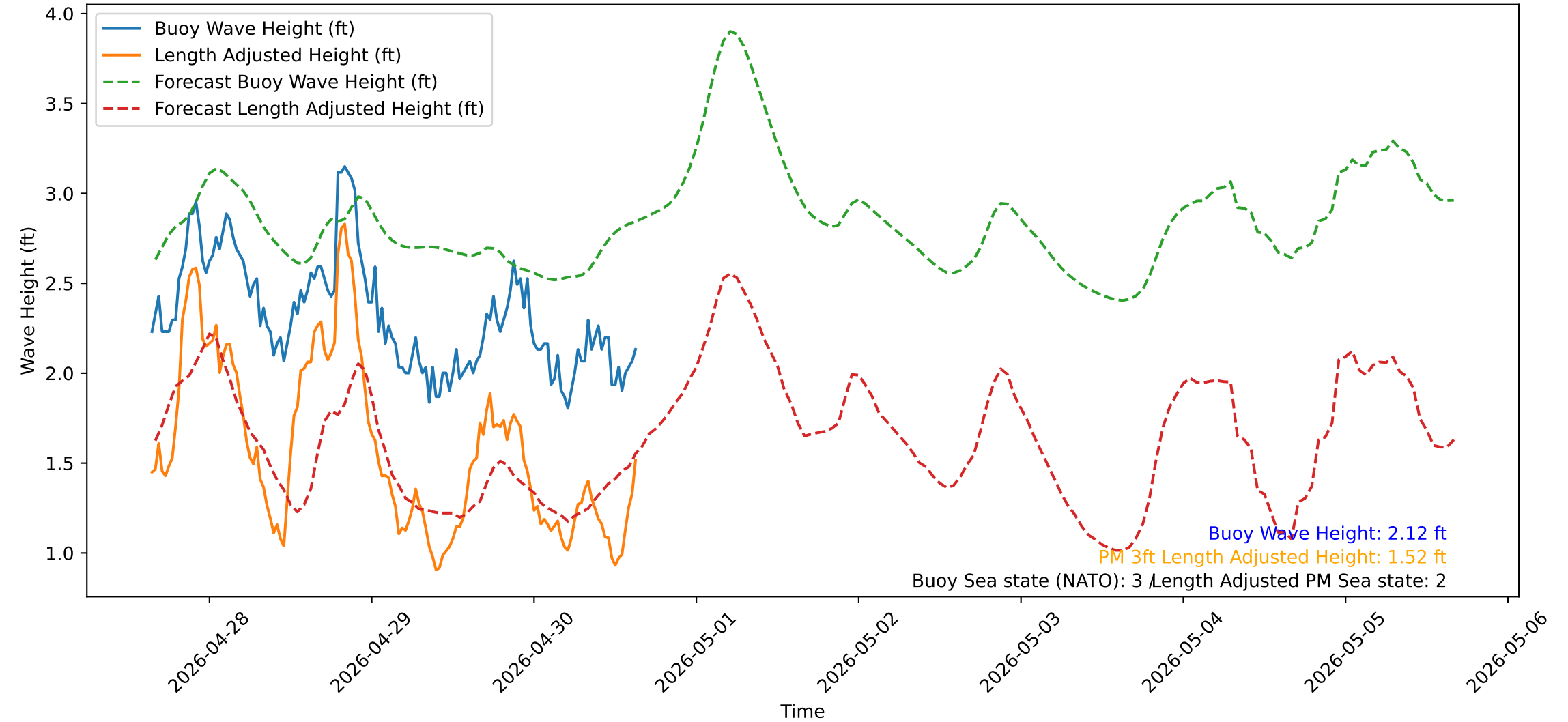
Wave Heights over Time for Green Beach at 2026-04-30 15:41:13
