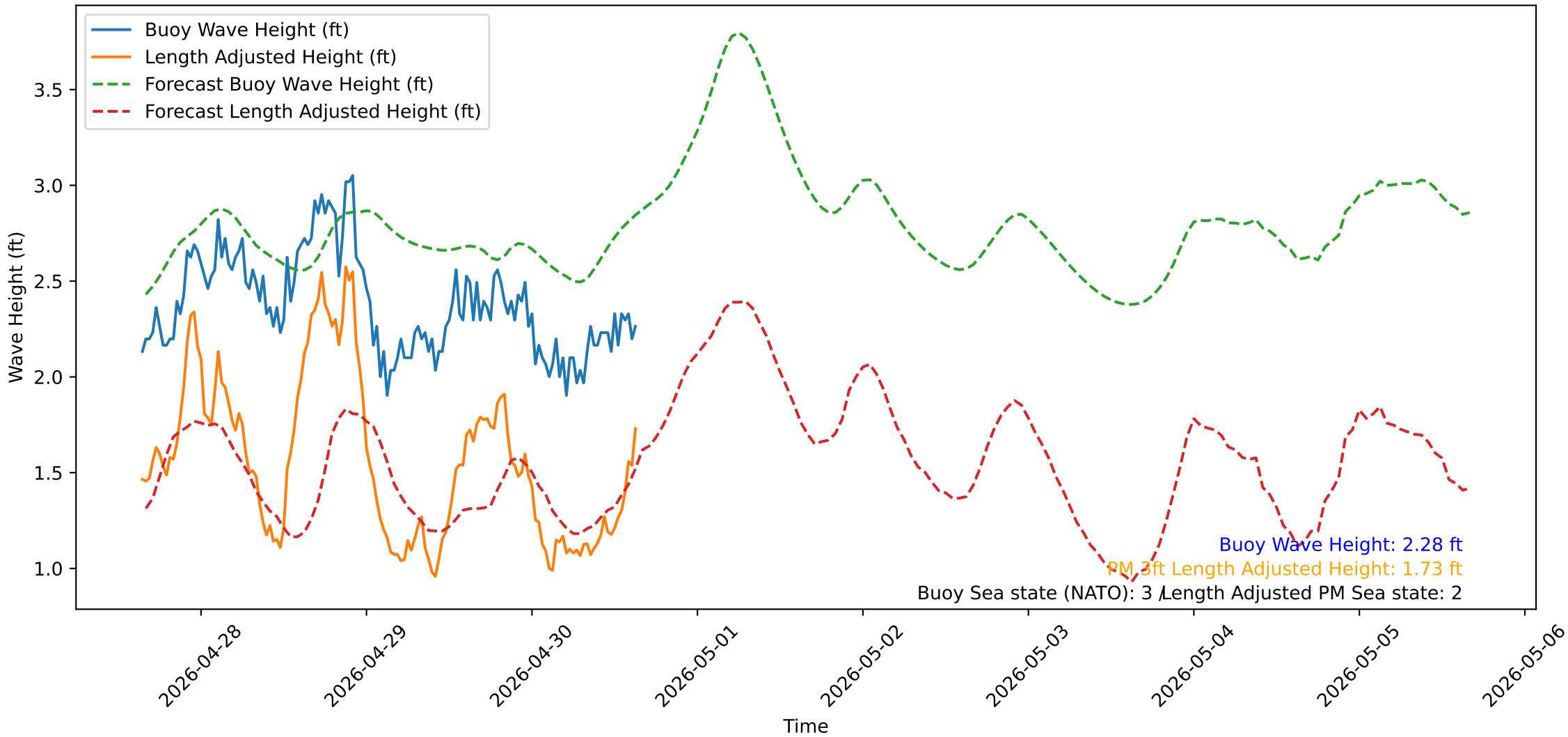
Wave Heights over Time for Oceanside Harbor at 2026-04-30 15:40:32
