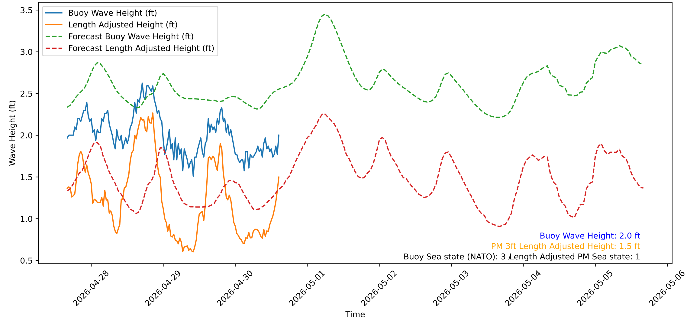
Wave Heights over Time for Red Beach at 2026-04-30 15:40:51
