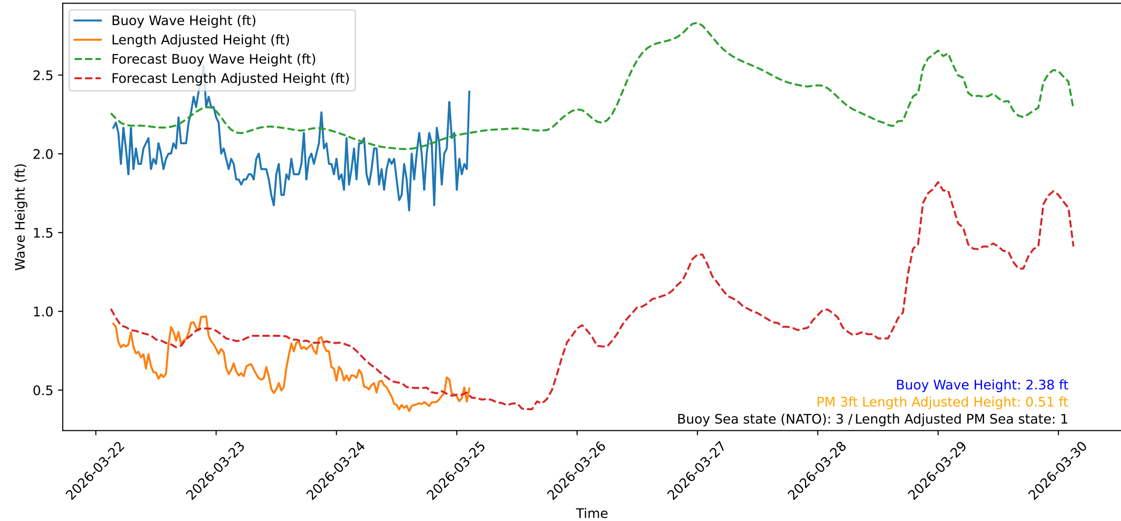
Wave Heights over Time for Red Beach at 2026-03-25 03:20:47
