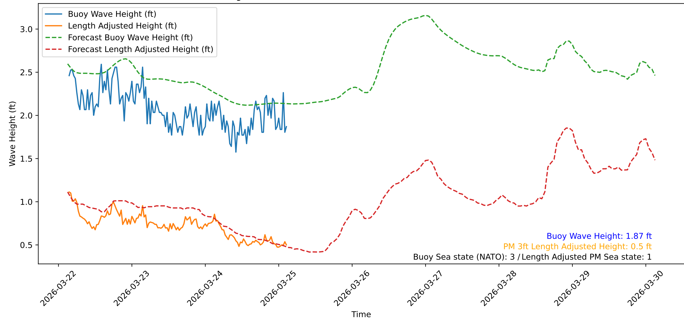
Wave Heights over Time for Oceanside Harbor at 2026-03-25 03:20:31
