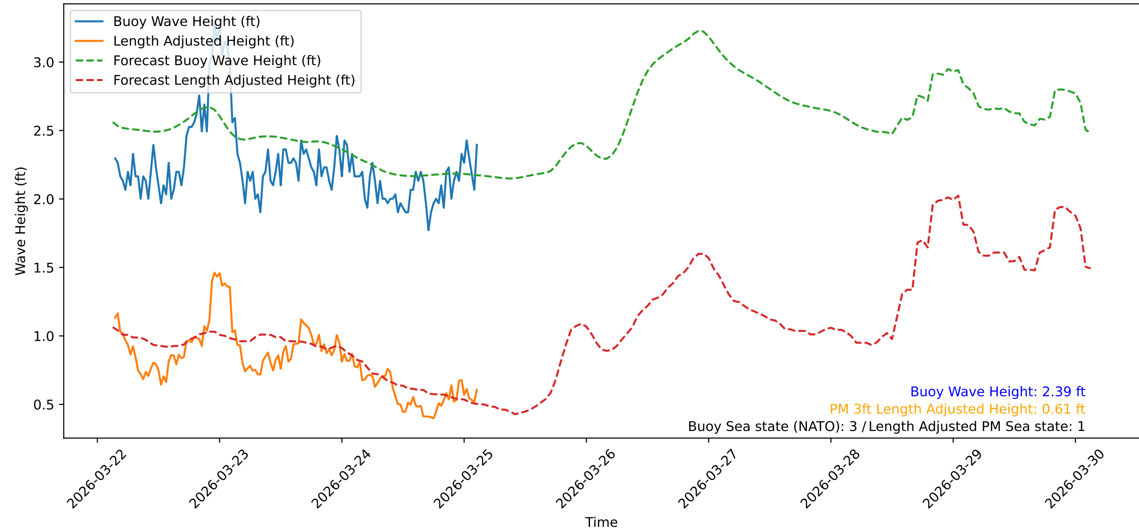
Wave Heights over Time for Green Beach at 2026-03-25 03:21:09
