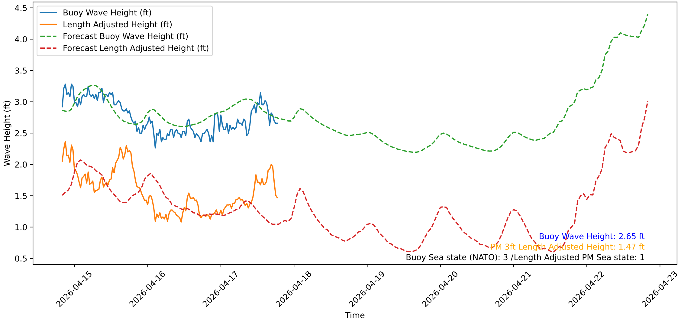
Wave Heights over Time for Red Beach at 2026-04-17 19:40:51
