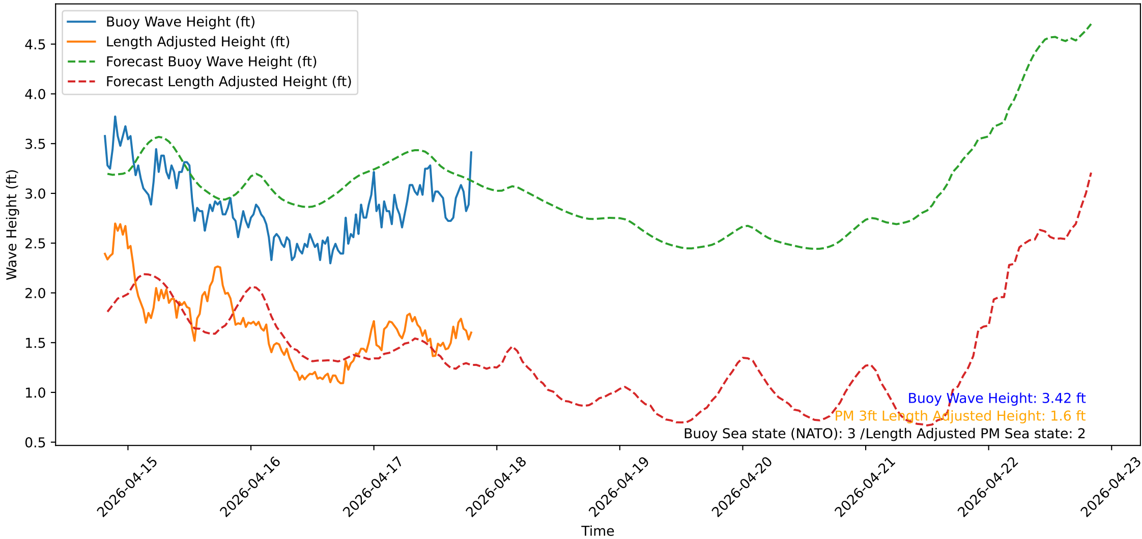
Wave Heights over Time for Oceanside Harbor at 2026-04-17 19:40:32
