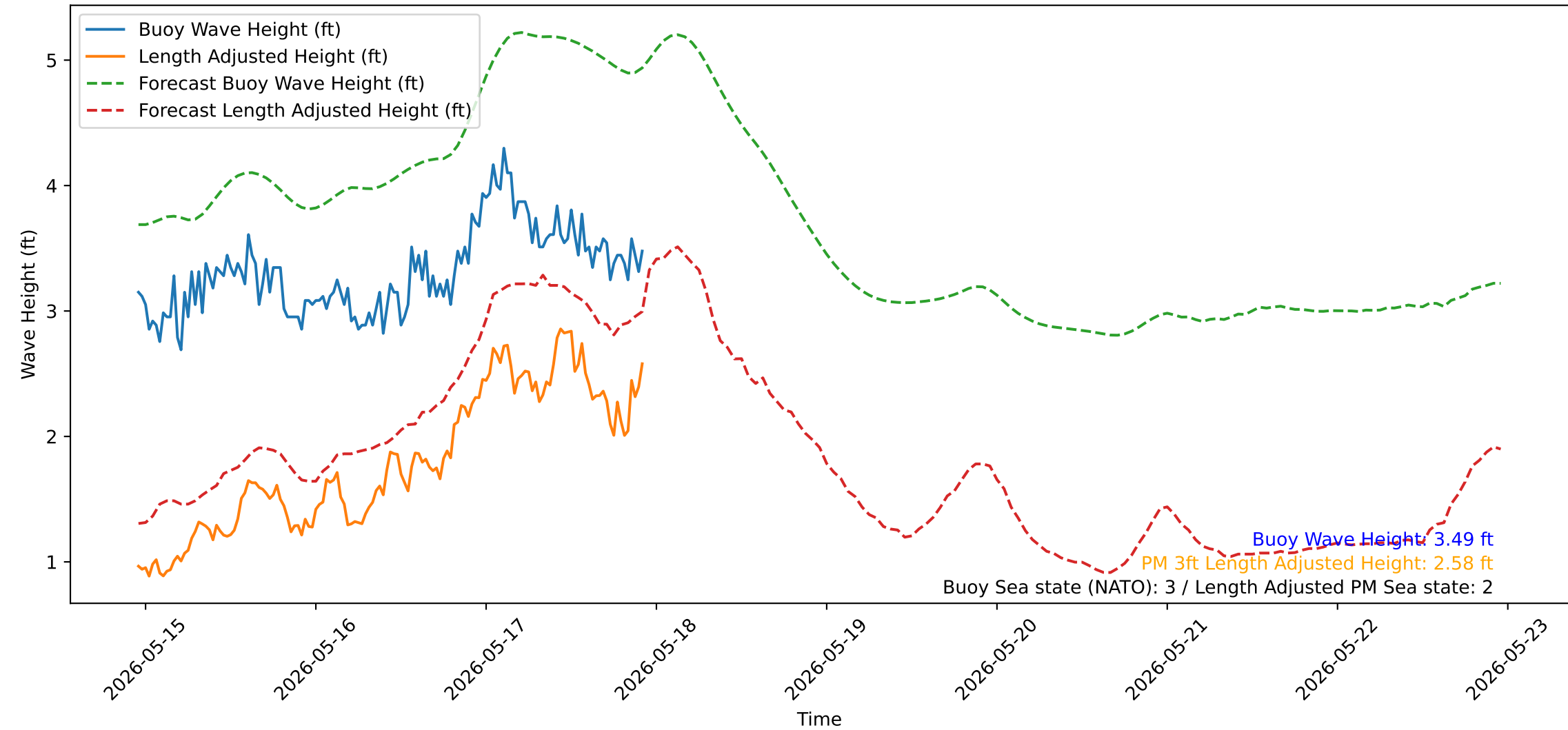
Wave Heights over Time for Oceanside Harbor at 2026-05-17 22:50:31
