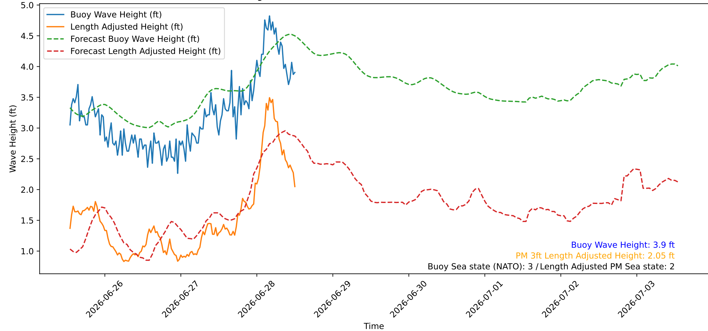
Wave Heights over Time for Green Beach at 2026-06-28 13:01:07
