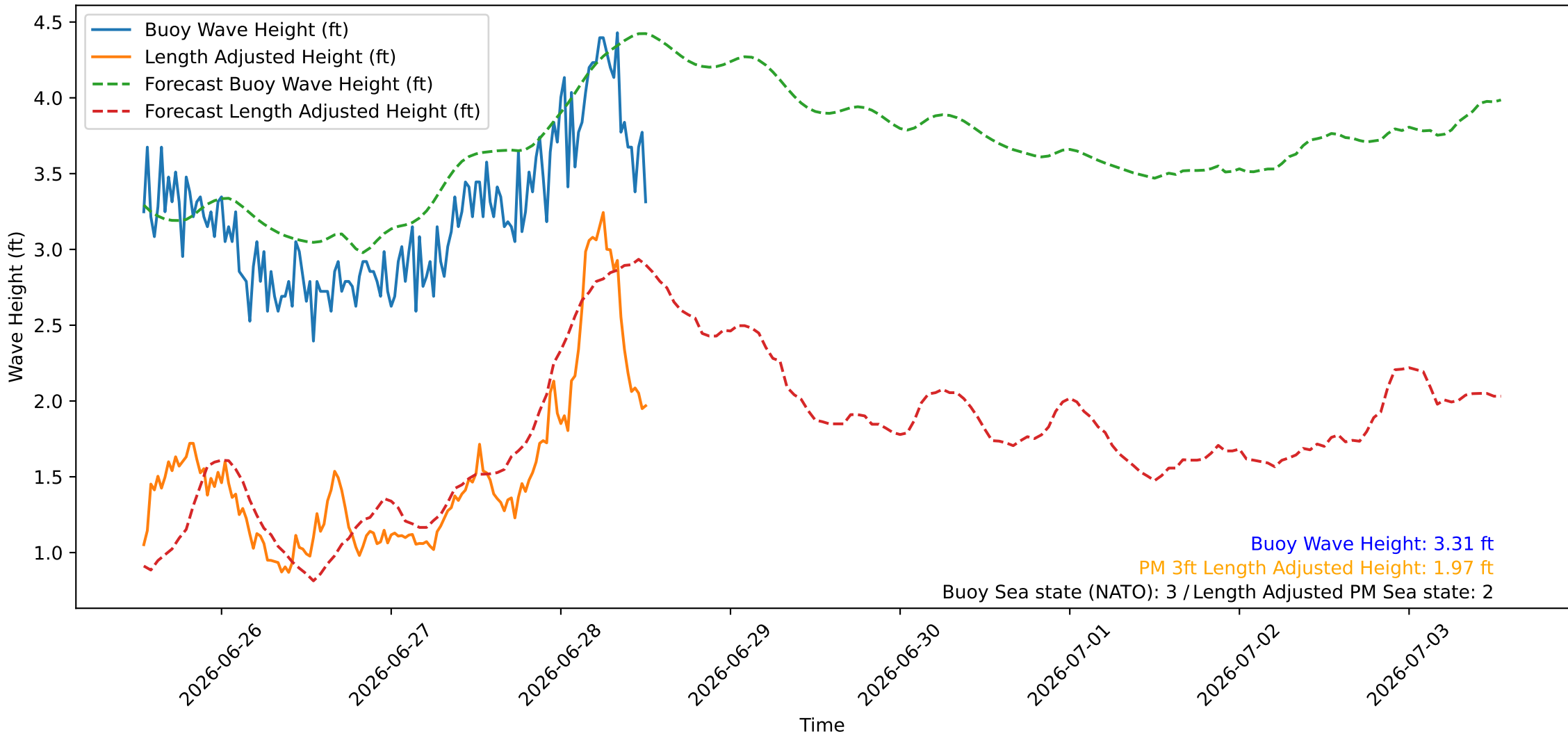
Wave Heights over Time for Oceanside Harbor at 2026-06-28 13:00:25
