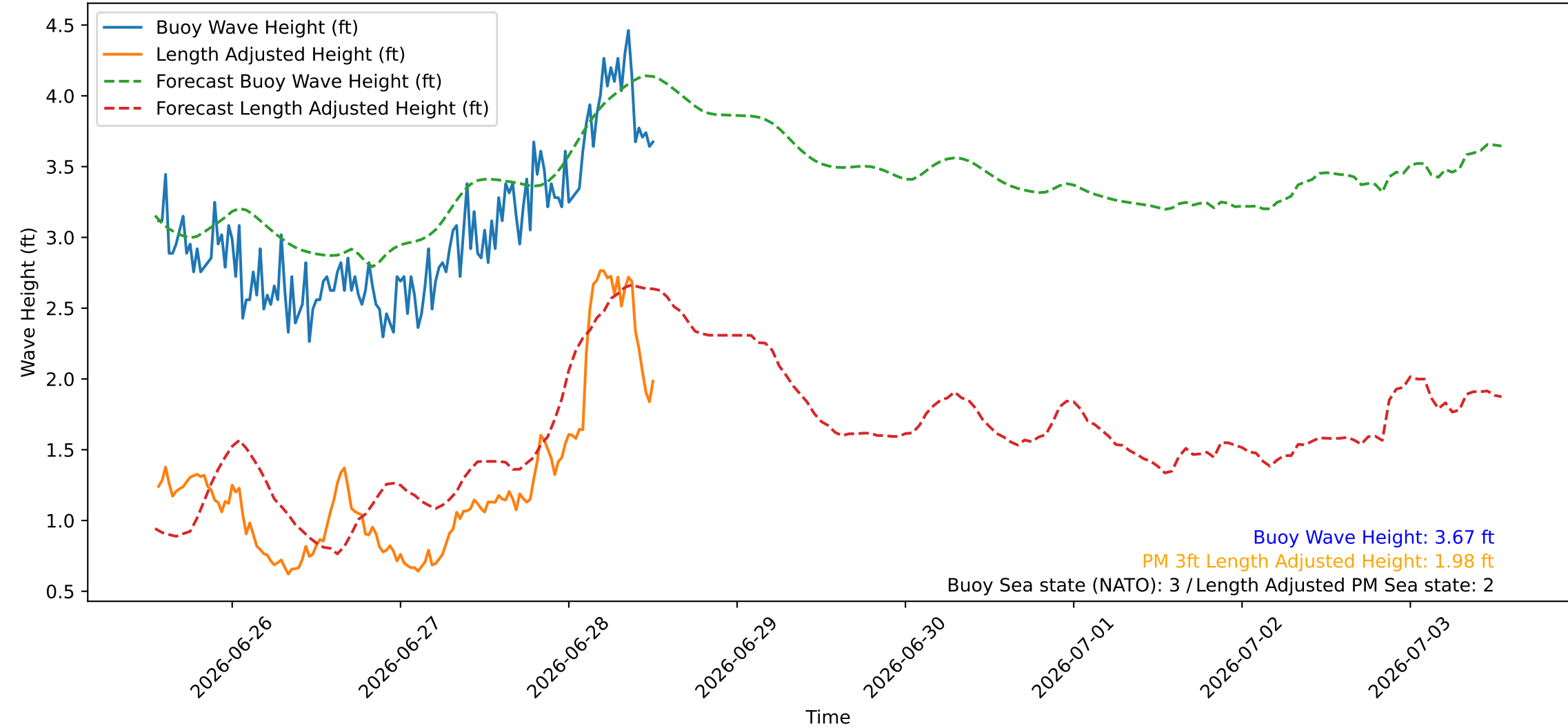
Wave Heights over Time for Red Beach at 2026-06-28 13:00:45
