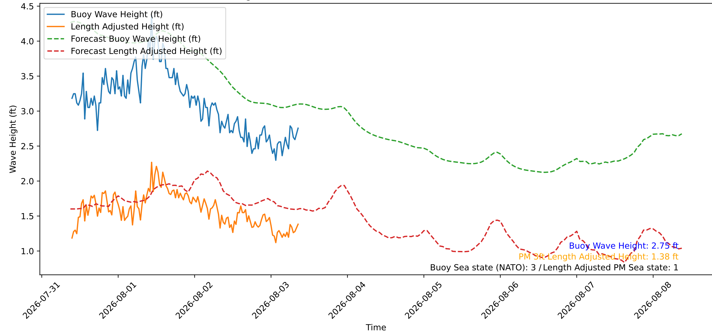
Wave Heights over Time for Oceanside Harbor at 2026-08-03 09:20:26
