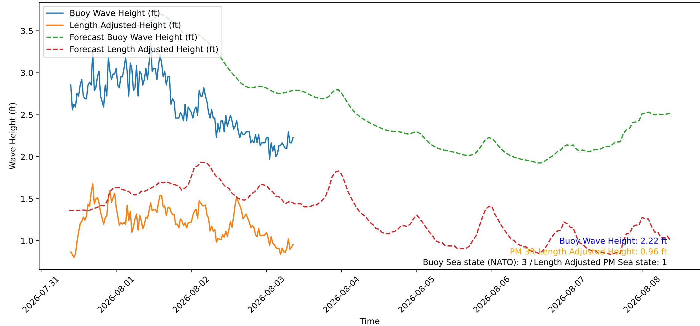
Wave Heights over Time for Red Beach at 2026-08-03 09:20:47
